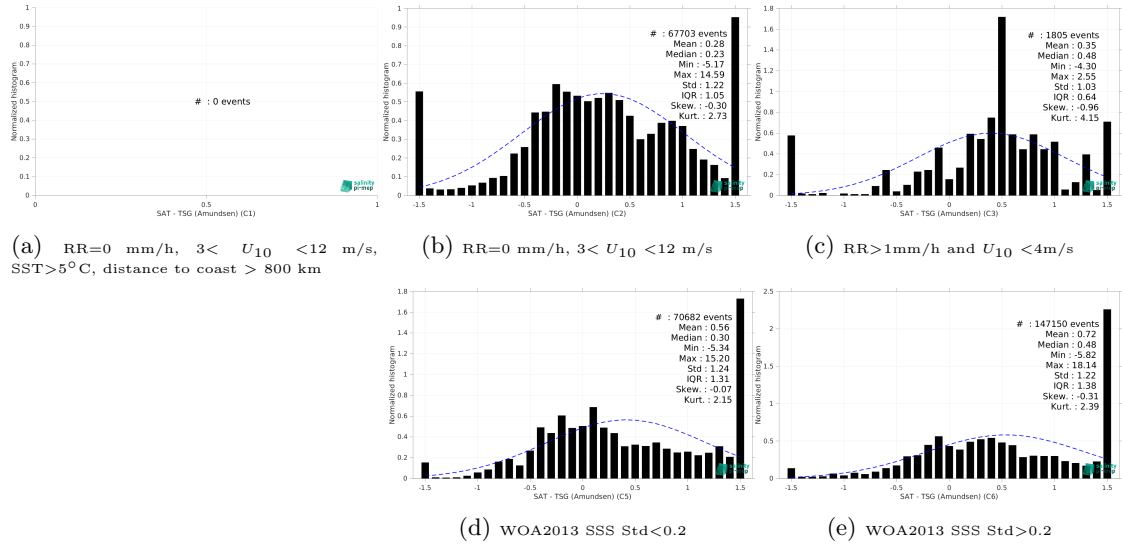
Figure 13: Normalized histogram of \Delta SSS (SMOS SSS L3 v2 - 9-Days (BEC) - TSG (Amundsen)) for 5 different subdatasets corresponding to: RR=0 mm/h, 3 < U_{10} < 12 m/s, SST > 5°C, distance to coast > 800 km (a), RR=0 mm/h, 3 < U_{10} < 12 m/s (b), RR > 1mm/h and U_{10} < 4 m/s (c), WOA2013 SSS Std < 0.2 (d), WOA2013 SSS Std > 0.2 (e).
