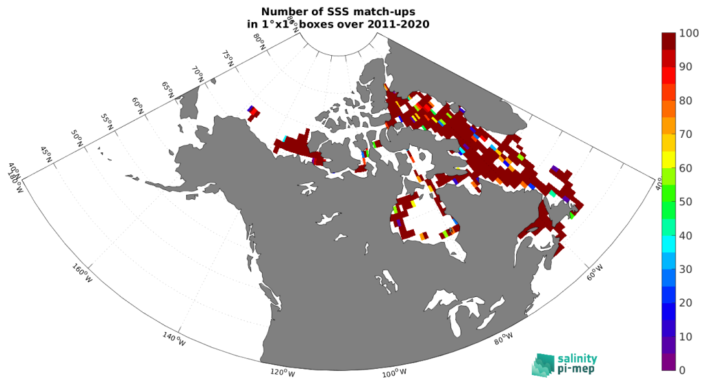
Figure 4: Number of SSS match-ups between TSG (Amundsen) SSS and the SMOS SSS L3 v2 - 9-Days (BEC) SSS product for the Global Ocean Pi-MEP region over 1^\circ \times 1^\circ boxes and for the full satellite product period.
