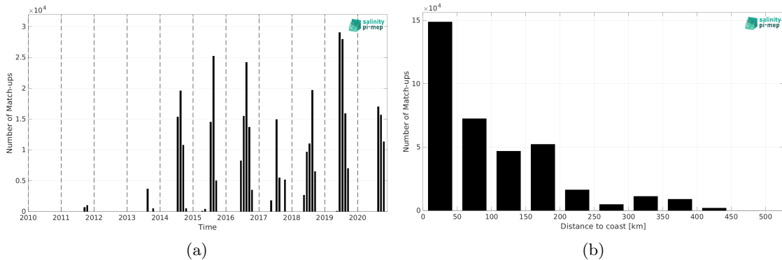
Figure 1: Number of match-ups between TSG (Amundsen) and SMOS SSS L3 v2 - 9-Days (BEC) SSS as a function of time (a) and as function of the distance to coast (b) over the Global Ocean Pi-MEP region and for the full satellite product period.
