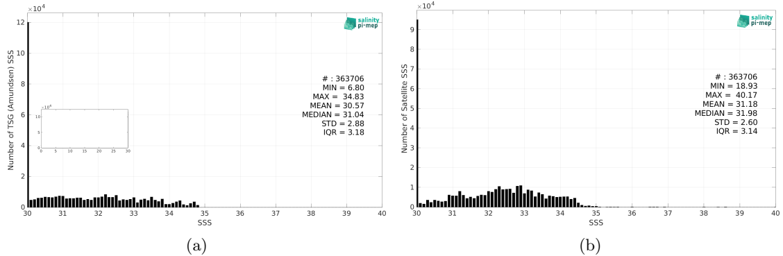
Figure 2: Histograms of SSS from TSG (Amundsen) (a) and SMOS SSS L3 v2 - 9-Days (BEC) (b) considering all match-up pairs per bins of 0.1 over the Global Ocean Pi-MEP region and for the full satellite product period.
