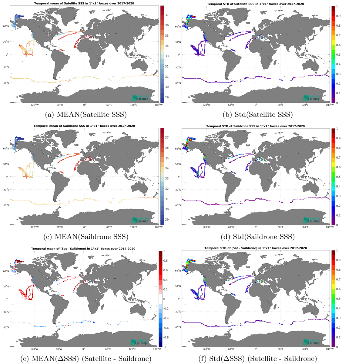
Figure 7: Temporal mean (left) and Std (right) of SSS from SMOS SSS L3 v2 - 9-Days (BEC) (top), Saildrone (middle), and of \Delta SSS (Satellite - Saildrone ). Only match-up pairs are used to generate these maps.
