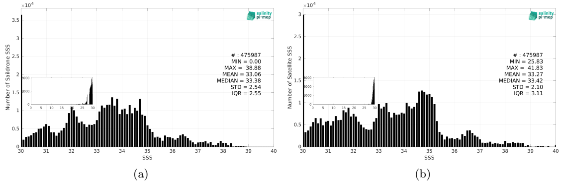
Figure 3: Histograms of SSS from Saildrone (a) and SMOS SSS L3 v2 - 9-Days (BEC) (b) considering all match-up pairs per bins of 0.1 over the Global Ocean Pi-MEP region and for the full satellite product period.
