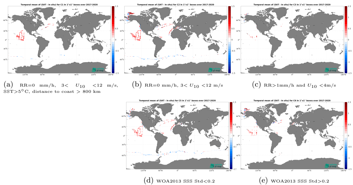
Figure 14: Temporal mean gridded over spatial boxes of size 1^\circ \times 1^\circ of \Delta SSS (SMOS SSS L3 v2 - 9-Days (BEC) - Saildrone) for 5 different subdatasets corresponding to:RR=0 mm/h, 3 < U_{10} < 12 m/s, SST > 5^\circ\text{C} , distance to coast > 800 km (a), RR=0 mm/h, 3 < U_{10} < 12 m/s (b), RR > 1 mm/h and U_{10} < 4 m/s (c), WOA2013 SSS Std < 0.2 (d), WOA2013 SSS Std > 0.2 (e).
