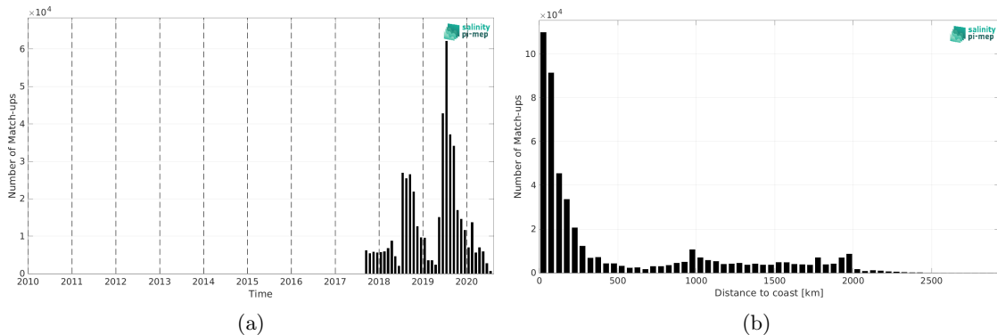
Figure 2: Number of match-ups between Saildrone and SMOS SSS L3 v2 - 9-Days (BEC) SSS as a function of time (a) and as function of the distance to coast (b) over the Global Ocean Pi-MEP region and for the full satellite product period.
