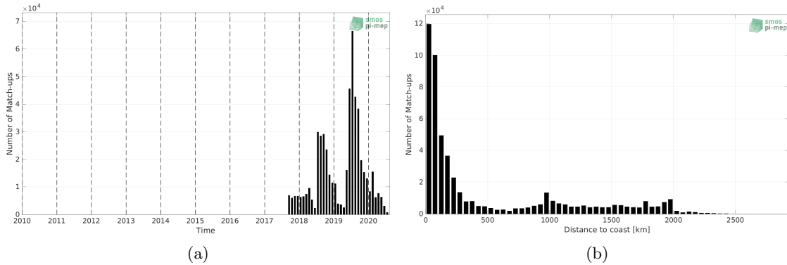
Figure 1: Number of match-ups between Saildrone and SMOS SSS L3 v2 - 9-Days (BEC) SSS as a function of time (a) and as function of the distance to coast (b) over the Global Ocean Pi-MEP region and for the full satellite product period.
