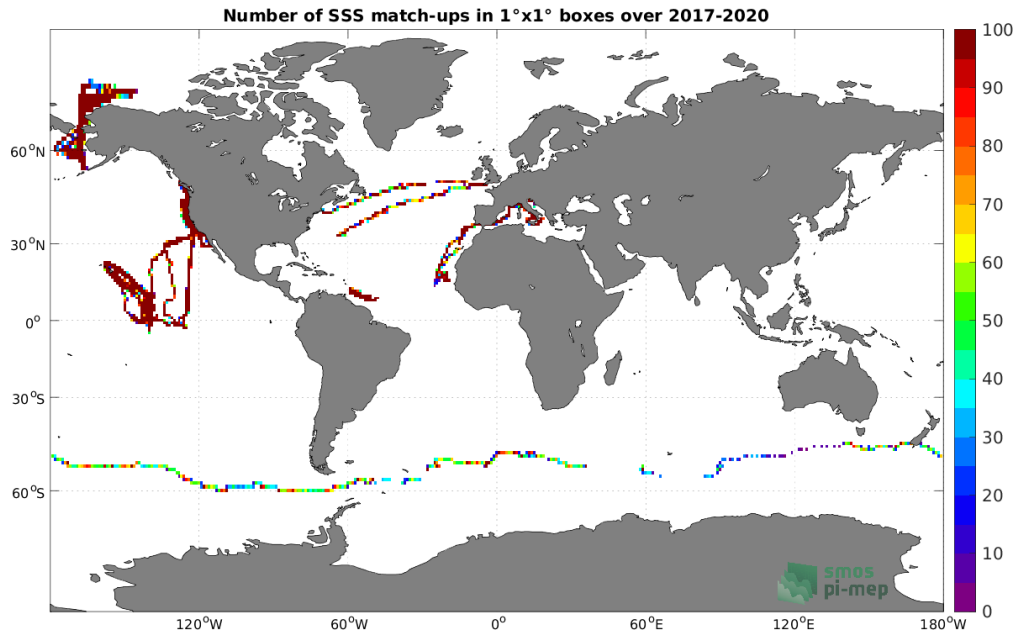
Figure 4: Number of SSS match-ups between Saildrone SSS and the SMOS SSS L3 v2 - 9-Days (BEC) SSS product for the Global Ocean Pi-MEP region over 1^\circ \times 1^\circ boxes and for the full satellite product period.
