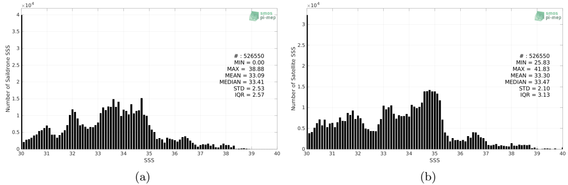
Figure 2: Histograms of SSS from Saildrone (a) and SMOS SSS L3 v2 - 9-Days (BEC) (b) considering all match-up pairs per bins of 0.1 over the Global Ocean Pi-MEP region and for the full satellite product period.
