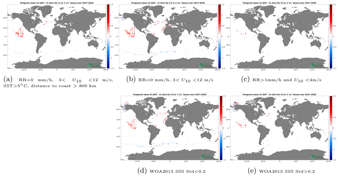
Figure 12: Temporal mean gridded over spatial boxes of size 1^\circ \times 1^\circ of \Delta SSS (SMOS SSS L3 v2 - 9-Days (BEC) - Saildrone) for 5 different subdatasets corresponding to:RR=0 mm/h, 3 < U_{10} < 12 m/s, SST > 5^\circ\text{C} , distance to coast > 800 km (a), RR=0 mm/h, 3 < U_{10} < 12 m/s (b), RR > 1 mm/h and U_{10} < 4 m/s (c), WOA2013 SSS Std < 0.2 (d), WOA2013 SSS Std > 0.2 (e).
