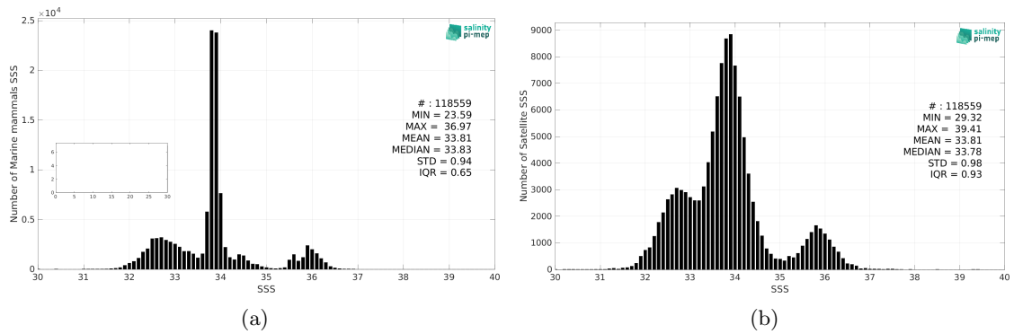
Figure 2: Histograms of SSS from Marine mammals (a) and SMOS SSS L3 v2 - 9-Days (BEC) (b) considering all match-up pairs per bins of 0.1 over the Global Ocean Pi-MEP region and for the full satellite product period.
