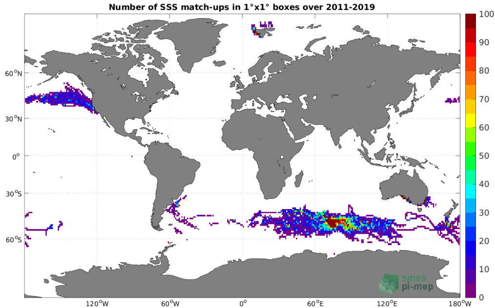
Figure 4: Number of SSS match-ups between Marine mammals SSS and the SMOS SSS L3 v2 - 9-Days (BEC) SSS product for the Global Ocean Pi-MEP region over 1°×1° boxes and for the full satellite product period.
