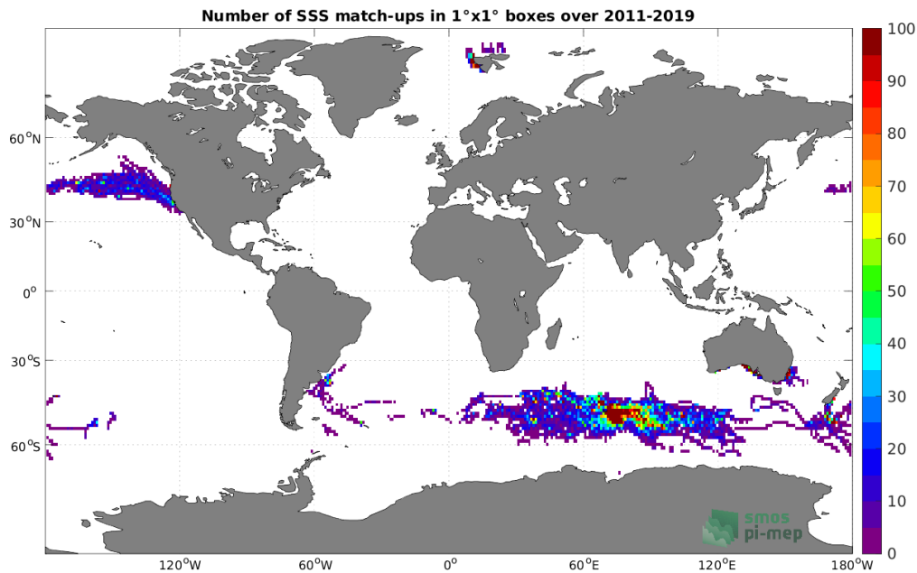
Figure 4: Number of SSS match-ups between Marine mammals SSS and the SMOS SSS L3 v2 - 9-Days (BEC) SSS product for the Global Ocean Pi-MEP region over 1^{\circ} \times 1^{\circ} boxes and for the full satellite product period.
