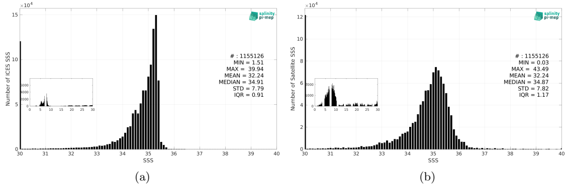
Figure 3: Histograms of SSS from ICES (a) and SMOS SSS L3 v2 - 9-Days (BEC) (b) considering all match-up pairs per bins of 0.1 over the Global Ocean Pi-MEP region and for the full satellite product period.
