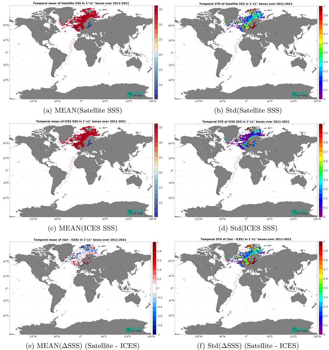
Figure 7: Temporal mean (left) and Std (right) of SSS from SMOS SSS L3 v2 - 9-Days (BEC) (top), ICES (middle), and of \Delta SSS (Satellite - ICES). Only match-up pairs are used to generate these maps.
