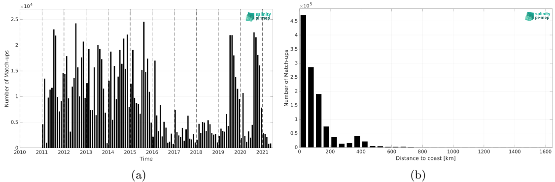
Figure 2: Number of match-ups between ICES and SMOS SSS L3 v2 - 9-Days (BEC) SSS as a function of time (a) and as function of the distance to coast (b) over the Global Ocean Pi-MEP region and for the full satellite product period.
