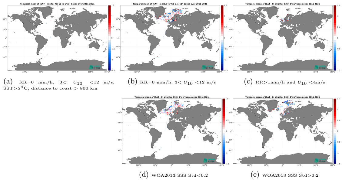
Figure 14: Temporal mean gridded over spatial boxes of size 1^\circ \times 1^\circ of \Delta SSS (SMOS SSS L3 v2 - 9-Days (BEC) - ICES) for 5 different subdatasets corresponding to:RR=0 mm/h, 3 < U_{10} < 12 m/s, SST > 5°C, distance to coast > 800 km (a), RR=0 mm/h, 3 < U_{10} < 12 m/s (b), RR > 1mm/h and U_{10} < 4 m/s (c), WOA2013 SSS Std < 0.2 (d), WOA2013 SSS Std > 0.2 (e).
