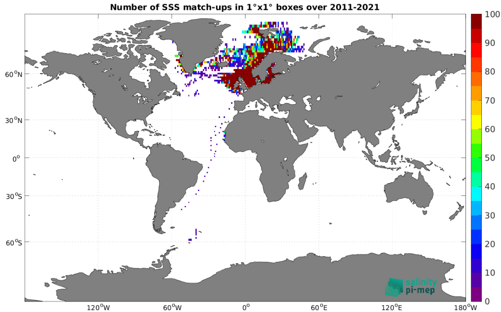
Figure 5: Number of SSS match-ups between ICES SSS and the SMOS SSS L3 v2 - 9-Days (BEC) SSS product for the Global Ocean Pi-MEP region over 1^\circ \times 1^\circ boxes and for the full satellite product period.
