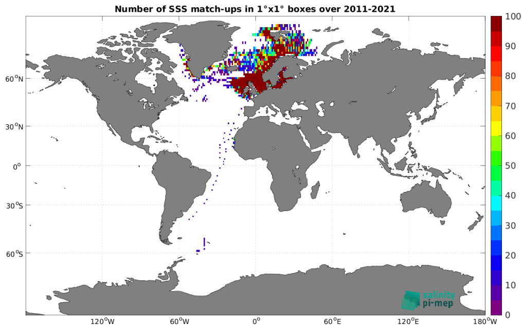
Figure 4: Number of SSS match-ups between ICES SSS and the SMOS SSS L3 v2 - 9-Days (BEC) SSS product for the Global Ocean Pi-MEP region over 1^\circ \times 1^\circ boxes and for the full satellite product period.
