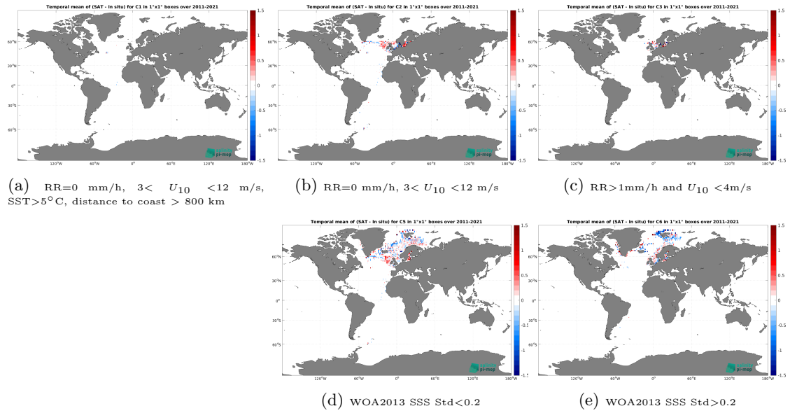
Figure 12: Temporal mean gridded over spatial boxes of size 1^\circ \times 1^\circ of \Delta SSS (SMOS SSS L3 v2 - 9-Days (BEC) - ICES) for 5 different subdatasets corresponding to:RR=0 mm/h, 3 < U_{10} < 12 m/s, SST >5^\circ\text{C} , distance to coast > 800 km (a), RR=0 mm/h, 3 < U_{10} < 12 m/s (b), RR >1 mm/h and U_{10} < 4 m/s (c), WOA2013 SSS Std <0.2 (d), WOA2013 SSS Std >0.2 (e).
