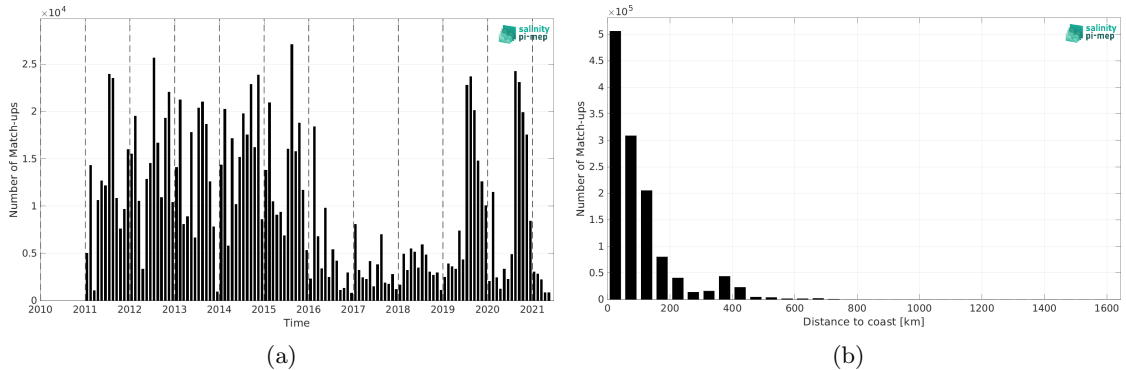
Figure 1: Number of match-ups between ICES and SMOS SSS L3 v2 - 9-Days (BEC) SSS as a function of time (a) and as function of the distance to coast (b) over the Global Ocean Pi-MEP region and for the full satellite product period.
