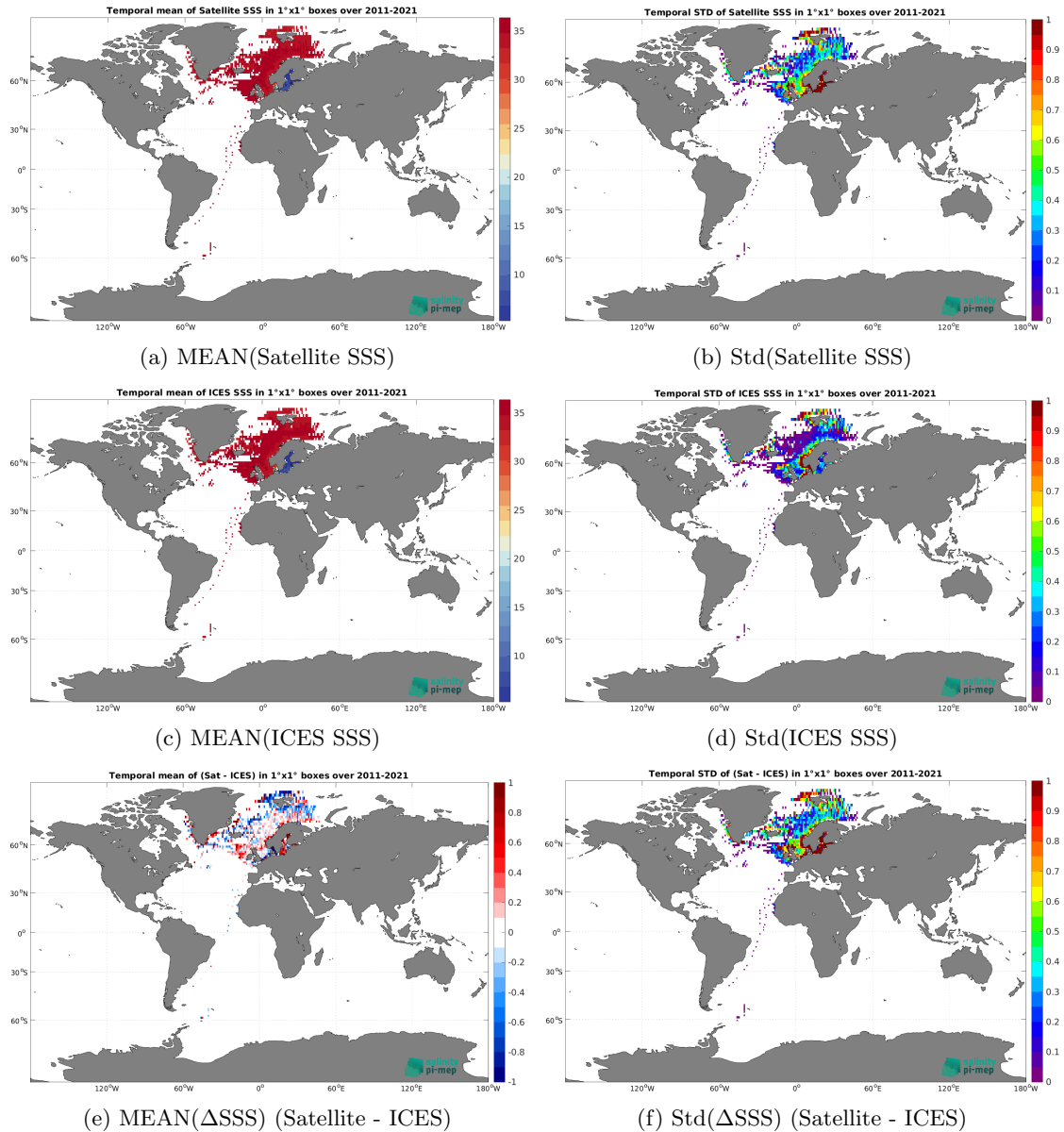
Figure 6: Temporal mean (left) and Std (right) of SSS from SMOS SSS L3 v2 - 9-Days (BEC) (top), ICES (middle), and of \Delta SSS (Satellite - ICES). Only match-up pairs are used to generate these maps.
