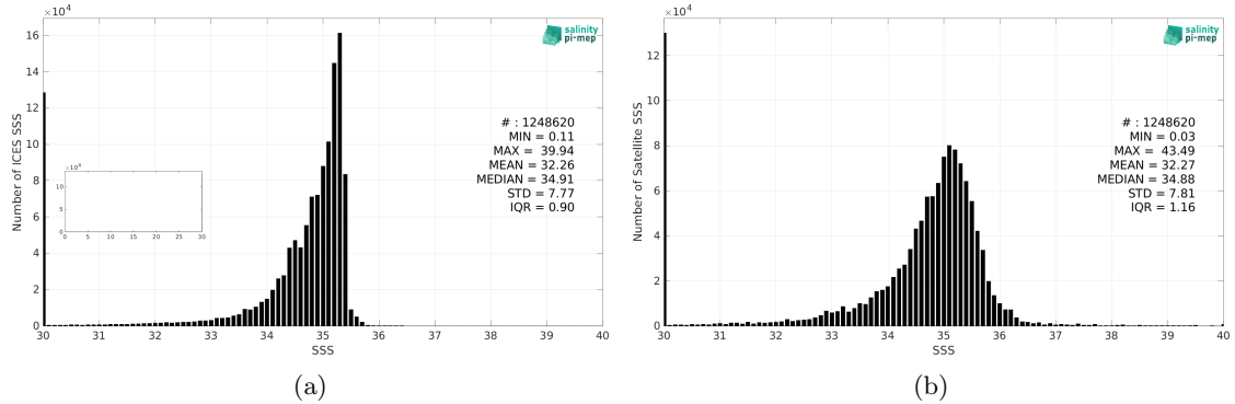
Figure 2: Histograms of SSS from ICES (a) and SMOS SSS L3 v2 - 9-Days (BEC) (b) considering all match-up pairs per bins of 0.1 over the Global Ocean Pi-MEP region and for the full satellite product period.
