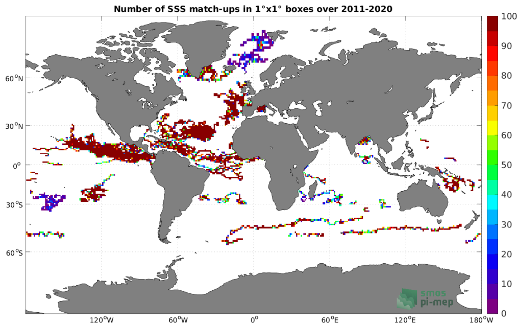
Figure 3: Number of SSS match-ups between Surface drifters SSS and the SMOS SSS L3 v2 - 9-Days (BEC) SSS product for the Global Ocean Pi-MEP region over 1^\circ \times 1^\circ boxes and for the full satellite product period.
