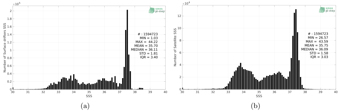
Figure 2: Histograms of SSS from Surface drifters (a) and SMOS SSS L3 v2 - 9-Days (BEC) (b) considering all match-up pairs per bins of 0.1 over the Global Ocean Pi-MEP region and for the full satellite product period.
