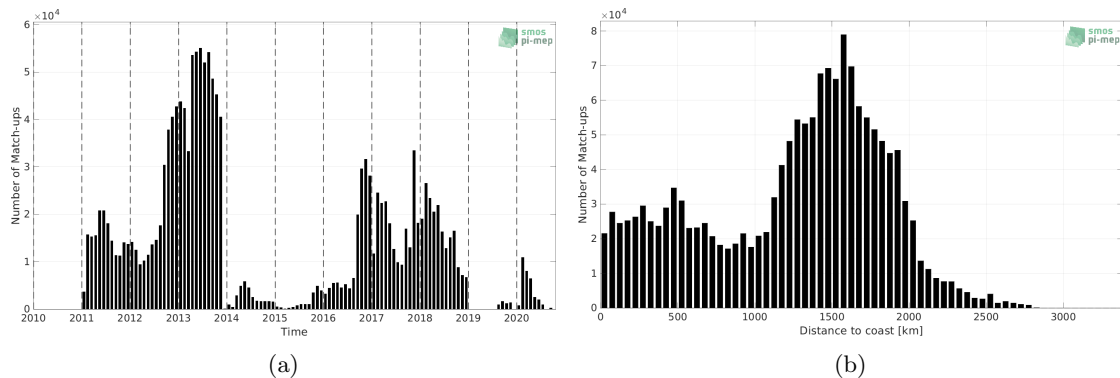
Figure 1: Number of match-ups between Surface drifters and SMOS SSS L3 v2 - 9-Days (BEC) SSS as a function of time (a) and as function of the distance to coast (b) over the Global Ocean Pi-MEP region and for the full satellite product period.
