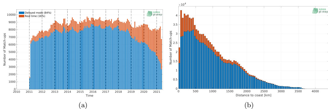
Figure 1: Number of match-ups between Argo and SMOS SSS L3 v2 - 9-Days (BEC) SSS as a function of time (a) and as function of the distance to coast (b) over the Global Ocean Pi-MEP region and for the full satellite product period.
