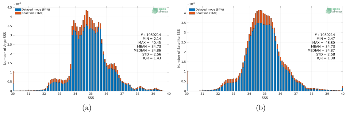
Figure 2: Histograms of SSS from Argo (a) and SMOS SSS L3 v2 - 9-Days (BEC) (b) considering all match-up pairs per bins of 0.1 over the Global Ocean Pi-MEP region and for the full satellite product period.
