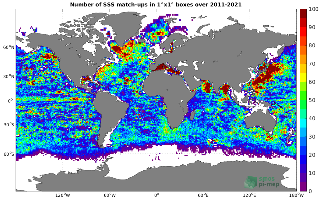
Figure 4: Number of SSS match-ups between Argo SSS and the SMOS SSS L3 v2 - 9-Days (BEC) SSS product for the Global Ocean Pi-MEP region over 1^\circ \times 1^\circ boxes and for the full satellite product period.
