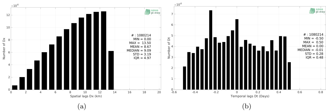
Figure 5: Histograms of the spatial (a) and temporal (b) lags between the location/time of the Argo measurement and the date of the corresponding SMOS SSS L3 v2 - 9-Days (BEC) SSS pixel.
