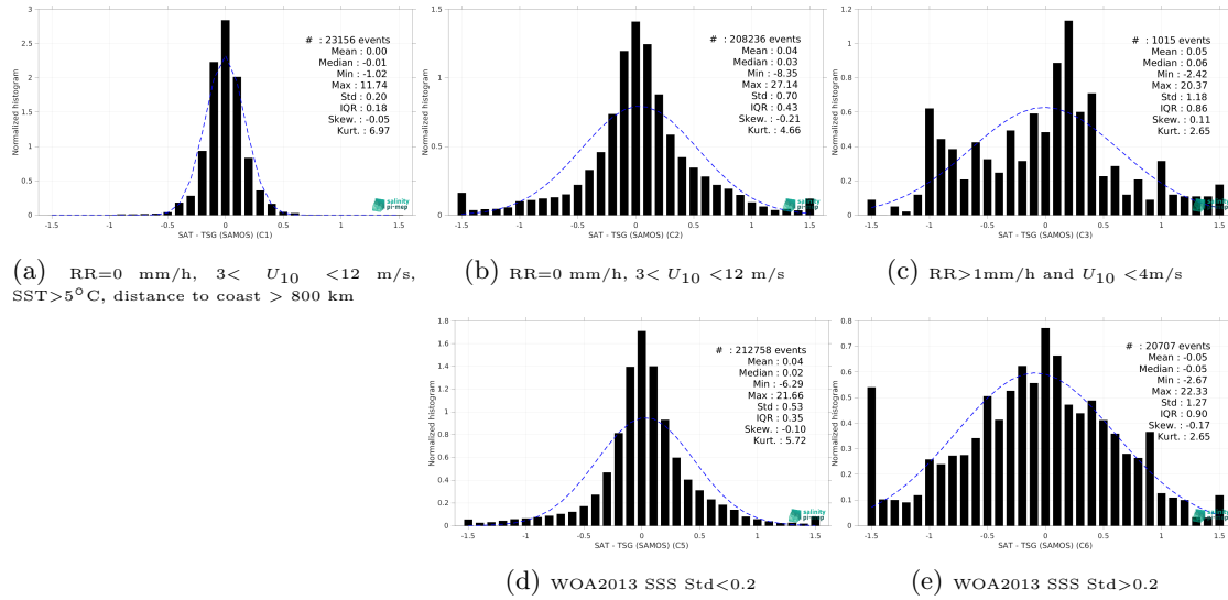
Figure 15: Normalized histogram of \Delta SSS (SMOS SSS L3 Southern Ocean v1 - 9-Day running mean (BEC) - TSG (SAMOS)) for 5 different subdatasets corresponding to: RR=0 mm/h, 3 < U_{10} < 12 m/s, SST>5°C, distance to coast > 800 km (a), RR=0 mm/h, 3 < U_{10} < 12 m/s (b), RR>1mm/h and U_{10} < 4 m/s (c), WOA2013 SSS Std<0.2 (d), WOA2013 SSS Std>0.2 (e).
