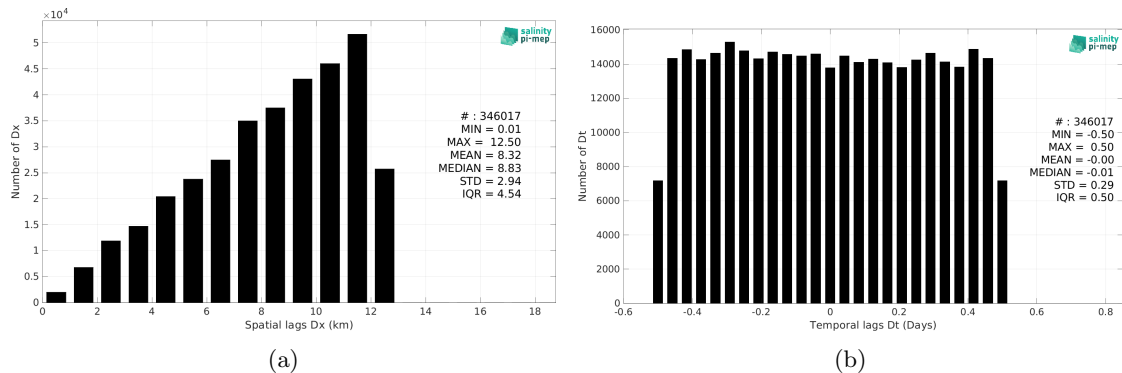
Figure 6: Histograms of the spatial (a) and temporal (b) lags between the location/time of the TSG (SAMOS) measurement and the date of the corresponding SMOS SSS L3 Southern Ocean v1 - 9-Day running mean (BEC) SSS pixel.
