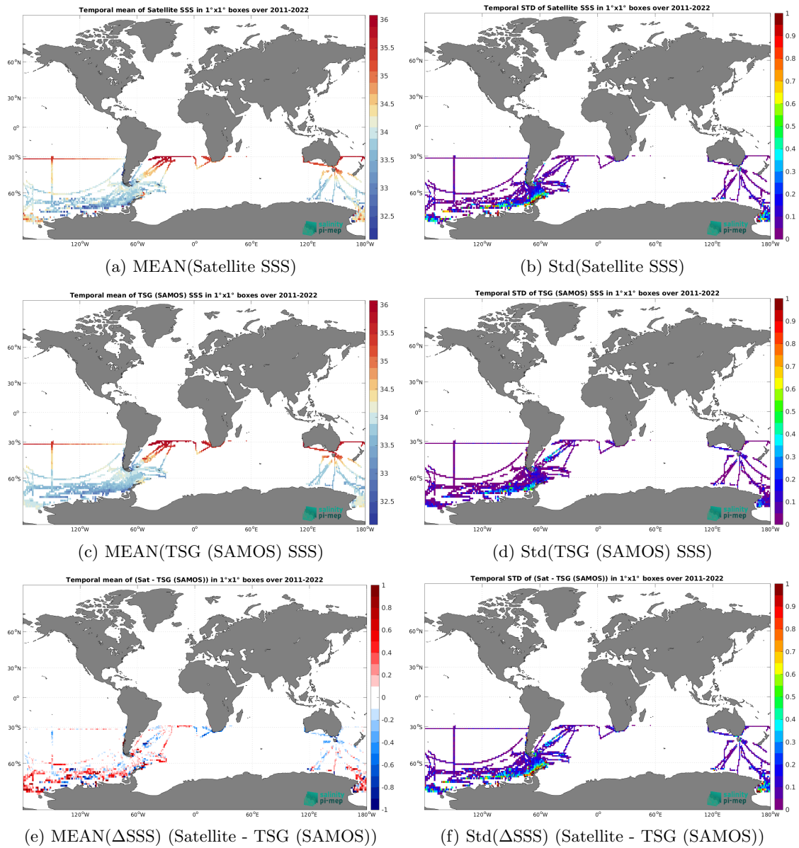
Figure 7: Temporal mean (left) and Std (right) of SSS from SMOS SSS L3 Southern Ocean v1 - 9-Day running mean (BEC) (top), TSG (SAMOS) (middle), and of \Delta SSS (Satellite - TSG (SAMOS)). Only match-up pairs are used to generate these maps.
