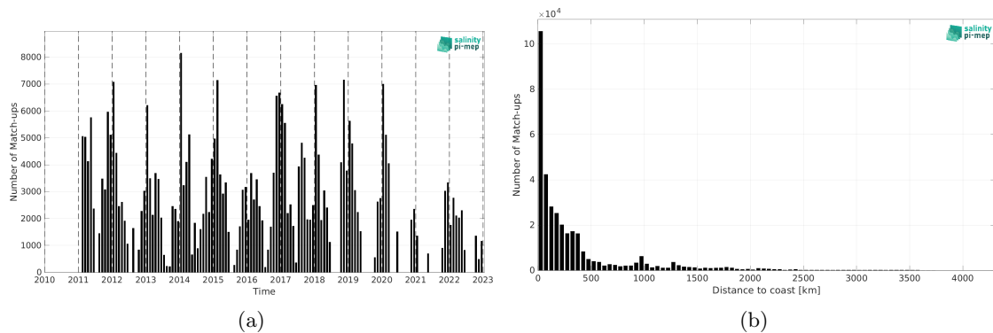
Figure 2: Number of match-ups between TSG (SAMOS) and SMOS SSS L3 Southern Ocean v1 - 9-Day running mean (BEC) SSS as a function of time (a) and as function of the distance to coast (b) over the Global Ocean Pi-MEP region and for the full satellite product period.
