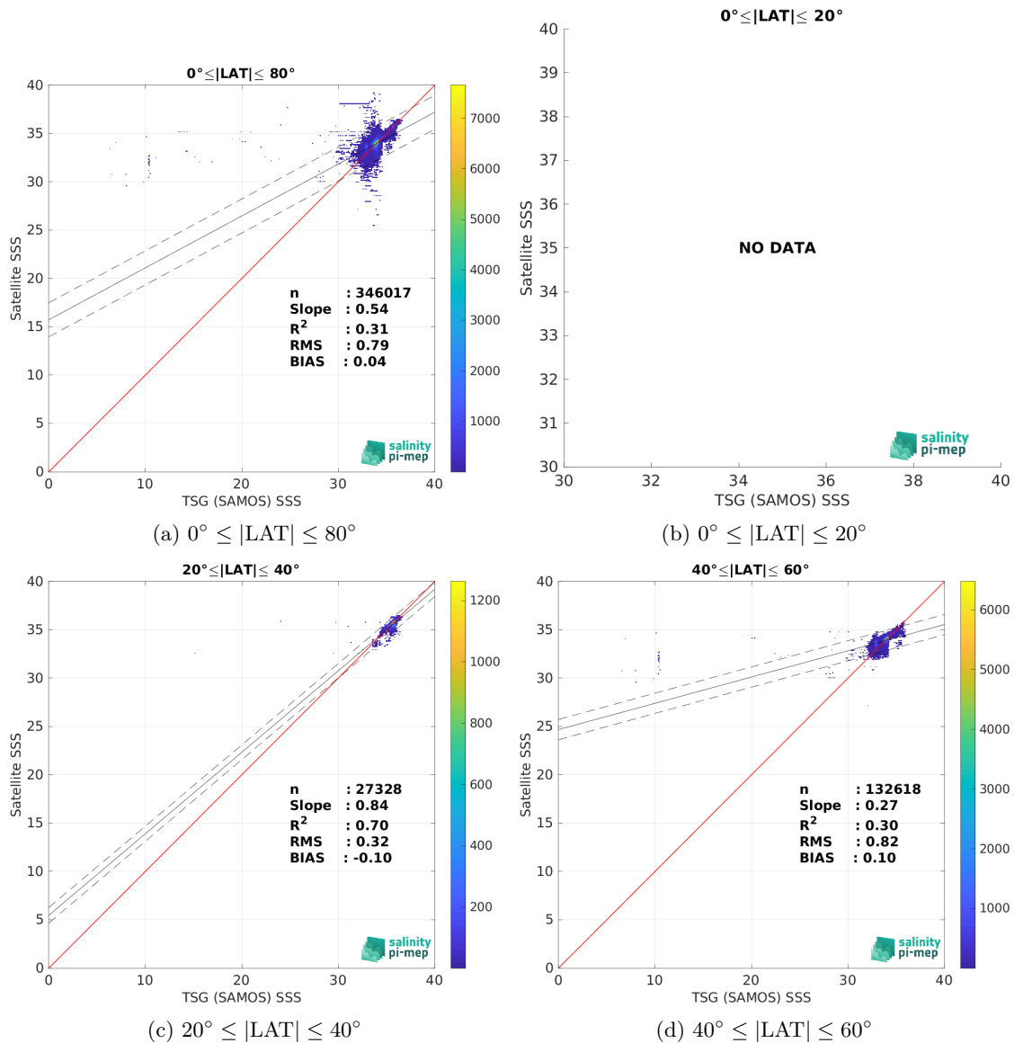
Figure 10: Contour maps of the concentration of SMOS SSS L3 Southern Ocean v1 - 9-Day running mean (BEC) SSS (y-axis) versus TSG (SAMOS) SSS (x-axis) at match-up pairs for different latitude bands. For each plot, the red line shows x=y . The black thin and dashed lines indicate a linear fit through the data cloud and the \pm 95\% confidence levels, respectively. The number match-up pairs n , the slope and R^2 coefficient of the linear fit, the root mean square (RMS) and the mean bias between satellite and in situ data are indicated for each latitude band in each plots.
