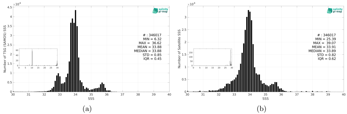
Figure 3: Histograms of SSS from TSG (SAMOS) (a) and SMOS SSS L3 Southern Ocean v1 - 9-Day running mean (BEC) (b) considering all match-up pairs per bins of 0.1 over the Global Ocean Pi-MEP region and for the full satellite product period.
