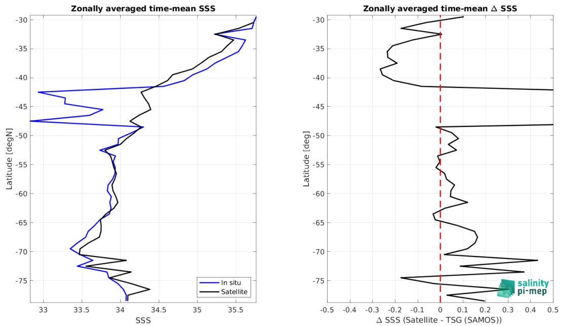
Figure 9: Left panel: Zonal mean SSS from SMOS SSS L3 Southern Ocean v1 - 9-Day running mean (BEC) satellite product (black) and from TSG (SAMOS) (blue). Right panel: Zonal mean of \Delta SSS (Satellite - TSG (SAMOS)) for all the collected Pi-MEP match-up pairs estimated over the full satellite product period.
