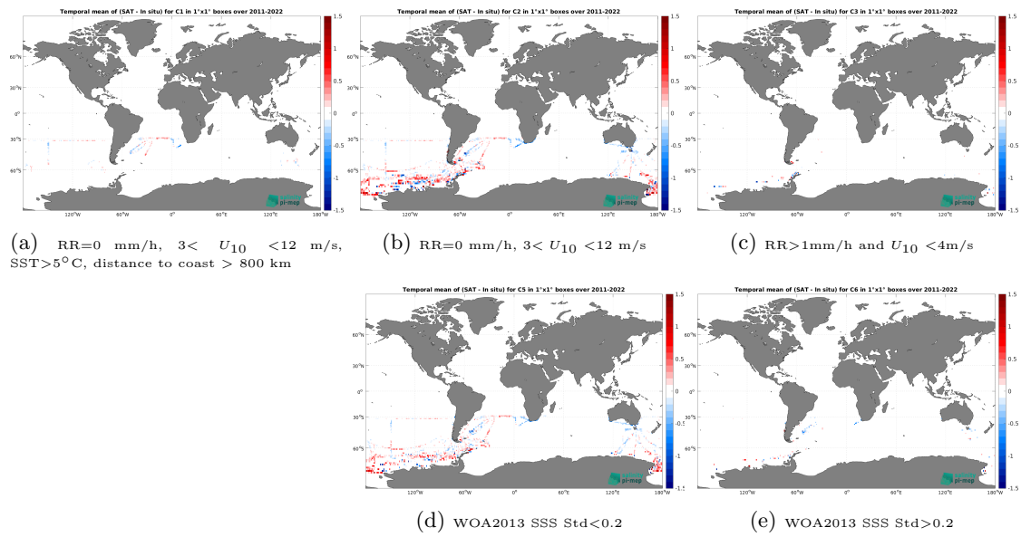
Figure 14: Temporal mean gridded over spatial boxes of size 1^\circ \times 1^\circ of \Delta SSS (SMOS SSS L3 Southern Ocean v1 - 9-Day running mean (BEC) - TSG (SAMOS)) for 5 different subdatasets corresponding to: RR=0 mm/h, 3 < U_{10} < 12 m/s, SST > 5^\circ\text{C} , distance to coast > 800 km (a), RR=0 mm/h, 3 < U_{10} < 12 m/s (b), RR > 1 mm/h and U_{10} < 4 m/s (c), WOA2013 SSS Std < 0.2 (d), WOA2013 SSS Std > 0.2 (e).
