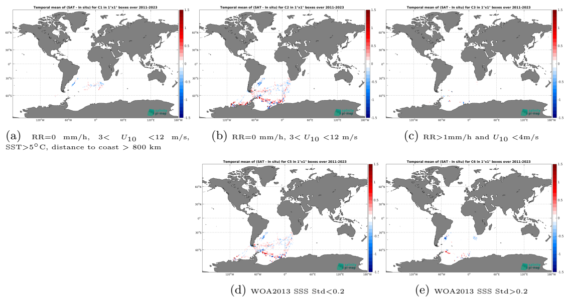
Figure 14: Temporal mean gridded over spatial boxes of size 1^\circ \times 1^\circ of \Delta SSS (SMOS SSS L3 Southern Ocean v1 - 9-Day running mean (BEC) - TSG (Polarstern)) for 5 different subdatasets corresponding to: RR=0 mm/h, 3 < U_{10} < 12 m/s, SST > 5^\circ\text{C} , distance to coast > 800 km (a), RR=0 mm/h, 3 < U_{10} < 12 m/s (b), RR > 1 mm/h and U_{10} < 4 m/s (c), WOA2013 SSS Std < 0.2 (d), WOA2013 SSS Std > 0.2 (e).
