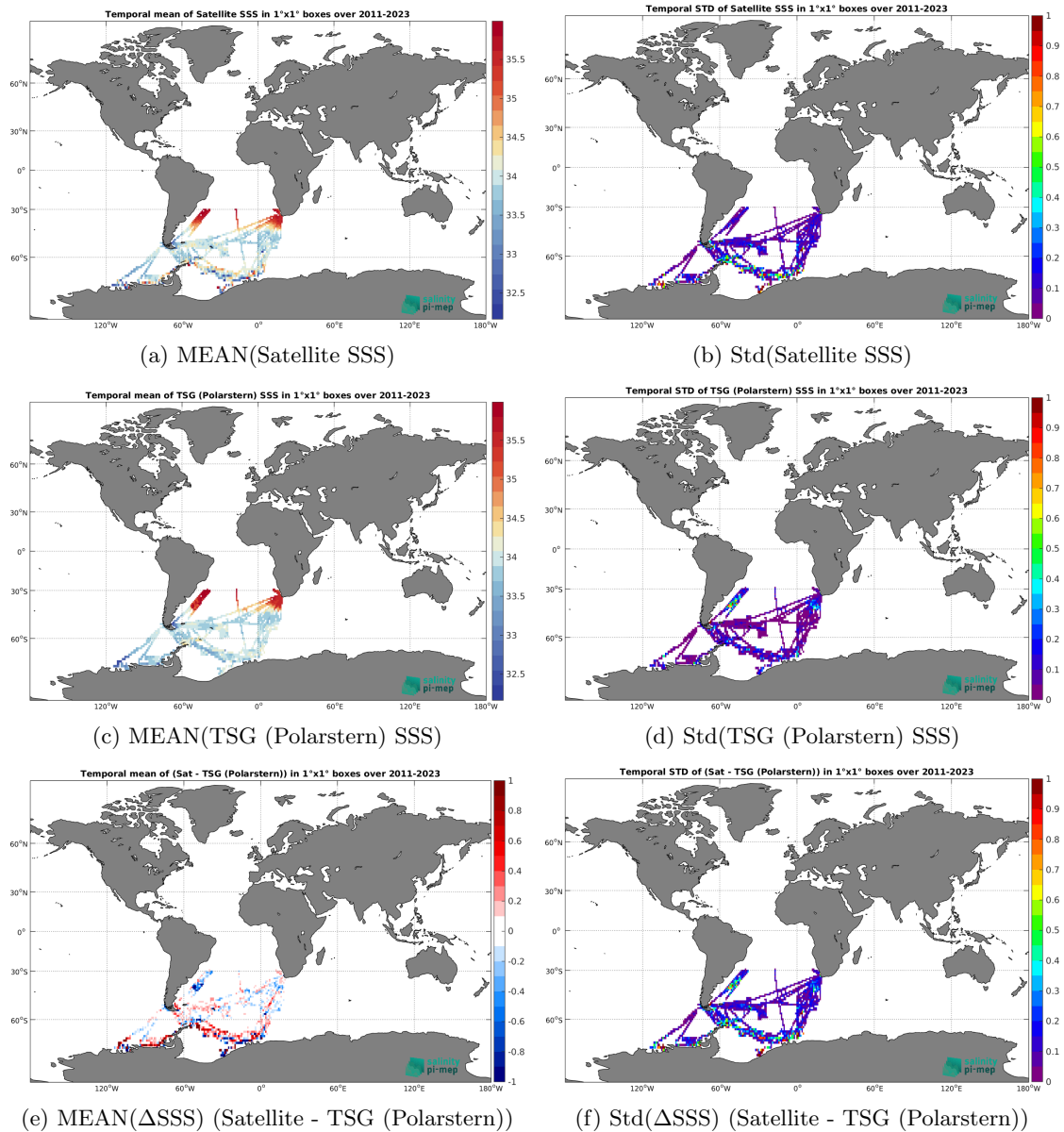
Figure 7: Temporal mean (left) and Std (right) of SSS from SMOS SSS L3 Southern Ocean v1 - 9-Day running mean (BEC) (top), TSG (Polarstern) (middle), and of \Delta SSS (Satellite - TSG (Polarstern)). Only match-up pairs are used to generate these maps.
