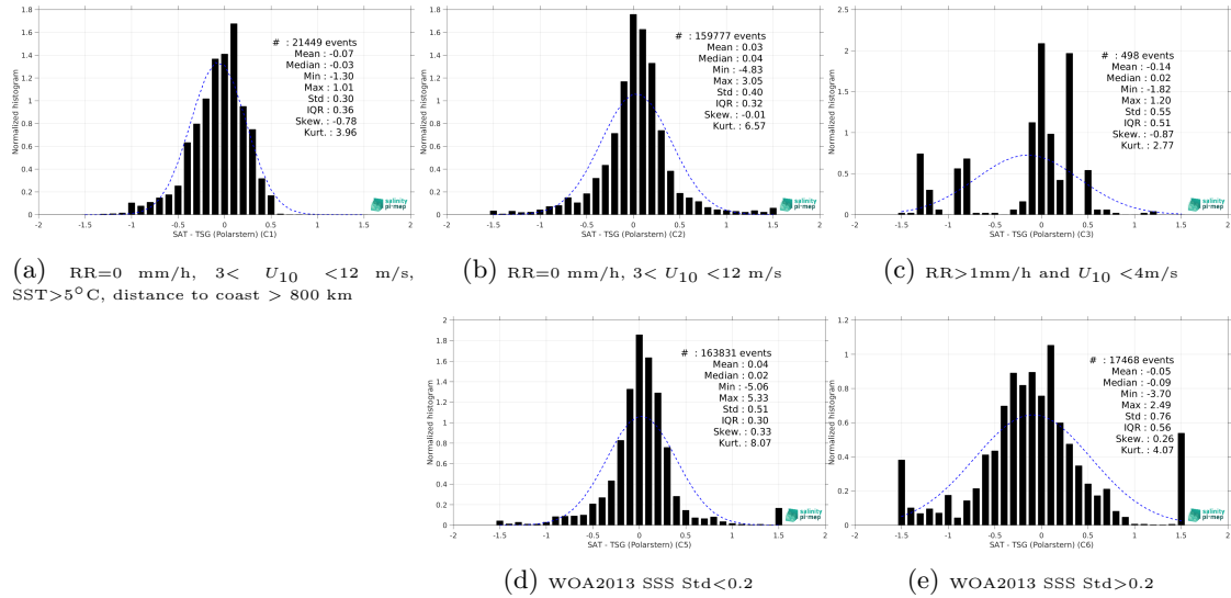
Figure 15: Normalized histogram of \Delta\text{SSS} (SMOS SSS L3 Southern Ocean v1 - 9-Day running mean (BEC) - TSG (Polarstern)) for 5 different subdatasets corresponding to: RR=0 mm/h, 3 < U_{10} < 12 m/s, SST>5°C, distance to coast > 800 km (a), RR=0 mm/h, 3 < U_{10} < 12 m/s (b), RR>1mm/h and U_{10} < 4 m/s (c), WOA2013 SSS Std<0.2 (d), WOA2013 SSS Std>0.2 (e).
