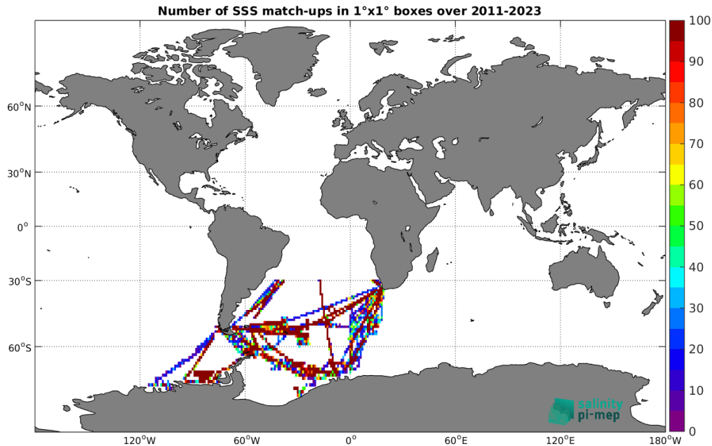
Figure 5: Number of SSS match-ups between TSG (Polarstern) SSS and the SMOS SSS L3 Southern Ocean v1 - 9-Day running mean (BEC) SSS product for the Global Ocean Pi-MEP region over 1^\circ \times 1^\circ boxes and for the full satellite product period.
