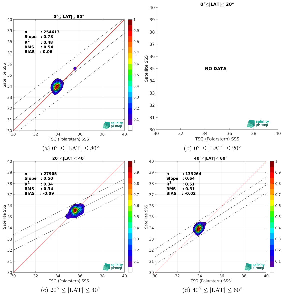
Figure 10: Contour maps of the concentration of SMOS SSS L3 Southern Ocean v1 - 9-Day running mean (BEC) SSS (y-axis) versus TSG (Polarstern) SSS (x-axis) at match-up pairs for different latitude bands. For each plot, the red line shows x=y . The black thin and dashed lines indicate a linear fit through the data cloud and the \pm 95\% confidence levels, respectively. The number match-up pairs n , the slope and R^2 coefficient of the linear fit, the root mean square (RMS) and the mean bias between satellite and in situ data are indicated for each latitude band in each plots.
