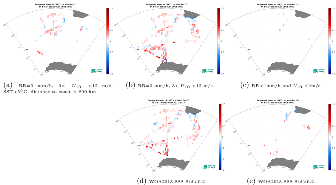
Figure 14: Temporal mean gridded over spatial boxes of size 1^\circ \times 1^\circ of \Delta SSS (SMOS SSS L3 Southern Ocean v1 - 9-Day running mean (BEC) - TSG (NCEI-0170743)) for 5 different sub-datasets corresponding to:RR=0 mm/h, 3 < U_{10} < 12 m/s, SST >5^\circ\text{C} , distance to coast > 800 km (a), RR=0 mm/h, 3 < U_{10} < 12 m/s (b), RR >1 mm/h and U_{10} < 4 m/s (c), WOA2013 SSS Std <0.2 (d), WOA2013 SSS Std >0.2 (e).
