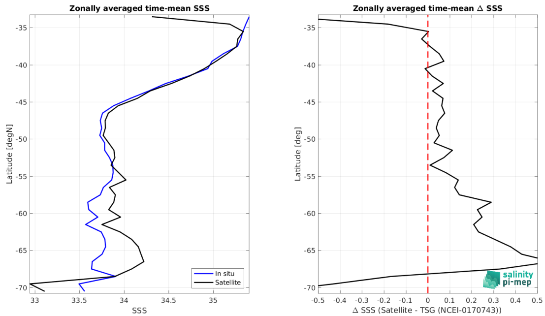
Figure 9: Left panel: Zonal mean SSS from SMOS SSS L3 Southern Ocean v1 - 9-Day running mean (BEC) satellite product (black) and from TSG (NCEI-0170743) (blue). Right panel: Zonal mean of \Delta SSS (Satellite - TSG (NCEI-0170743)) for all the collected Pi-MEP match-up pairs estimated over the full satellite product period.
