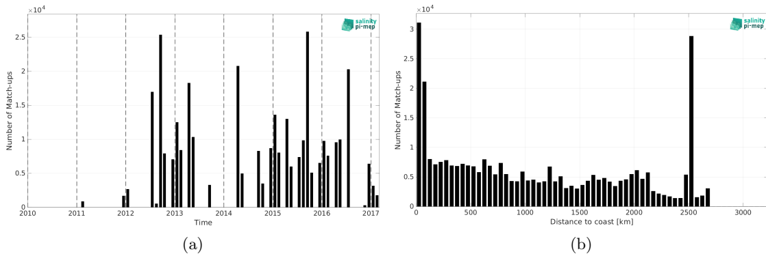
Figure 2: Number of match-ups between TSG (NCEI-0170743) and SMOS SSS L3 Southern Ocean v1 - 9-Day running mean (BEC) SSS as a function of time (a) and as function of the distance to coast (b) over the Global Ocean Pi-MEP region and for the full satellite product period.
