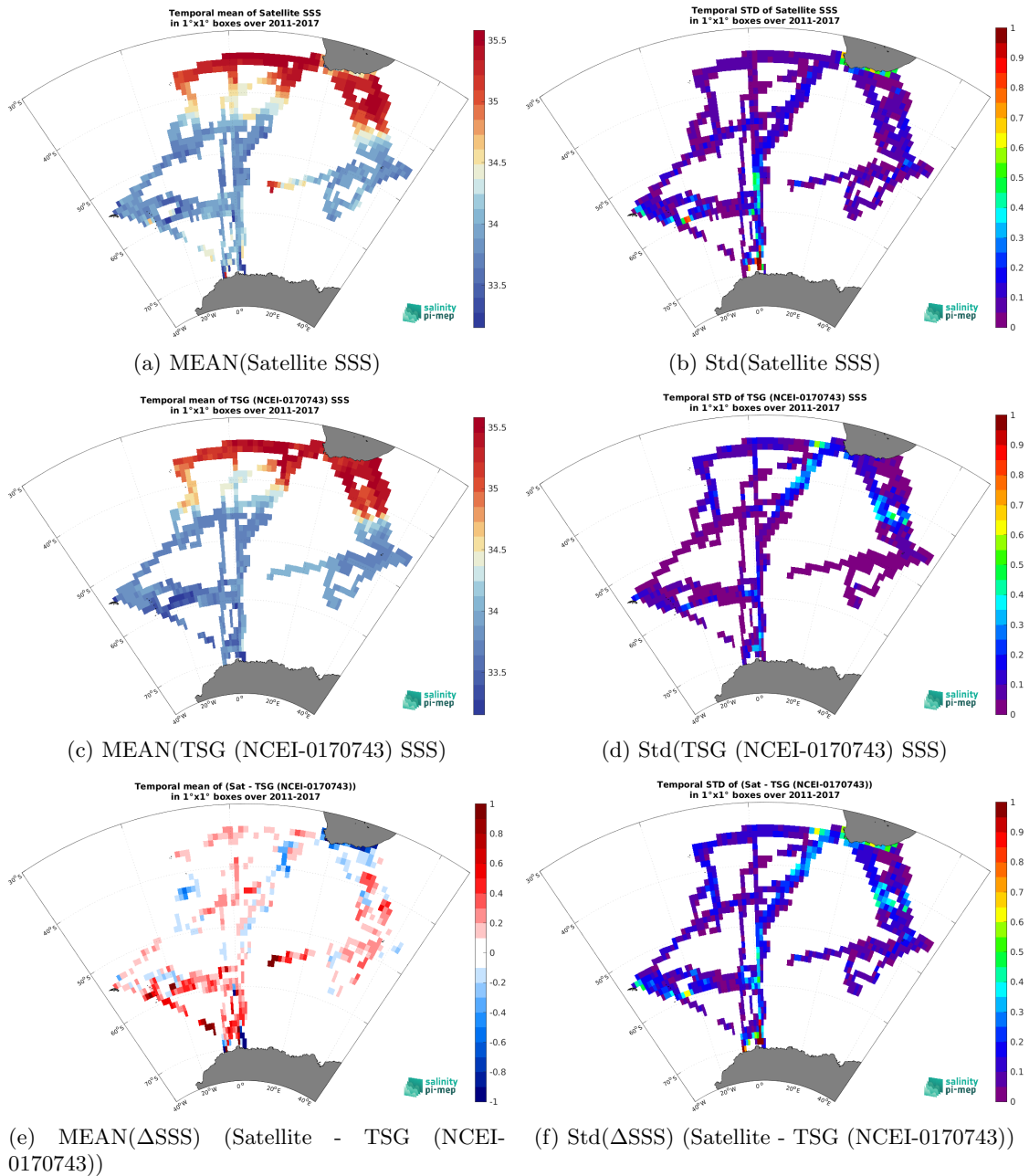
Figure 7: Temporal mean (left) and Std (right) of SSS from SMOS SSS L3 Southern Ocean v1 - 9-Day running mean (BEC) (top), TSG (NCEI-0170743) (middle), and of \Delta SSS (Satellite - TSG (NCEI-0170743)). Only match-up pairs are used to generate these maps.
