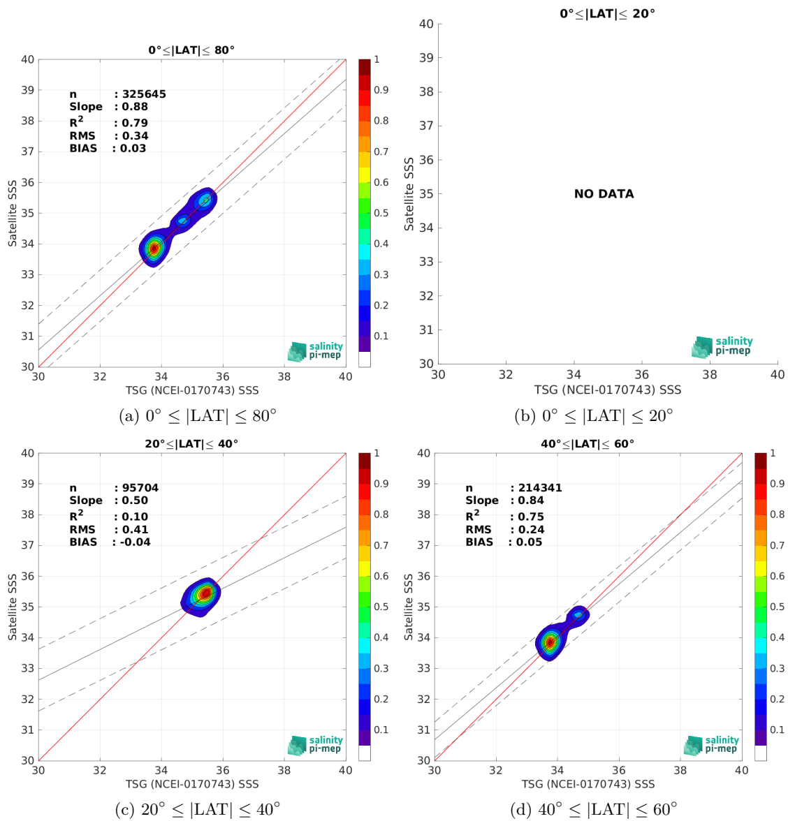
Figure 10: Contour maps of the concentration of SMOS SSS L3 Southern Ocean v1 - 9-Day running mean (BEC) SSS (y-axis) versus TSG (NCEI-0170743) SSS (x-axis) at match-up pairs for different latitude bands. For each plot, the red line shows x=y . The black thin and dashed lines indicate a linear fit through the data cloud and the \pm 95\% confidence levels, respectively. The number match-up pairs n , the slope and R^2 coefficient of the linear fit, the root mean square (RMS) and the mean bias between satellite and in situ data are indicated for each latitude band in each plots.
