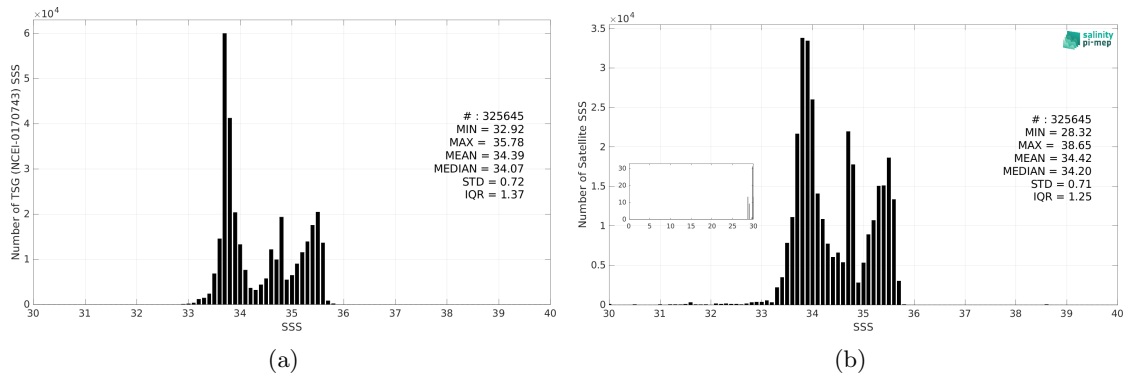
Figure 3: Histograms of SSS from TSG (NCEI-0170743) (a) and SMOS SSS L3 Southern Ocean v1 - 9-Day running mean (BEC) (b) considering all match-up pairs per bins of 0.1 over the Global Ocean Pi-MEP region and for the full satellite product period.
