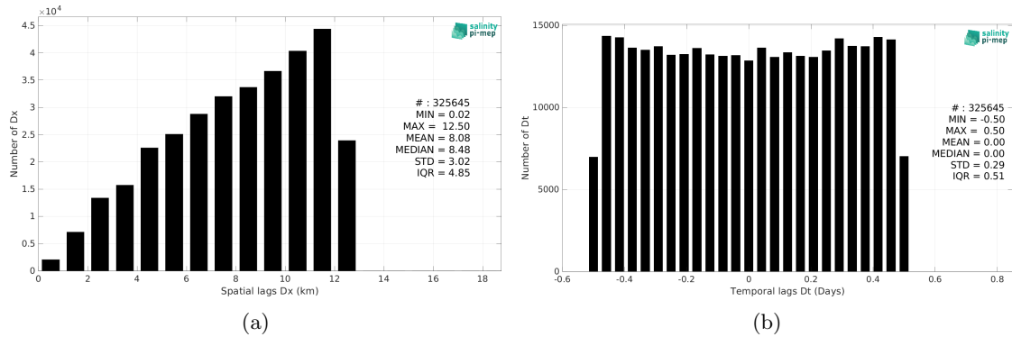
Figure 6: Histograms of the spatial (a) and temporal (b) lags between the location/time of the TSG (NCEI-0170743) measurement and the date of the corresponding SMOS SSS L3 Southern Ocean v1 - 9-Day running mean (BEC) SSS pixel.
