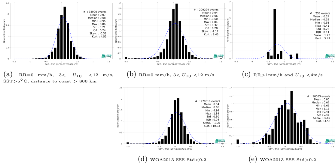
Figure 15: Normalized histogram of \Delta SSS (SMOS SSS L3 Southern Ocean v1 - 9-Day running mean (BEC) - TSG (NCEI-0170743)) for 5 different subdatasets corresponding to: RR=0 mm/h, 3 < U_{10} < 12 m/s, SST>5°C, distance to coast > 800 km (a), RR=0 mm/h, 3 < U_{10} < 12 m/s (b), RR>1mm/h and U_{10} < 4 m/s (c), WOA2013 SSS Std<0.2 (d), WOA2013 SSS Std>0.2 (e).
