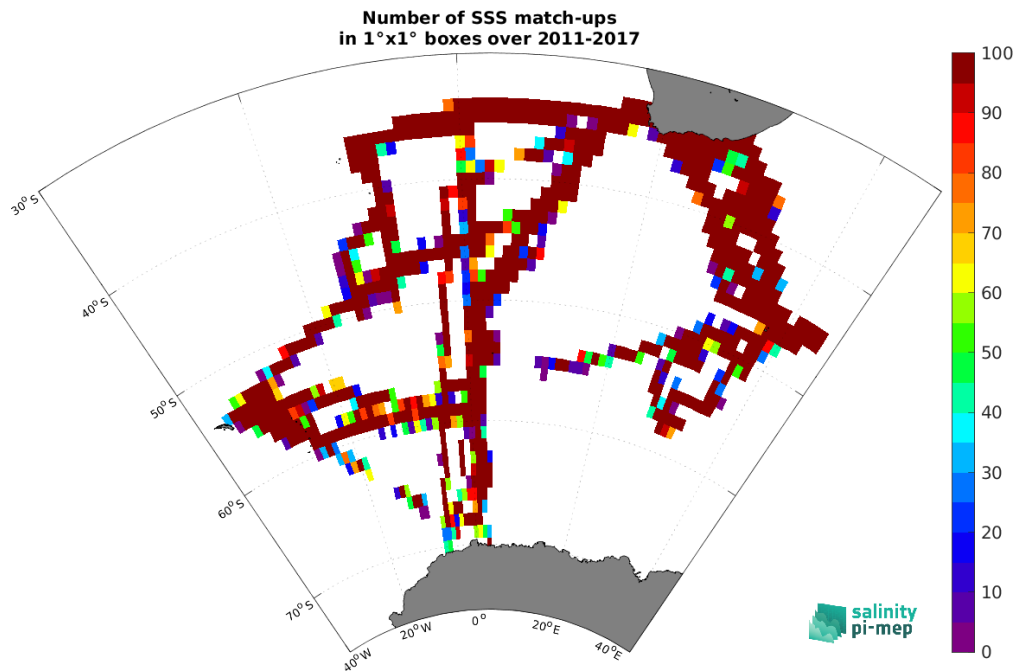
Figure 5: Number of SSS match-ups between TSG (NCEI-0170743) SSS and the SMOS SSS L3 Southern Ocean v1 - 9-Day running mean (BEC) SSS product for the Global Ocean Pi-MEP region over 1^\circ \times 1^\circ boxes and for the full satellite product period.
