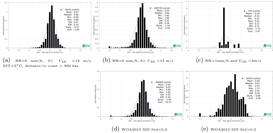
Figure 15: Normalized histogram of \Delta\text{SSS} (SMOS SSS L3 Southern Ocean v1 - 9-Day running mean (BEC) - TSG (NCEI-0170743)) for 5 different subdatasets corresponding to: RR=0 mm/h, 3 < U_{10} < 12 m/s, SST>5°C, distance to coast > 800 km (a), RR=0 mm/h, 3 < U_{10} < 12 m/s (b), RR>1mm/h and U_{10} < 4 m/s (c), WOA2013 SSS Std<0.2 (d), WOA2013 SSS Std>0.2 (e).
