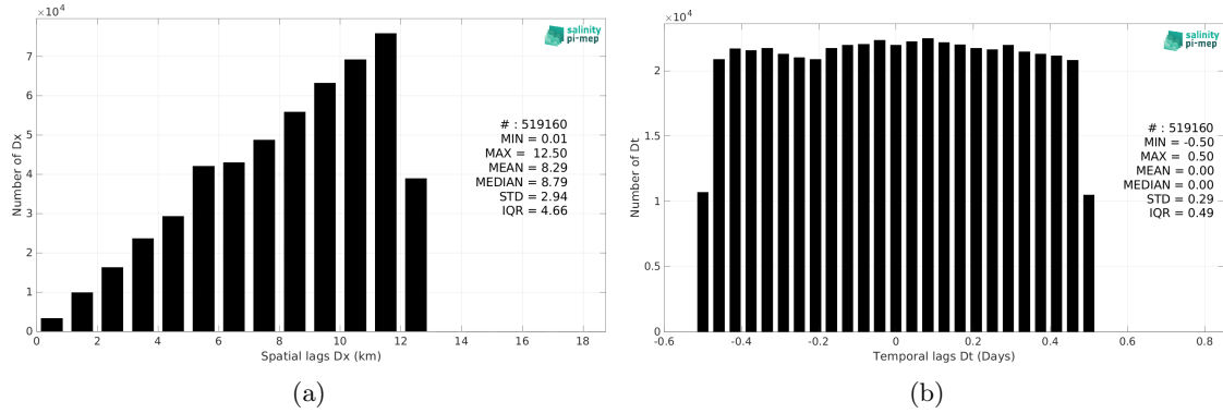
Figure 6: Histograms of the spatial (a) and temporal (b) lags between the location/time of the TSG (LEGOS-Survostral) measurement and the date of the corresponding SMOS SSS L3 Southern Ocean v1 - 9-Day running mean (BEC) SSS pixel.
