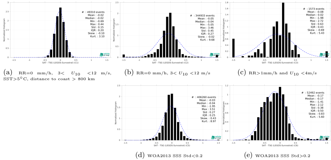
Figure 15: Normalized histogram of \Delta SSS (SMOS SSS L3 Southern Ocean v1 - 9-Day running mean (BEC) - TSG (LEGOS-Survostral)) for 5 different subdatasets corresponding to: RR=0 mm/h, 3 < U_{10} < 12 m/s, SST>5°C, distance to coast > 800 km (a), RR=0 mm/h, 3 < U_{10} < 12 m/s (b), RR>1mm/h and U_{10} < 4 m/s (c), WOA2013 SSS Std<0.2 (d), WOA2013 SSS Std>0.2 (e).
