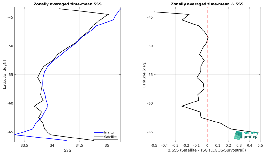
Figure 9: Left panel: Zonal mean SSS from SMOS SSS L3 Southern Ocean v1 - 9-Day running mean (BEC) satellite product (black) and from TSG (LEGOS-Survostral) (blue). Right panel: Zonal mean of \Delta SSS (Satellite - TSG (LEGOS-Survostral)) for all the collected Pi-MEP match-up pairs estimated over the full satellite product period.
