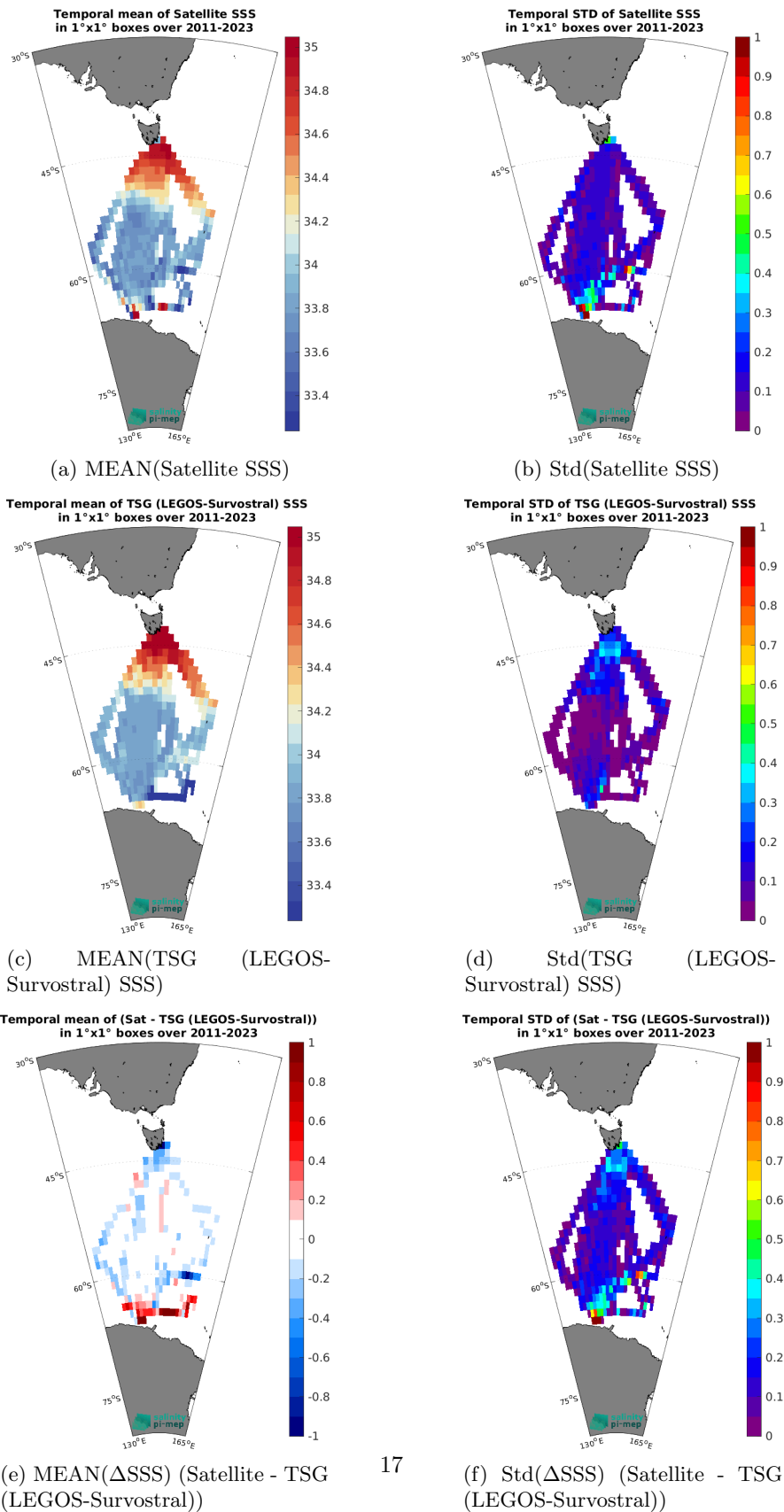
Figure 7: Temporal mean (left) and Std (right) of SSS from SMOS SSS L3 Southern Ocean v1 - 9-Day running mean (BEC) (top), TSG (LEGOS-Survostral) (middle), and of \Delta SSS (Satellite - TSG (LEGOS-Survostral)). Only match-up pairs are used to generate these maps.
