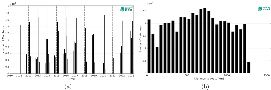
Figure 2: Number of match-ups between TSG (LEGOS-Survostral) and SMOS SSS L3 Southern Ocean v1 - 9-Day running mean (BEC) SSS as a function of time (a) and as function of the distance to coast (b) over the Global Ocean Pi-MEP region and for the full satellite product period.
