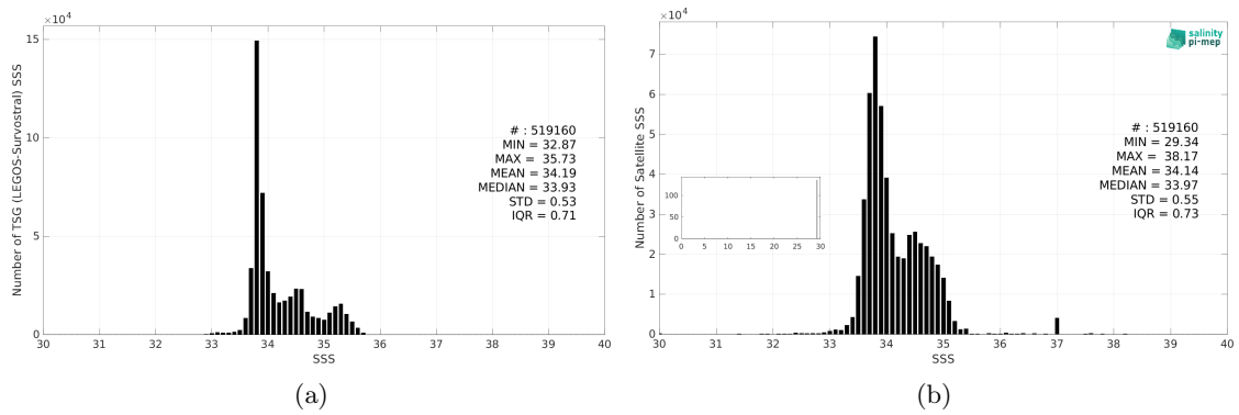
Figure 3: Histograms of SSS from TSG (LEGOS-Survostral) (a) and SMOS SSS L3 Southern Ocean v1 - 9-Day running mean (BEC) (b) considering all match-up pairs per bins of 0.1 over the Global Ocean Pi-MEP region and for the full satellite product period.
