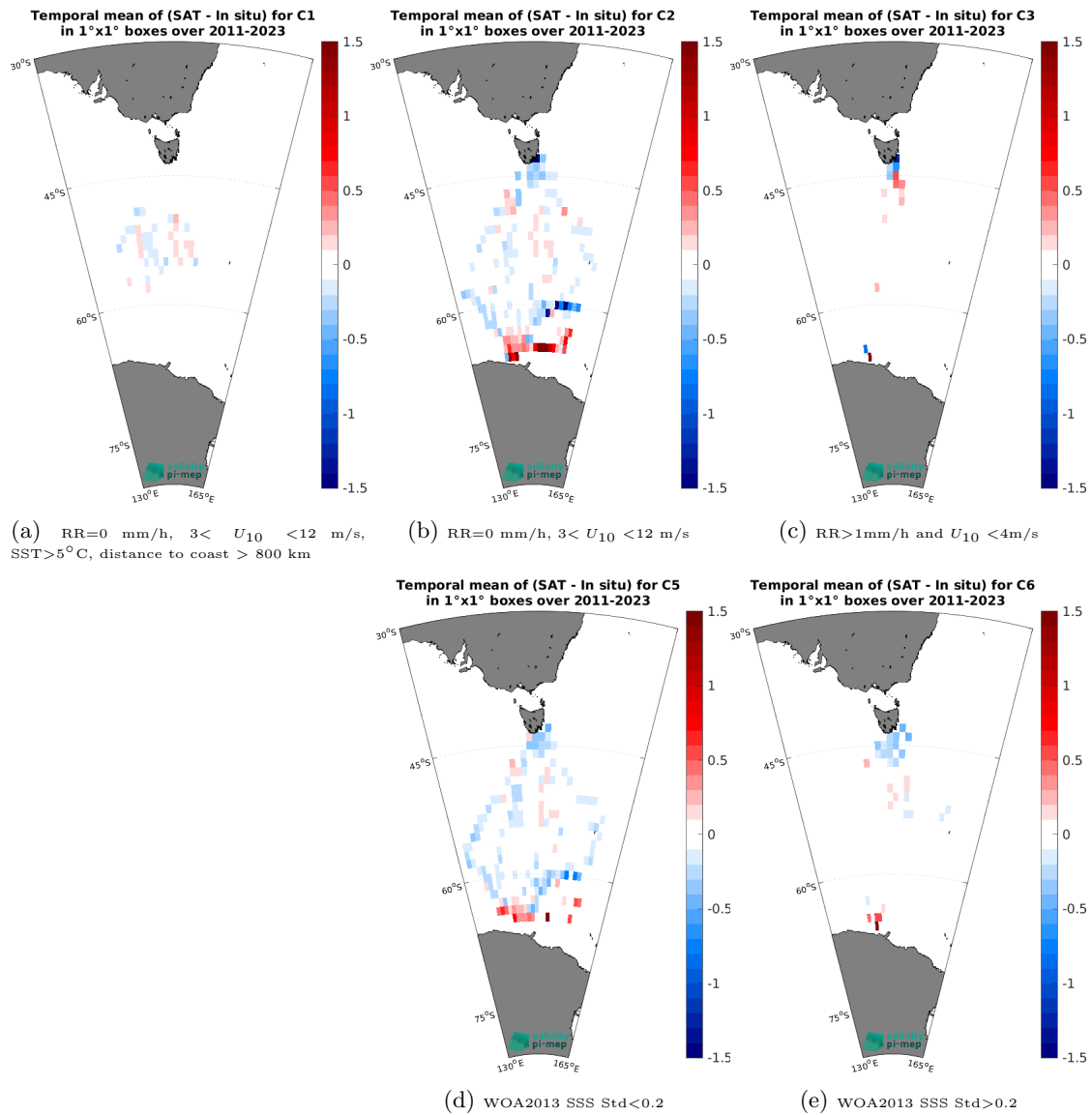
Figure 14: Temporal mean gridded over spatial boxes of size 1^\circ \times 1^\circ of \Delta\text{SSS} (SMOS SSS L3 Southern Ocean v1 - 9-Day running mean (BEC) - TSG (LEGOS-Survostral)) for 5 different subdatasets corresponding to: RR=0 mm/h, 3 < U_{10} < 12 m/s, SST > 5^\circ\text{C} , distance to coast > 800 km (a), RR=0 mm/h, 3 < U_{10} < 12 m/s (b), RR > 1 mm/h and U_{10} < 4 m/s (c), WOA2013 SSS Std < 0.2 (d), WOA2013 SSS Std > 0.2 (e).
