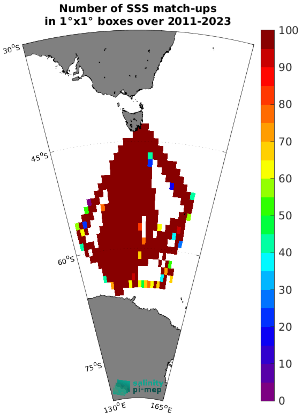
Figure 5: Number of SSS match-ups between TSG (LEGOS-Survostral) SSS and the SMOS SSS L3 Southern Ocean v1 - 9-Day running mean (BEC) SSS product for the Global Ocean Pi-MEP region over 1°x1° boxes and for the full satellite product period.
