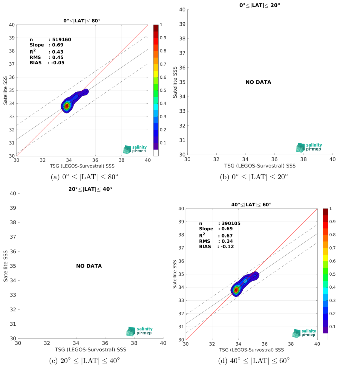
Figure 10: Contour maps of the concentration of SMOS SSS L3 Southern Ocean v1 - 9-Day running mean (BEC) SSS (y-axis) versus TSG (LEGOS-Survostral) SSS (x-axis) at match-up pairs for different latitude bands. For each plot, the red line shows x=y . The black thin and dashed lines indicate a linear fit through the data cloud and the \pm 95\% confidence levels, respectively. The number match-up pairs n , the slope and R^2 coefficient of the linear fit, the root mean square (RMS) and the mean bias between satellite and in situ data are indicated for each latitude band in each plots.
