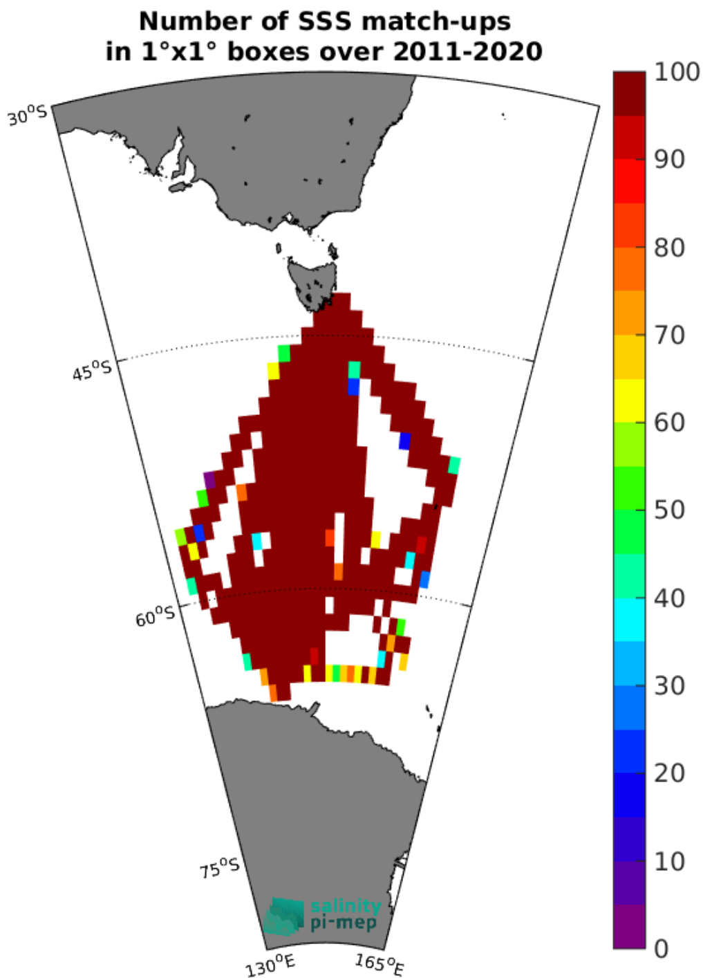
Figure 5: Number of SSS match-ups between TSG (LEGOS-Survostral) SSS and the SMOS SSS L3 Southern Ocean v1 - 9-Day running mean (BEC) SSS product for the Global Ocean Pi-MEP region over 1°x1° boxes and for the full satellite product period.
