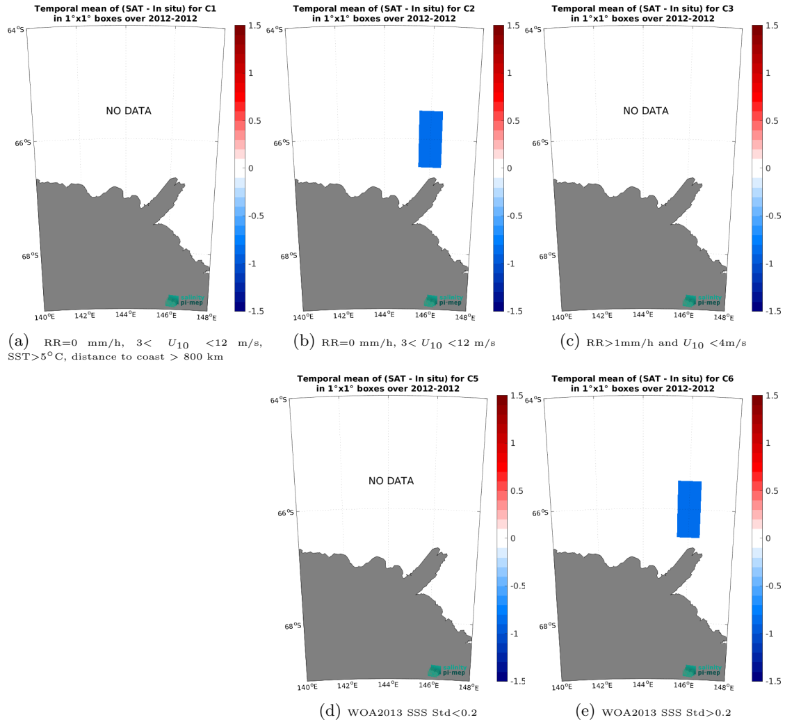
Figure 14: Temporal mean gridded over spatial boxes of size 1^{\circ} \times 1^{\circ} of \Delta SSS (SMOS SSS L3 Southern Ocean v1 - 9-Day running mean (BEC) - TSG (LEGOS-Surv-Adel)) for 5 different subdatasets corresponding to: RR=0 mm/h, 3 < U_{10} < 12 m/s, SST > 5°C, distance to coast > 800 km (a), RR=0 mm/h, 3 < U_{10} < 12 m/s (b), RR > 1mm/h and U_{10} < 4 m/s (c), WOA2013 SSS Std < 0.2 (d), WOA2013 SSS Std > 0.2 (e).
