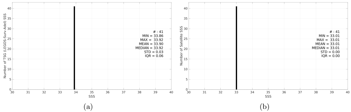
Figure 3: Histograms of SSS from TSG (LEGOS-Surv-Adel) (a) and SMOS SSS L3 Southern Ocean v1 - 9-Day running mean (BEC) (b) considering all match-up pairs per bins of 0.1 over the Global Ocean Pi-MEP region and for the full satellite product period.
