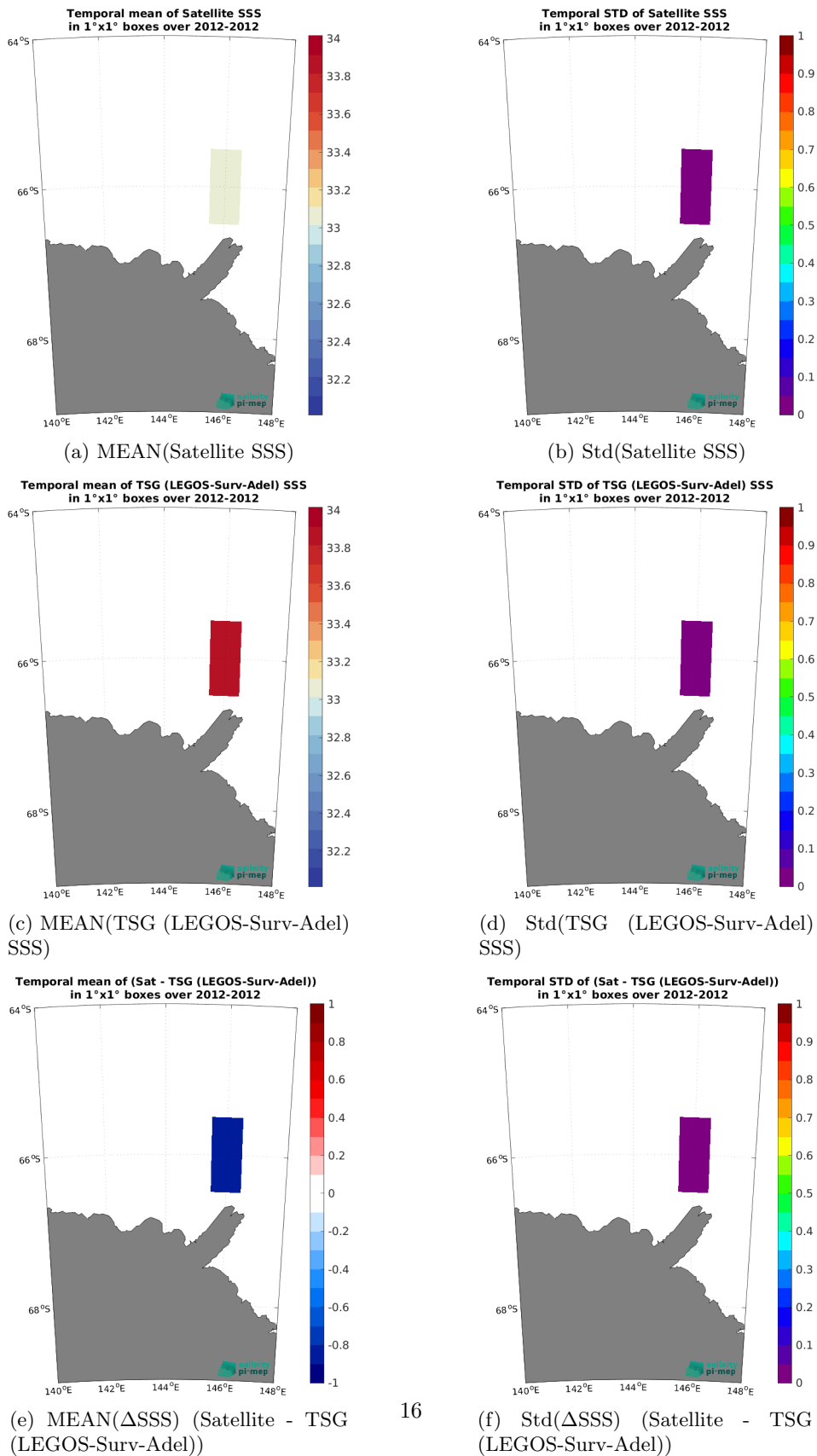
Figure 7: Temporal mean (left) and Std (right) of SSS from SMOS SSS L3 Southern Ocean v1 - 9-Day running mean (BEC) (top), TSG (LEGOS-Surv-Adel) (middle), and of \Delta SSS (Satellite - TSG (LEGOS-Surv-Adel)). Only match-up pairs are used to generate these maps.
