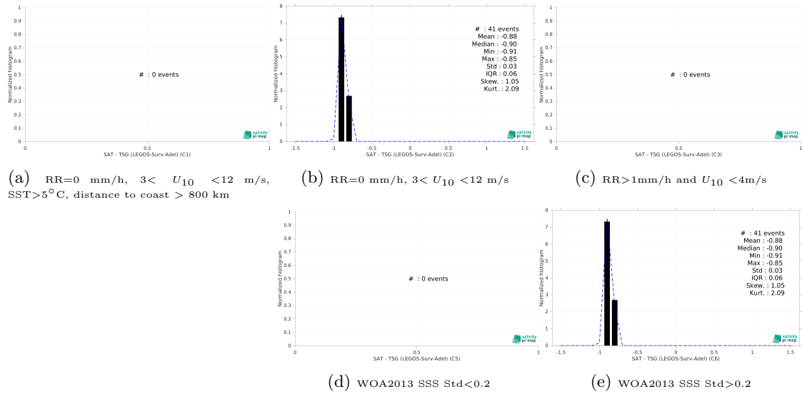
Figure 15: Normalized histogram of \Delta\text{SSS} (SMOS SSS L3 Southern Ocean v1 - 9-Day running mean (BEC) - TSG (LEGOS-Surv-Adel)) for 5 different subdatasets corresponding to: RR=0 mm/h, 3 < U_{10} < 12 m/s, SST > 5^{\circ}\text{C} , distance to coast > 800 km (a), RR=0 mm/h, 3 < U_{10} < 12 m/s (b), RR > 1\text{mm/h} and U_{10} < 4\text{m/s} (c), WOA2013 SSS Std < 0.2 (d), WOA2013 SSS Std > 0.2 (e).
