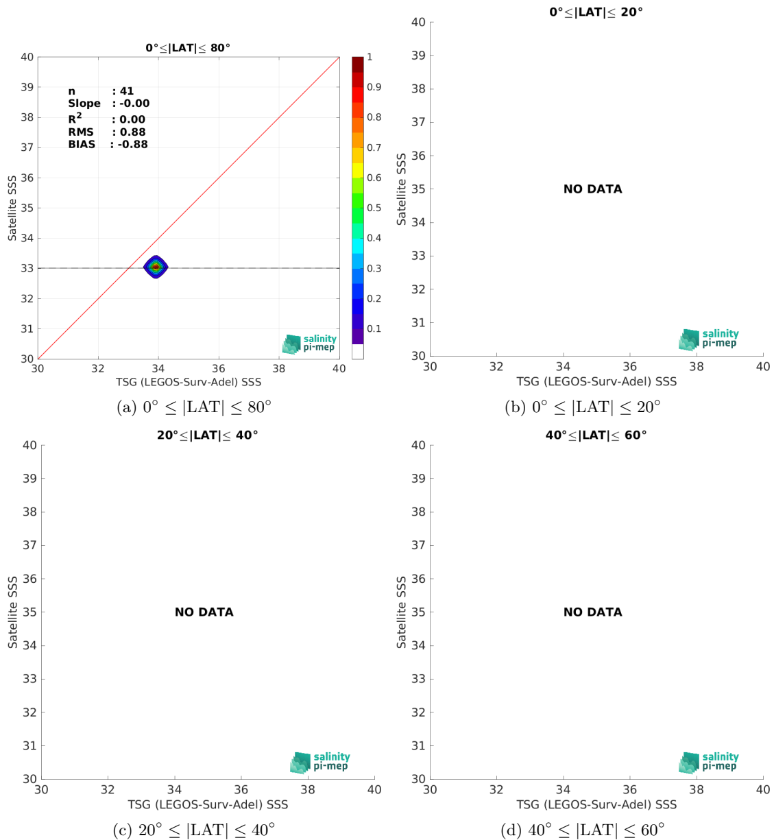
Figure 10: Contour maps of the concentration of SMOS SSS L3 Southern Ocean v1 - 9-Day running mean (BEC) SSS (y-axis) versus TSG (LEGOS-Surv-Adel) SSS (x-axis) at match-up pairs for different latitude bands. For each plot, the red line shows x=y . The black thin and dashed lines indicate a linear fit through the data cloud and the \pm 95\% confidence levels, respectively. The number match-up pairs n , the slope and R^2 coefficient of the linear fit, the root mean square (RMS) and the mean bias between satellite and in situ data are indicated for each latitude band in each plots.
