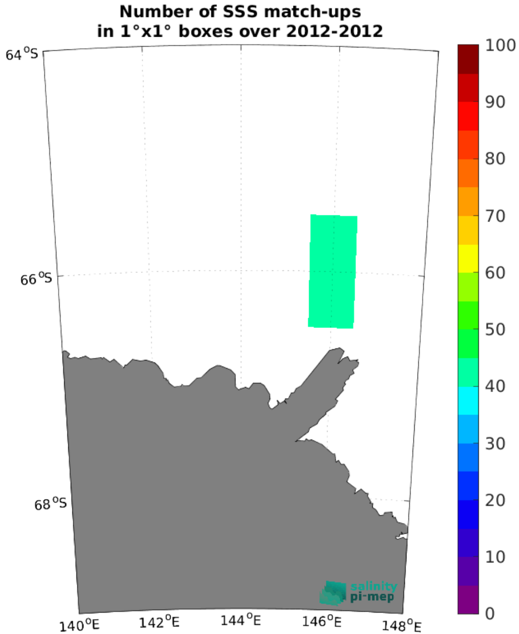
Figure 5: Number of SSS match-ups between TSG (LEGOS-Surv-Adel) SSS and the SMOS SSS L3 Southern Ocean v1 - 9-Day running mean (BEC) SSS product for the Global Ocean Pi-MEP region over 1^\circ \times 1^\circ boxes and for the full satellite product period.
