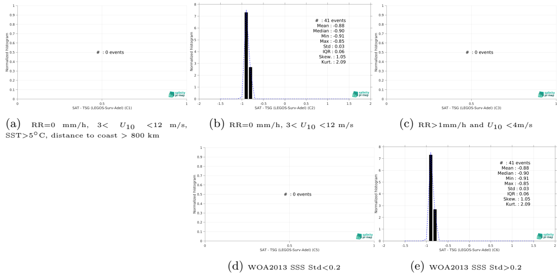
Figure 15: Normalized histogram of \Delta SSS (SMOS SSS L3 Southern Ocean v1 - 9-Day running mean (BEC) - TSG (LEGOS-Surv-Adel)) for 5 different subdatasets corresponding to: RR=0 mm/h, 3 < U_{10} < 12 m/s, SST>5°C, distance to coast > 800 km (a), RR=0 mm/h, 3 < U_{10} < 12 m/s (b), RR>1mm/h and U_{10} < 4 m/s (c), WOA2013 SSS Std<0.2 (d), WOA2013 SSS Std>0.2 (e).
