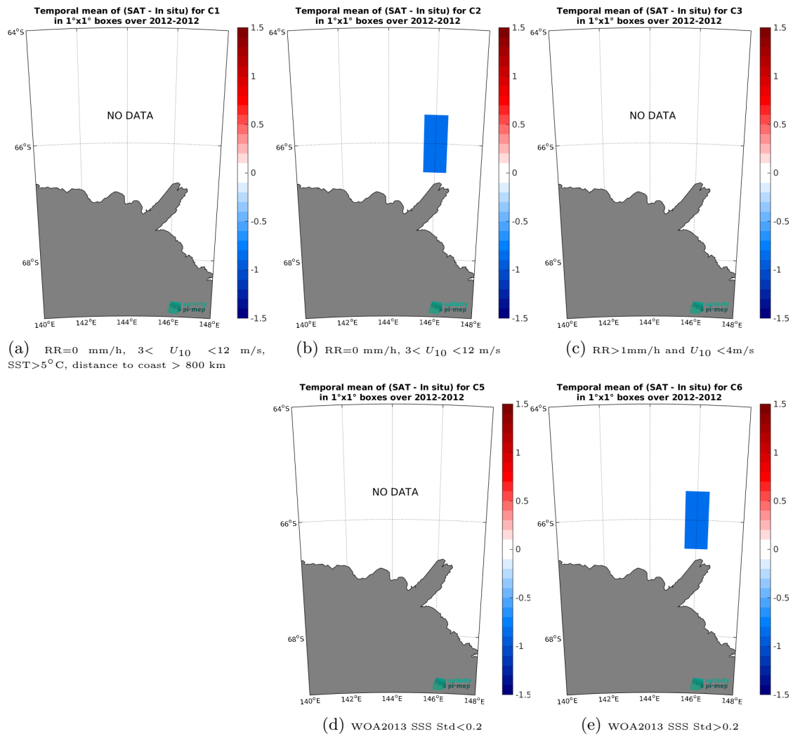
Figure 14: Temporal mean gridded over spatial boxes of size 1^\circ \times 1^\circ of \Delta SSS (SMOS SSS L3 Southern Ocean v1 - 9-Day running mean (BEC) - TSG (LEGOS-Surv-Adel)) for 5 different subdatasets corresponding to: RR=0 mm/h, 3 < U_{10} < 12 m/s, SST>5°C, distance to coast > 800 km (a), RR=0 mm/h, 3 < U_{10} < 12 m/s (b), RR>1mm/h and U_{10} < 4 m/s (c), WOA2013 SSS Std<0.2 (d), WOA2013 SSS Std>0.2 (e).
