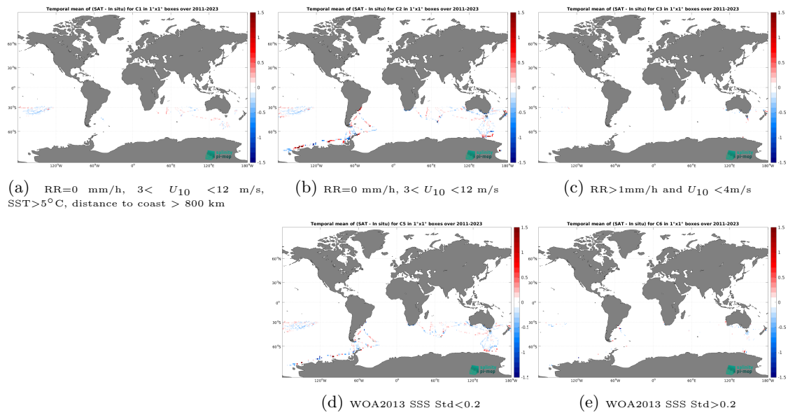
Figure 14: Temporal mean gridded over spatial boxes of size 1^\circ \times 1^\circ of \Delta SSS (SMOS SSS L3 Southern Ocean v1 - 9-Day running mean (BEC) - TSG (LEGOS-DM)) for 5 different subdatasets corresponding to: RR=0 mm/h, 3 < U_{10} < 12 m/s, SST > 5^\circ\text{C} , distance to coast > 800 km (a), RR=0 mm/h, 3 < U_{10} < 12 m/s (b), RR > 1 mm/h and U_{10} < 4 m/s (c), WOA2013 SSS Std < 0.2 (d), WOA2013 SSS Std > 0.2 (e).
