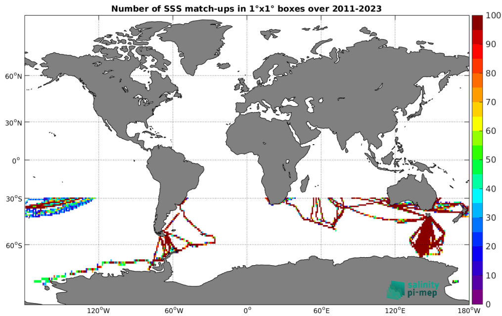
Figure 5: Number of SSS match-ups between TSG (LEGOS-DM) SSS and the SMOS SSS L3 Southern Ocean v1 - 9-Day running mean (BEC) SSS product for the Global Ocean Pi-MEP region over 1^\circ \times 1^\circ boxes and for the full satellite product period.
