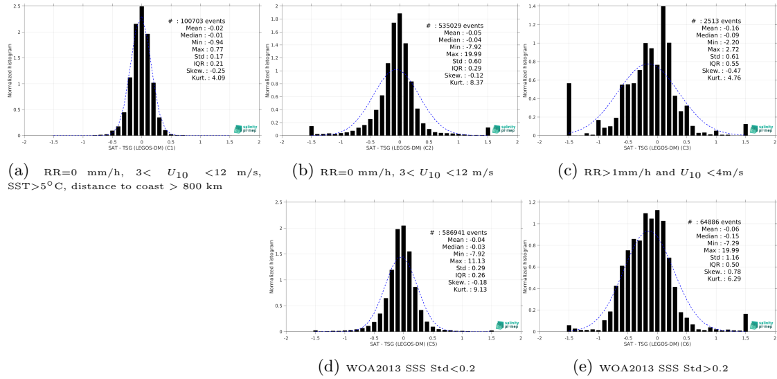
Figure 15: Normalized histogram of \Delta SSS (SMOS SSS L3 Southern Ocean v1 - 9-Day running mean (BEC) - TSG (LEGOS-DM)) for 5 different subdatasets corresponding to: RR=0 mm/h, 3 < U_{10} < 12 m/s, SST>5°C, distance to coast > 800 km (a), RR=0 mm/h, 3 < U_{10} < 12 m/s (b), RR>1mm/h and U_{10} < 4 m/s (c), WOA2013 SSS Std<0.2 (d), WOA2013 SSS Std>0.2 (e).
