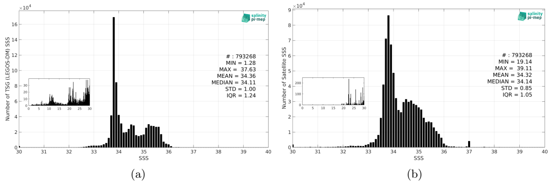
Figure 3: Histograms of SSS from TSG (LEGOS-DM) (a) and SMOS SSS L3 Southern Ocean v1 - 9-Day running mean (BEC) (b) considering all match-up pairs per bins of 0.1 over the Global Ocean Pi-MEP region and for the full satellite product period.
