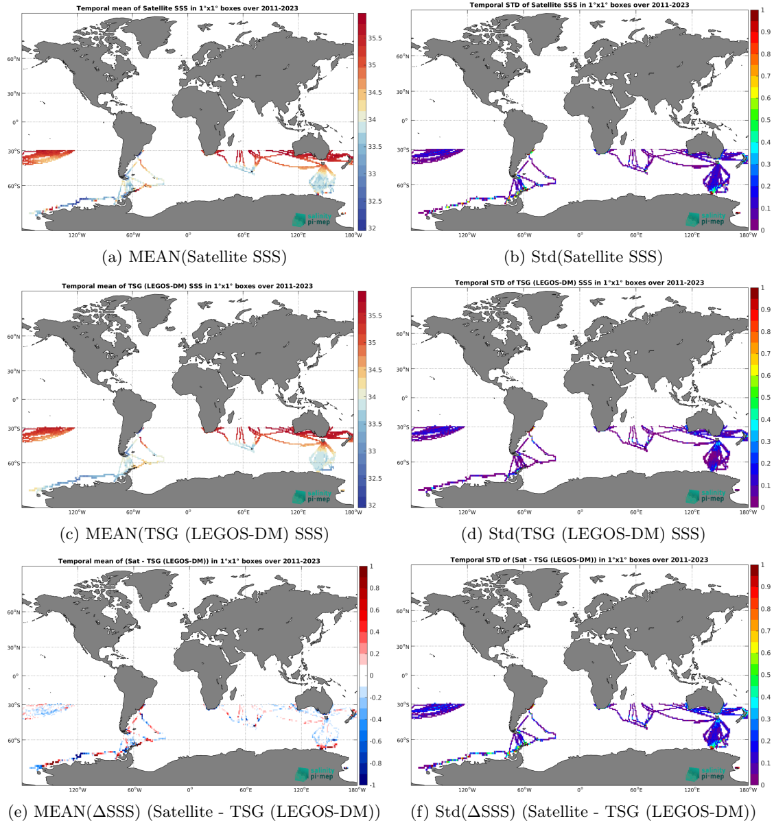
Figure 7: Temporal mean (left) and Std (right) of SSS from SMOS SSS L3 Southern Ocean v1 - 9-Day running mean (BEC) (top), TSG (LEGOS-DM) (middle), and of \Delta SSS (Satellite - TSG (LEGOS-DM)). Only match-up pairs are used to generate these maps.
