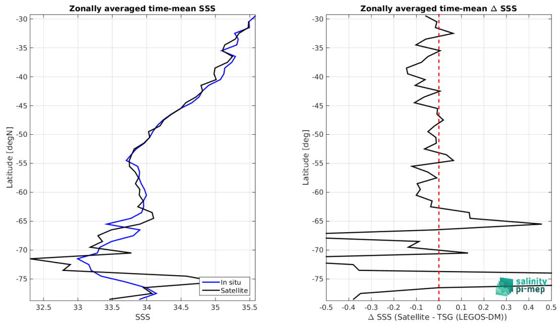
Figure 9: Left panel: Zonal mean SSS from SMOS SSS L3 Southern Ocean v1 - 9-Day running mean (BEC) satellite product (black) and from TSG (LEGOS-DM) (blue). Right panel: Zonal mean of \Delta SSS (Satellite - TSG (LEGOS-DM)) for all the collected Pi-MEP match-up pairs estimated over the full satellite product period.
