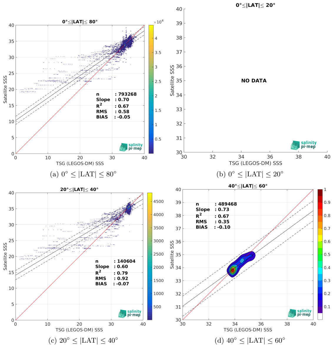
Figure 10: Contour maps of the concentration of SMOS SSS L3 Southern Ocean v1 - 9-Day running mean (BEC) SSS (y-axis) versus TSG (LEGOS-DM) SSS (x-axis) at match-up pairs for different latitude bands. For each plot, the red line shows x=y . The black thin and dashed lines indicate a linear fit through the data cloud and the \pm 95\% confidence levels, respectively. The number match-up pairs n , the slope and R^2 coefficient of the linear fit, the root mean square (RMS) and the mean bias between satellite and in situ data are indicated for each latitude band in each plots.
