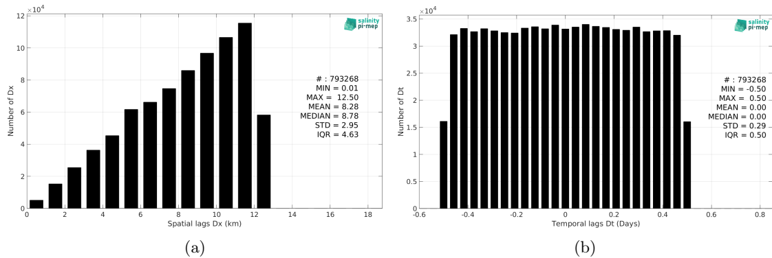
Figure 6: Histograms of the spatial (a) and temporal (b) lags between the location/time of the TSG (LEGOS-DM) measurement and the date of the corresponding SMOS SSS L3 Southern Ocean v1 - 9-Day running mean (BEC) SSS pixel.
