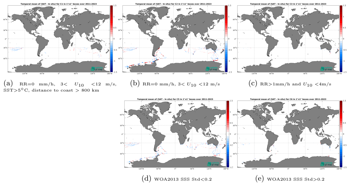
Figure 14: Temporal mean gridded over spatial boxes of size 1^\circ \times 1^\circ of \Delta\text{SSS} (SMOS SSS L3 Southern Ocean v1 - 9-Day running mean (BEC) - TSG (LEGOS-DM)) for 5 different subdatasets corresponding to: RR=0 mm/h, 3 < U_{10} < 12 m/s, SST > 5°C, distance to coast > 800 km (a), RR=0 mm/h, 3 < U_{10} < 12 m/s (b), RR > 1mm/h and U_{10} < 4 m/s (c), WOA2013 SSS Std < 0.2 (d), WOA2013 SSS Std > 0.2 (e).
