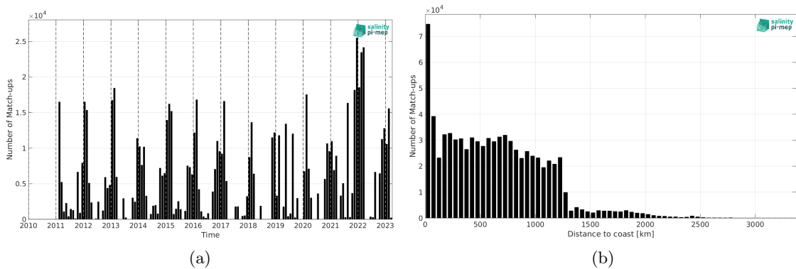
Figure 2: Number of match-ups between TSG (LEGOS-DM) and SMOS SSS L3 Southern Ocean v1 - 9-Day running mean (BEC) SSS as a function of time (a) and as function of the distance to coast (b) over the Global Ocean Pi-MEP region and for the full satellite product period.
