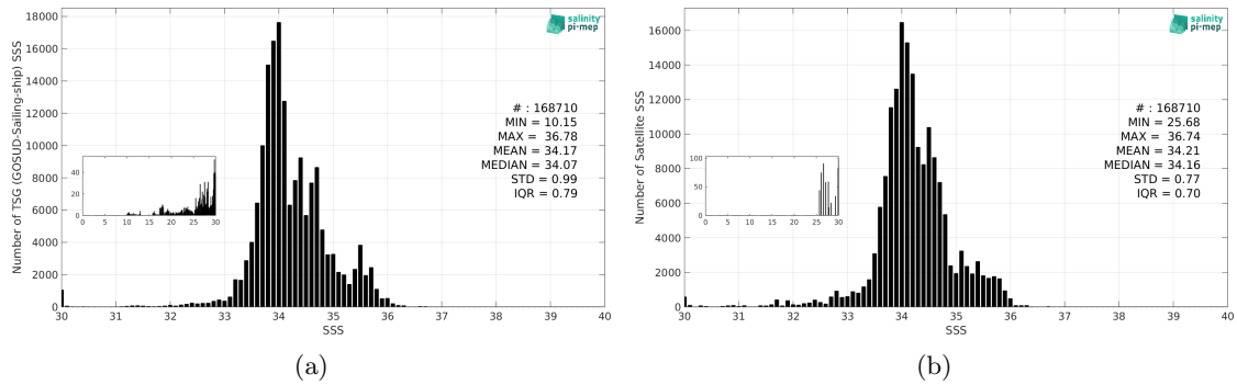
Figure 3: Histograms of SSS from TSG (GOSUD-Sailing-ship) (a) and SMOS SSS L3 Southern Ocean v1 - 9-Day running mean (BEC) (b) considering all match-up pairs per bins of 0.1 over the Global Ocean Pi-MEP region and for the full satellite product period.
