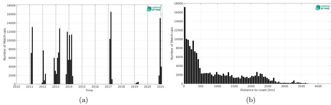
Figure 2: Number of match-ups between TSG (GOSUD-Sailing-ship) and SMOS SSS L3 Southern Ocean v1 - 9-Day running mean (BEC) SSS as a function of time (a) and as function of the distance to coast (b) over the Global Ocean Pi-MEP region and for the full satellite product period.
