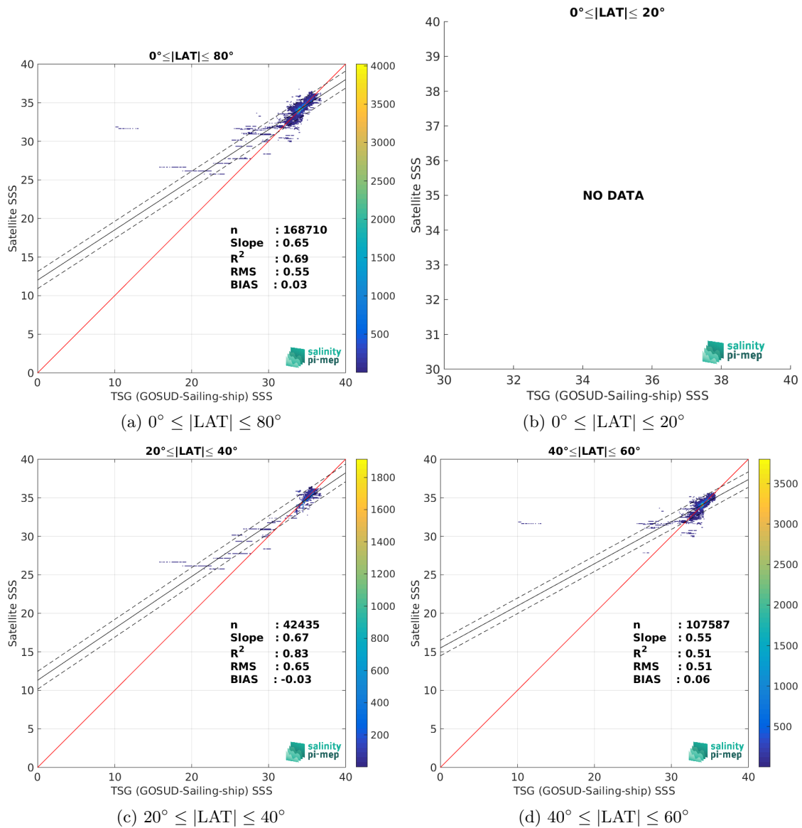
Figure 10: Contour maps of the concentration of SMOS SSS L3 Southern Ocean v1 - 9-Day running mean (BEC) SSS (y-axis) versus TSG (GOSUD-Sailing-ship) SSS (x-axis) at match-up pairs for different latitude bands. For each plot, the red line shows x=y . The black thin and dashed lines indicate a linear fit through the data cloud and the \pm 95\% confidence levels, respectively. The number match-up pairs n , the slope and R^2 coefficient of the linear fit, the root mean square (RMS) and the mean bias between satellite and in situ data are indicated for each latitude band in each plots.
