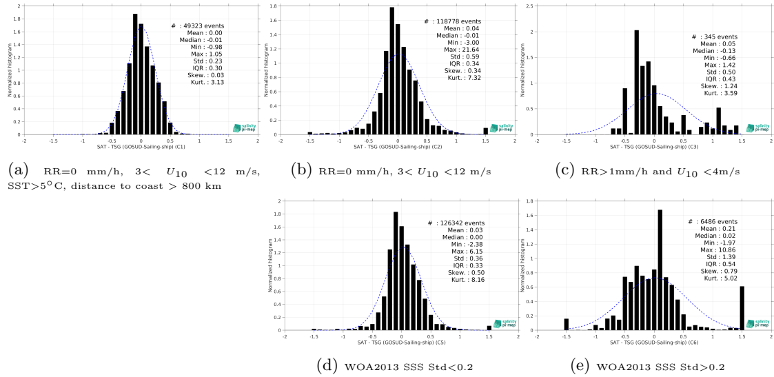
Figure 15: Normalized histogram of \Delta\text{SSS} (SMOS SSS L3 Southern Ocean v1 - 9-Day running mean (BEC) - TSG (GOSUD-Sailing-ship)) for 5 different subdatasets corresponding to: RR=0 mm/h, 3 < U_{10} < 12 m/s, SST>5°C, distance to coast > 800 km (a), RR=0 mm/h, 3 < U_{10} < 12 m/s (b), RR>1mm/h and U_{10} < 4 m/s (c), WOA2013 SSS Std<0.2 (d), WOA2013 SSS Std>0.2 (e).
