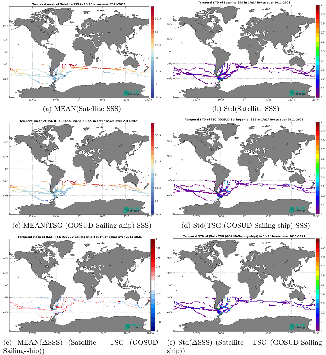
Figure 7: Temporal mean (left) and Std (right) of SSS from SMOS SSS L3 Southern Ocean v1 - 9-Day running mean (BEC) (top), TSG (GOSUD-Sailing-ship) (middle), and of \Delta SSS (Satellite - TSG (GOSUD-Sailing-ship)). Only match-up pairs are used to generate these maps.
