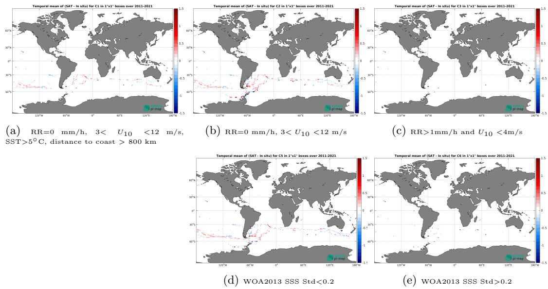
Figure 14: Temporal mean gridded over spatial boxes of size 1^\circ \times 1^\circ of \Delta SSS (SMOS SSS L3 Southern Ocean v1 - 9-Day running mean (BEC) - TSG (GOSUD-Sailing-ship)) for 5 different subdatasets corresponding to:RR=0 mm/h, 3 < U_{10} < 12 m/s, SST > 5^\circ\text{C} , distance to coast > 800 km (a), RR=0 mm/h, 3 < U_{10} < 12 m/s (b), RR > 1 mm/h and U_{10} < 4 m/s (c), WOA2013 SSS Std < 0.2 (d), WOA2013 SSS Std > 0.2 (e).
