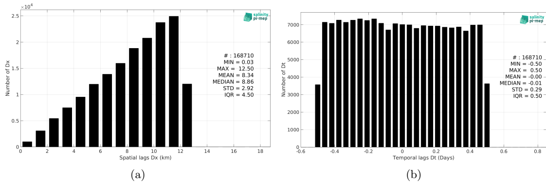
Figure 6: Histograms of the spatial (a) and temporal (b) lags between the location/time of the TSG (GOSUD-Sailing-ship) measurement and the date of the corresponding SMOS SSS L3 Southern Ocean v1 - 9-Day running mean (BEC) SSS pixel.
