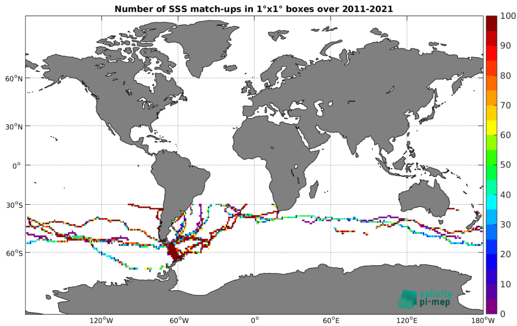
Figure 5: Number of SSS match-ups between TSG (GOSUD-Sailing-ship) SSS and the SMOS SSS L3 Southern Ocean v1 - 9-Day running mean (BEC) SSS product for the Global Ocean Pi-MEP region over 1^\circ \times 1^\circ boxes and for the full satellite product period.
