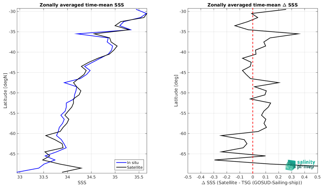
Figure 9: Left panel: Zonal mean SSS from SMOS SSS L3 Southern Ocean v1 - 9-Day running mean (BEC) satellite product (black) and from TSG (GOSUD-Sailing-ship) (blue). Right panel: Zonal mean of \Delta SSS (Satellite - TSG (GOSUD-Sailing-ship)) for all the collected Pi-MEP match-up pairs estimated over the full satellite product period.
