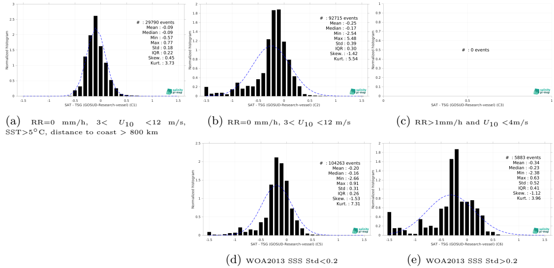
Figure 15: Normalized histogram of \Delta SSS (SMOS SSS L3 Southern Ocean v1 - 9-Day running mean (BEC) - TSG (GOSUD-Research-vessel)) for 5 different subdatasets corresponding to: RR=0 mm/h, 3 < U_{10} < 12 m/s, SST > 5°C, distance to coast > 800 km (a), RR=0 mm/h, 3 < U_{10} < 12 m/s (b), RR > 1mm/h and U_{10} < 4 m/s (c), WOA2013 SSS Std < 0.2 (d), WOA2013 SSS Std > 0.2 (e).
