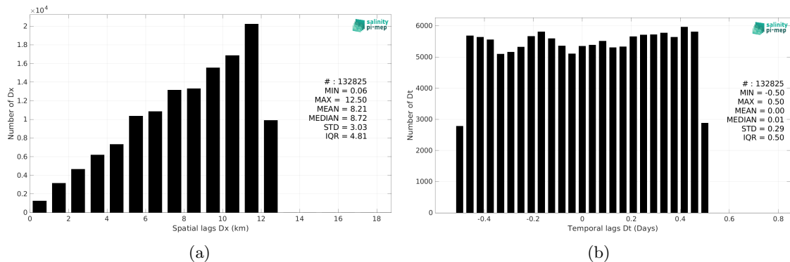
Figure 6: Histograms of the spatial (a) and temporal (b) lags between the location/time of the TSG (GOSUD-Research-vessel) measurement and the date of the corresponding SMOS SSS L3 Southern Ocean v1 - 9-Day running mean (BEC) SSS pixel.
