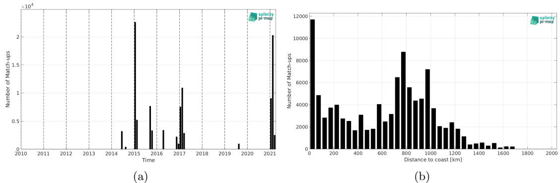
Figure 2: Number of match-ups between TSG (GOSUD-Research-vessel) and SMOS SSS L3 Southern Ocean v1 - 9-Day running mean (BEC) SSS as a function of time (a) and as function of the distance to coast (b) over the Global Ocean Pi-MEP region and for the full satellite product period.
