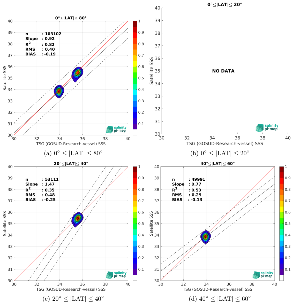
Figure 10: Contour maps of the concentration of SMOS SSS L3 Southern Ocean v1 - 9-Day running mean (BEC) SSS (y-axis) versus TSG (GOSUD-Research-vessel) SSS (x-axis) at match-up pairs for different latitude bands. For each plot, the red line shows x=y . The black thin and dashed lines indicate a linear fit through the data cloud and the \pm 95\% confidence levels, respectively. The number match-up pairs n , the slope and R^2 coefficient of the linear fit, the root mean square (RMS) and the mean bias between satellite and in situ data are indicated for each latitude band in each plots.
