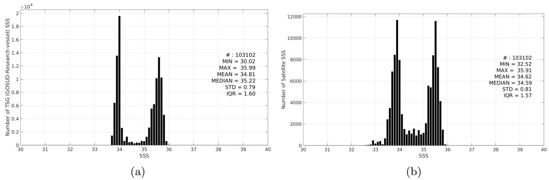
Figure 3: Histograms of SSS from TSG (GOSUD-Research-vessel) (a) and SMOS SSS L3 Southern Ocean v1 - 9-Day running mean (BEC) (b) considering all match-up pairs per bins of 0.1 over the Global Ocean Pi-MEP region and for the full satellite product period.
