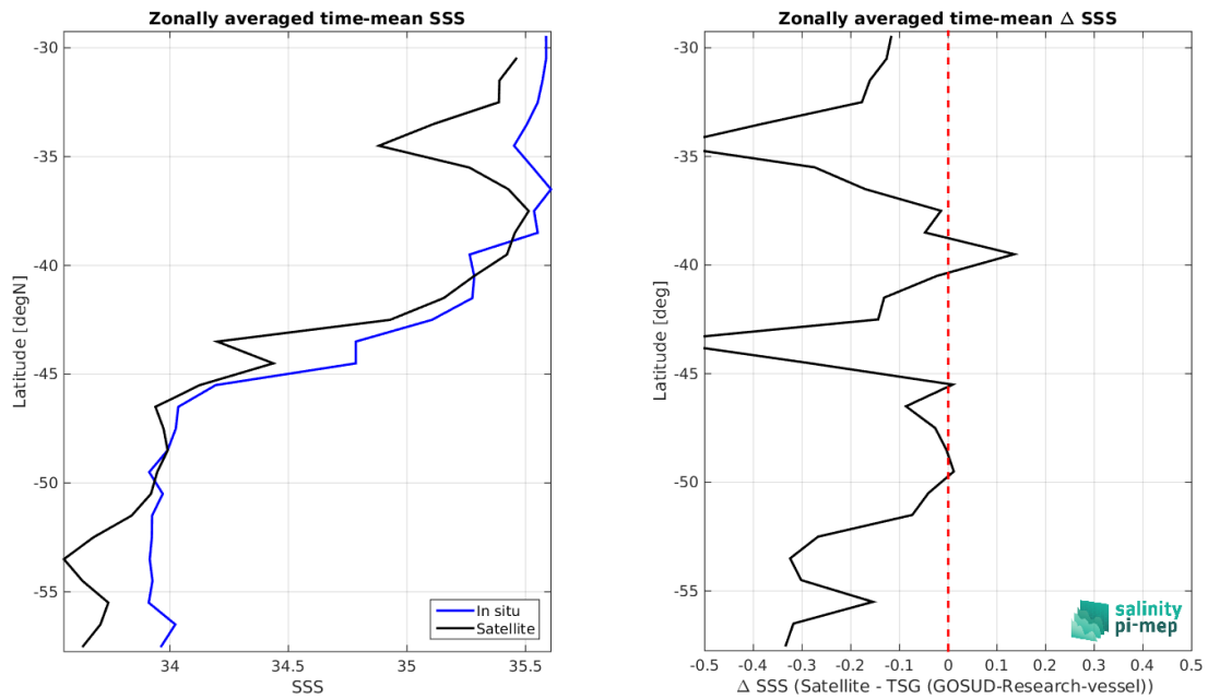
Figure 9: Left panel: Zonal mean SSS from SMOS SSS L3 Southern Ocean v1 - 9-Day running mean (BEC) satellite product (black) and from TSG (GOSUD-Research-vessel) (blue). Right panel: Zonal mean of \Delta SSS (Satellite - TSG (GOSUD-Research-vessel)) for all the collected Pi-MEP match-up pairs estimated over the full satellite product period.
