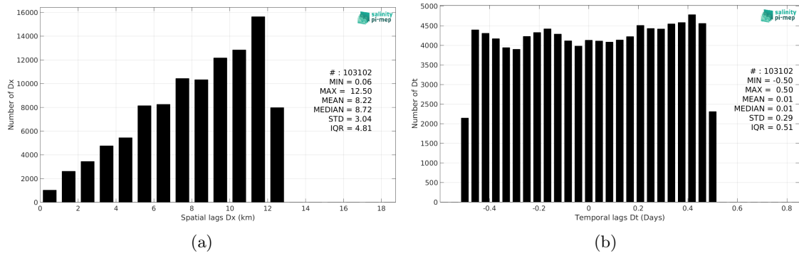
Figure 6: Histograms of the spatial (a) and temporal (b) lags between the location/time of the TSG (GOSUD-Research-vessel) measurement and the date of the corresponding SMOS SSS L3 Southern Ocean v1 - 9-Day running mean (BEC) SSS pixel.
