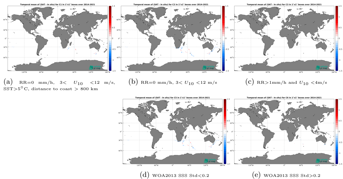
Figure 14: Temporal mean gridded over spatial boxes of size 1^\circ \times 1^\circ of \Delta SSS (SMOS SSS L3 Southern Ocean v1 - 9-Day running mean (BEC) - TSG (GOSUD-Research-vessel)) for 5 different subdatasets corresponding to:RR=0 mm/h, 3 < U_{10} < 12 m/s, SST > 5^\circ C, distance to coast > 800 km (a), RR=0 mm/h, 3 < U_{10} < 12 m/s (b), RR > 1 mm/h and U_{10} < 4 m/s (c), WOA2013 SSS Std < 0.2 (d), WOA2013 SSS Std > 0.2 (e).
