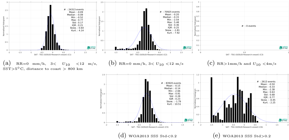
Figure 15: Normalized histogram of \Delta SSS (SMOS SSS L3 Southern Ocean v1 - 9-Day running mean (BEC) - TSG (GOSUD-Research-vessel)) for 5 different subdatasets corresponding to: RR=0 mm/h, 3 < U_{10} < 12 m/s, SST > 5°C, distance to coast > 800 km (a), RR=0 mm/h, 3 < U_{10} < 12 m/s (b), RR > 1mm/h and U_{10} < 4 m/s (c), WOA2013 SSS Std < 0.2 (d), WOA2013 SSS Std > 0.2 (e).
