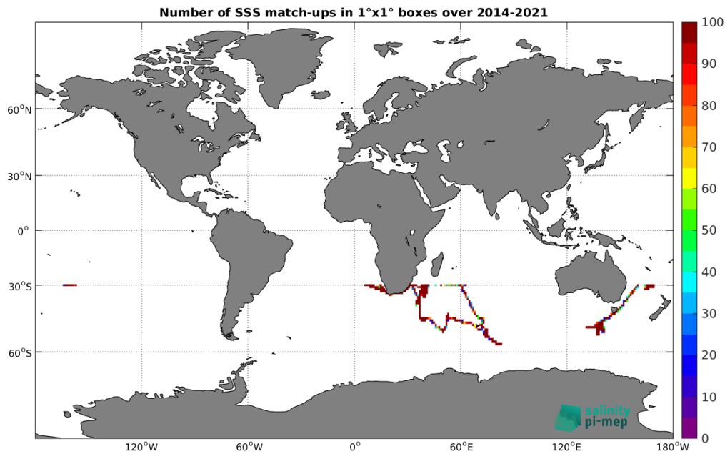
Figure 5: Number of SSS match-ups between TSG (GOSUD-Research-vessel) SSS and the SMOS SSS L3 Southern Ocean v1 - 9-Day running mean (BEC) SSS product for the Global Ocean Pi-MEP region over 1^\circ \times 1^\circ boxes and for the full satellite product period.
