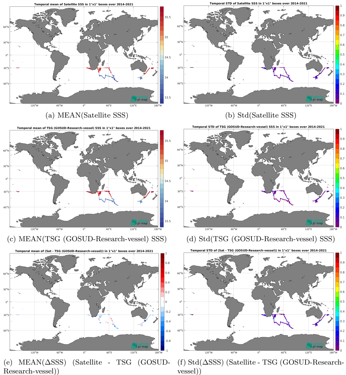
Figure 7: Temporal mean (left) and Std (right) of SSS from SMOS SSS L3 Southern Ocean v1 - 9-Day running mean (BEC) (top), TSG (GOSUD-Research-vessel) (middle), and of \Delta SSS (Satellite - TSG (GOSUD-Research-vessel)). Only match-up pairs are used to generate these maps.
