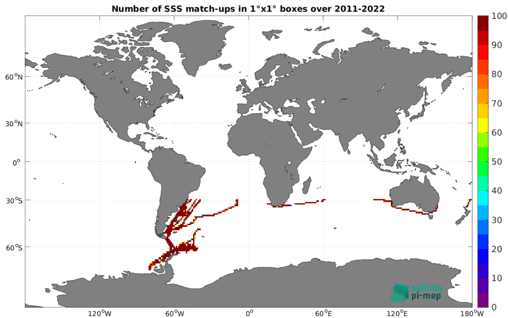
Figure 5: Number of SSS match-ups between TSG (CSIC-UTM) SSS and the SMOS SSS L3 Southern Ocean v1 - 9-Day running mean (BEC) SSS product for the Global Ocean Pi-MEP region over 1^\circ \times 1^\circ boxes and for the full satellite product period.
