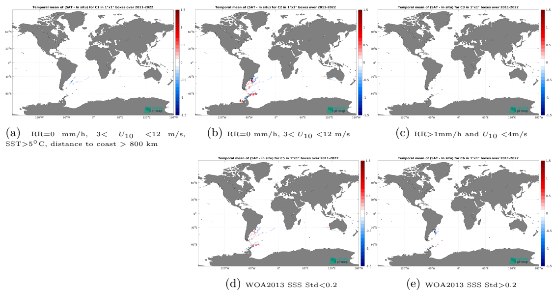
Figure 14: Temporal mean gridded over spatial boxes of size 1^\circ \times 1^\circ of \Delta SSS (SMOS SSS L3 Southern Ocean v1 - 9-Day running mean (BEC) - TSG (CSIC-UTM)) for 5 different subdatasets corresponding to: RR=0 mm/h, 3 < U_{10} < 12 m/s, SST > 5^\circ\text{C} , distance to coast > 800 km (a), RR=0 mm/h, 3 < U_{10} < 12 m/s (b), RR > 1 mm/h and U_{10} < 4 m/s (c), WOA2013 SSS Std < 0.2 (d), WOA2013 SSS Std > 0.2 (e).
