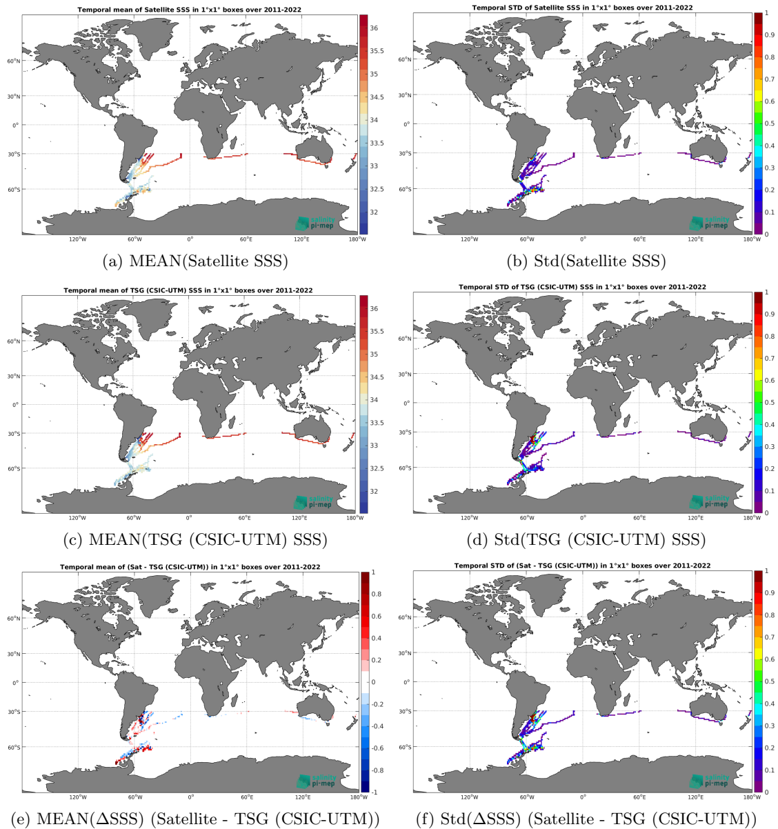
Figure 7: Temporal mean (left) and Std (right) of SSS from SMOS SSS L3 Southern Ocean v1 - 9-Day running mean (BEC) (top), TSG (CSIC-UTM) (middle), and of \Delta SSS (Satellite - TSG (CSIC-UTM)). Only match-up pairs are used to generate these maps.
