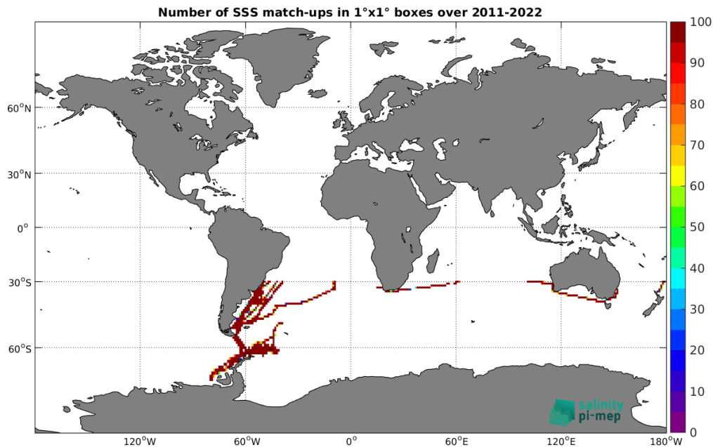
Figure 5: Number of SSS match-ups between TSG (CSIC-UTM) SSS and the SMOS SSS L3 Southern Ocean v1 - 9-Day running mean (BEC) SSS product for the Global Ocean Pi-MEP region over 1°×1° boxes and for the full satellite product period.
