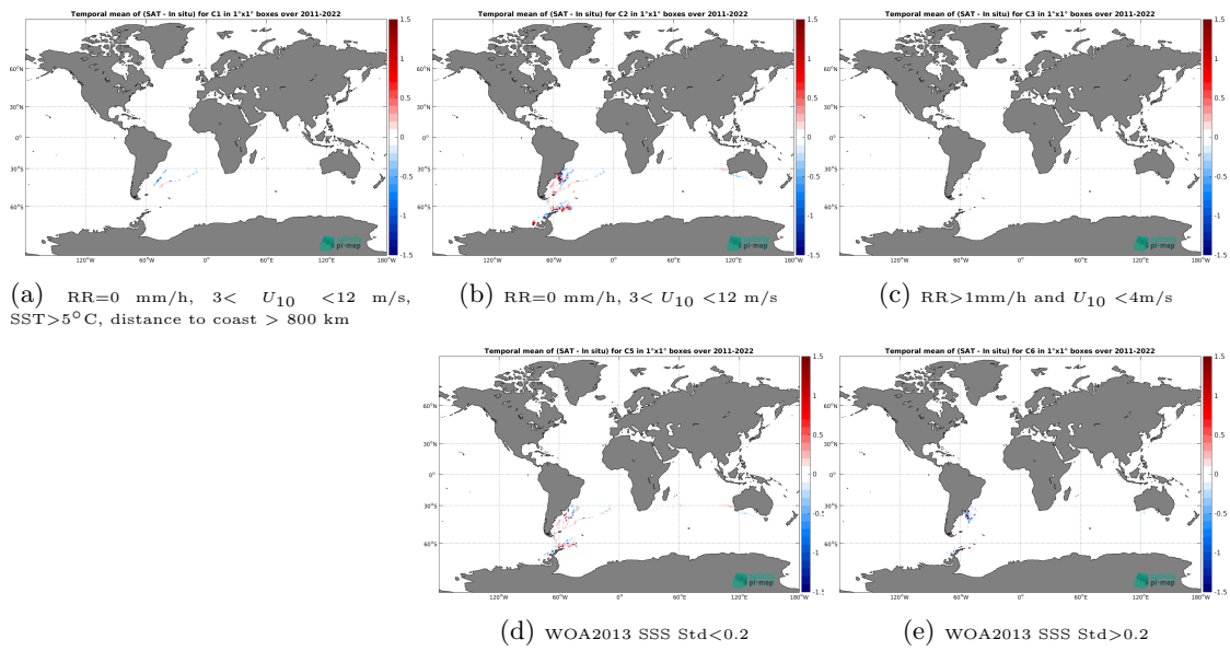
Figure 14: Temporal mean gridded over spatial boxes of size 1^\circ \times 1^\circ of \Delta\text{SSS} (SMOS SSS L3 Southern Ocean v1 - 9-Day running mean (BEC) - TSG (CSIC-UTM)) for 5 different subdatasets corresponding to:RR=0 mm/h, 3 < U_{10} < 12 m/s, SST > 5^\circ\text{C} , distance to coast > 800 km (a), RR=0 mm/h, 3 < U_{10} < 12 m/s (b), RR > 1 mm/h and U_{10} < 4 m/s (c), WOA2013 SSS Std < 0.2 (d), WOA2013 SSS Std > 0.2 (e).
