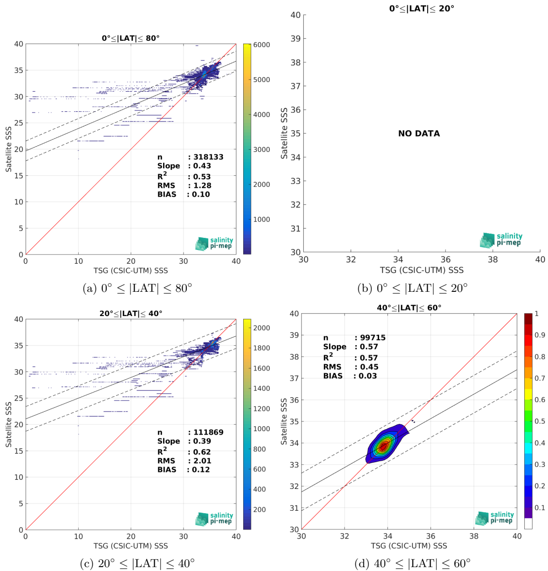
Figure 10: Contour maps of the concentration of SMOS SSS L3 Southern Ocean v1 - 9-Day running mean (BEC) SSS (y-axis) versus TSG (CSIC-UTM) SSS (x-axis) at match-up pairs for different latitude bands. For each plot, the red line shows x=y . The black thin and dashed lines indicate a linear fit through the data cloud and the \pm 95\% confidence levels, respectively. The number match-up pairs n , the slope and R^2 coefficient of the linear fit, the root mean square (RMS) and the mean bias between satellite and in situ data are indicated for each latitude band in each plots.
