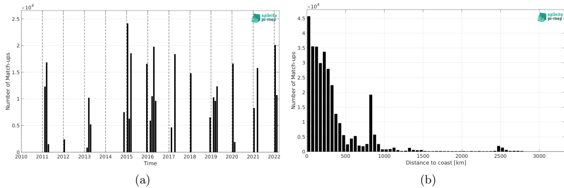
Figure 2: Number of match-ups between TSG (CSIC-UTM) and SMOS SSS L3 Southern Ocean v1 - 9-Day running mean (BEC) SSS as a function of time (a) and as function of the distance to coast (b) over the Global Ocean Pi-MEP region and for the full satellite product period.
