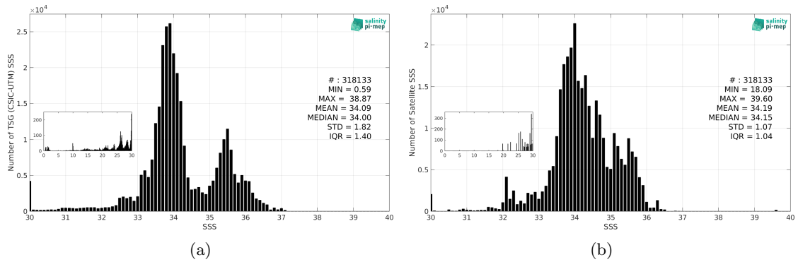
Figure 3: Histograms of SSS from TSG (CSIC-UTM) (a) and SMOS SSS L3 Southern Ocean v1 - 9-Day running mean (BEC) (b) considering all match-up pairs per bins of 0.1 over the Global Ocean Pi-MEP region and for the full satellite product period.
