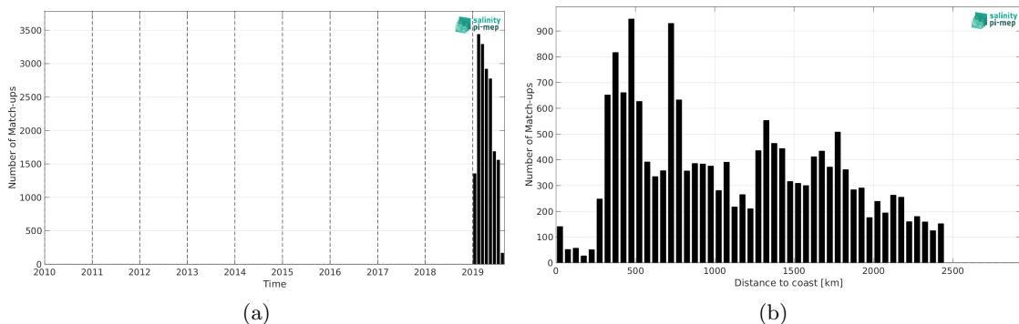
Figure 2: Number of match-ups between Saildrone and SMOS SSS L3 Southern Ocean v1 - 9-Day running mean (BEC) SSS as a function of time (a) and as function of the distance to coast (b) over the Global Ocean Pi-MEP region and for the full satellite product period.
