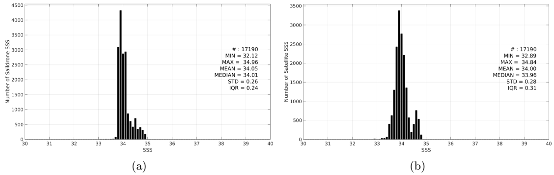
Figure 3: Histograms of SSS from Saildrone (a) and SMOS SSS L3 Southern Ocean v1 - 9-Day running mean (BEC) (b) considering all match-up pairs per bins of 0.1 over the Global Ocean Pi-MEP region and for the full satellite product period.
