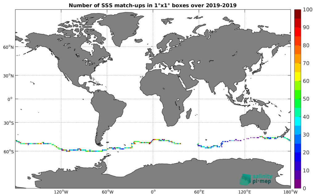
Figure 5: Number of SSS match-ups between Saildrone SSS and the SMOS SSS L3 Southern Ocean v1 - 9-Day running mean (BEC) SSS product for the Global Ocean Pi-MEP region over 1^\circ \times 1^\circ boxes and for the full satellite product period.
