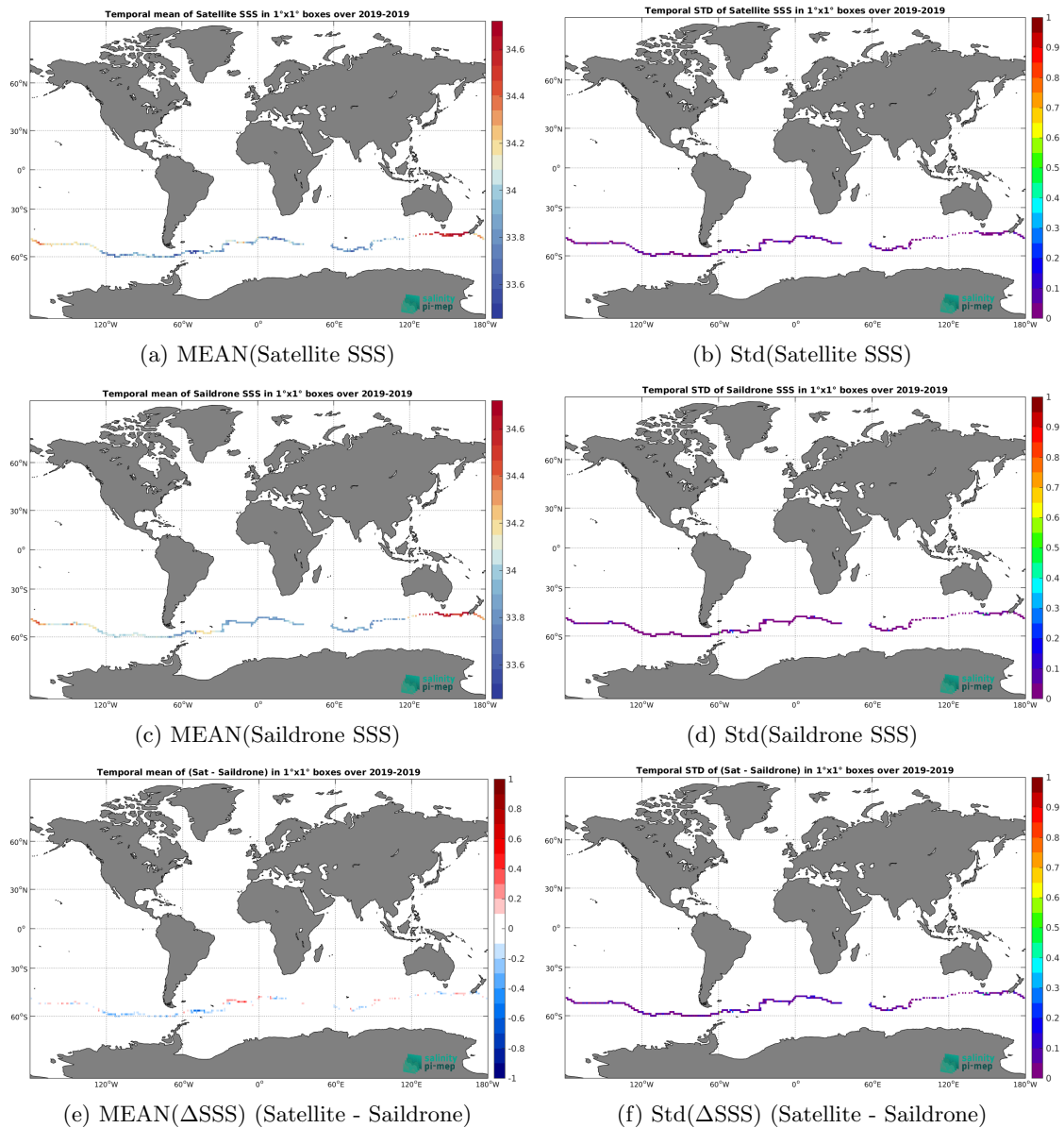
Figure 7: Temporal mean (left) and Std (right) of SSS from SMOS SSS L3 Southern Ocean v1 - 9-Day running mean (BEC) (top), Saildrone (middle), and of \Delta SSS (Satellite - Saildrone). Only match-up pairs are used to generate these maps.
