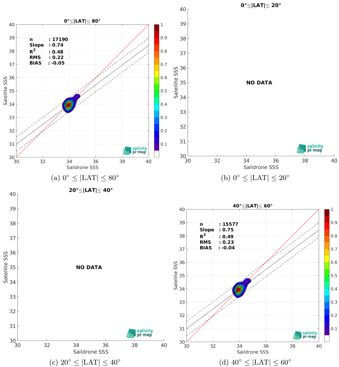
Figure 10: Contour maps of the concentration of SMOS SSS L3 Southern Ocean v1 - 9-Day running mean (BEC) SSS (y-axis) versus Saildrone SSS (x-axis) at match-up pairs for different latitude bands. For each plot, the red line shows x=y . The black thin and dashed lines indicate a linear fit through the data cloud and the \pm 95\% confidence levels, respectively. The number match-up pairs n , the slope and R^2 coefficient of the linear fit, the root mean square (RMS) and the mean bias between satellite and in situ data are indicated for each latitude band in each plots.
