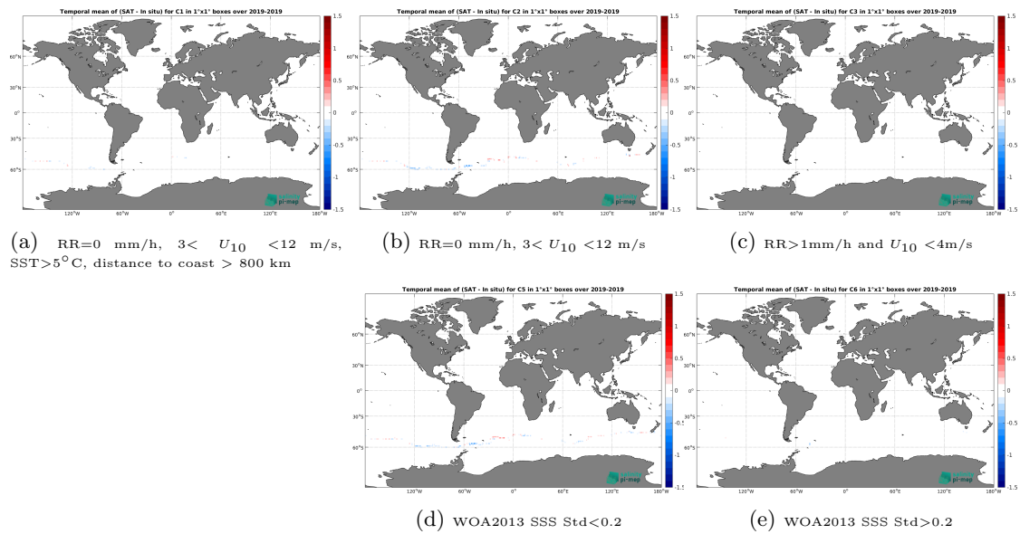
Figure 14: Temporal mean gridded over spatial boxes of size 1^\circ \times 1^\circ of \Delta SSS (SMOS SSS L3 Southern Ocean v1 - 9-Day running mean (BEC) - Saildrone) for 5 different subdatasets corresponding to:RR=0 mm/h, 3 < U_{10} < 12 m/s, SST >5^\circ C, distance to coast > 800 km (a), RR=0 mm/h, 3 < U_{10} < 12 m/s (b), RR >1 mm/h and U_{10} < 4 m/s (c), WOA2013 SSS Std <0.2 (d), WOA2013 SSS Std >0.2 (e).
