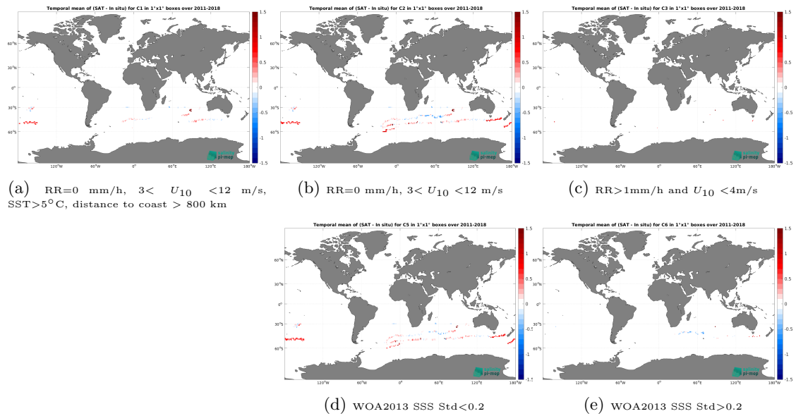
Figure 13: Temporal mean gridded over spatial boxes of size 1^\circ \times 1^\circ of \Delta SSS (SMOS SSS L3 Southern Ocean v1 - 9-Day running mean (BEC) - Surface drifters) for 5 different subdatasets corresponding to: RR=0 mm/h, 3 < U_{10} < 12 m/s, SST > 5^\circ\text{C} , distance to coast > 800 km (a), RR=0 mm/h, 3 < U_{10} < 12 m/s (b), RR > 1 mm/h and U_{10} < 4 m/s (c), WOA2013 SSS Std < 0.2 (d), WOA2013 SSS Std > 0.2 (e).
