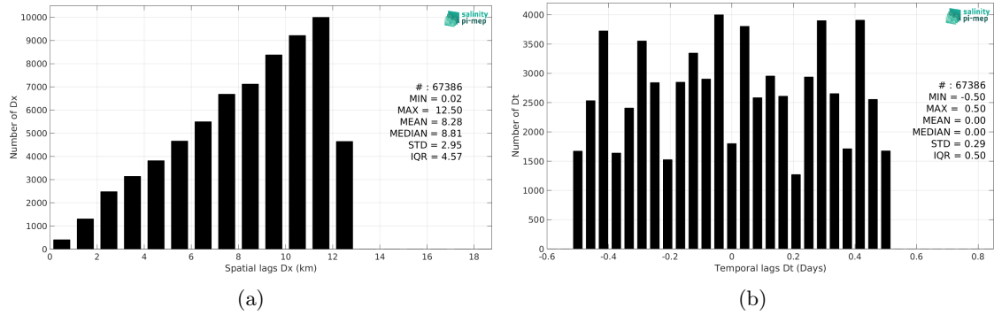
Figure 5: Histograms of the spatial (a) and temporal (b) lags between the location/time of the Surface drifters measurement and the date of the corresponding SMOS SSS L3 Southern Ocean v1 - 9-Day running mean (BEC) SSS pixel.
