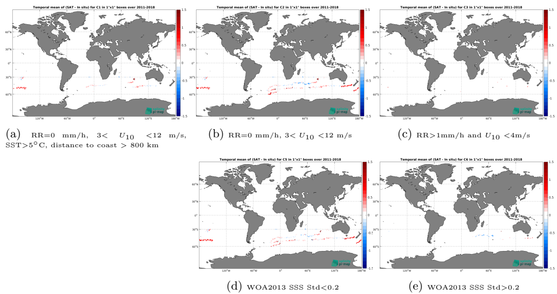
Figure 13: Temporal mean gridded over spatial boxes of size 1^\circ \times 1^\circ of \Delta\text{SSS} (SMOS SSS L3 Southern Ocean v1 - 9-Day running mean (BEC) - Surface drifters) for 5 different subdatasets corresponding to:RR=0 mm/h, 3 < U_{10} < 12 m/s, SST > 5^\circ\text{C} , distance to coast > 800 km (a), RR=0 mm/h, 3 < U_{10} < 12 m/s (b), RR > 1 mm/h and U_{10} < 4 m/s (c), WOA2013 SSS Std < 0.2 (d), WOA2013 SSS Std > 0.2 (e).
