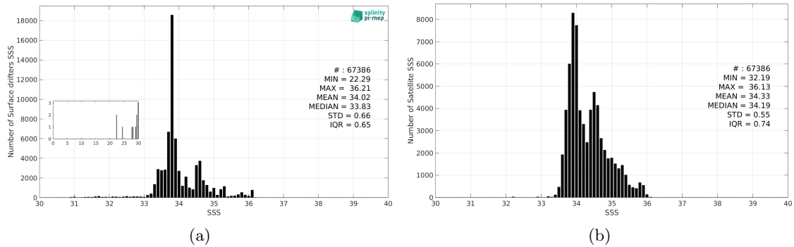
Figure 3: Histograms of SSS from Surface drifters (a) and SMOS SSS L3 Southern Ocean v1 - 9-Day running mean (BEC) (b) considering all match-up pairs per bins of 0.1 over the Global Ocean Pi-MEP region and for the full satellite product period.
