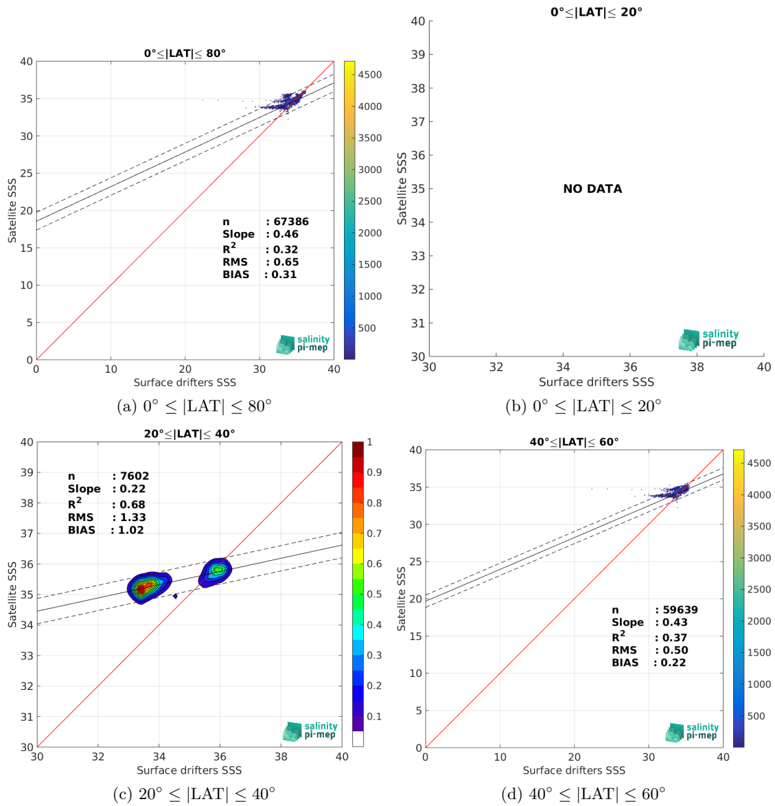
Figure 9: Contour maps of the concentration of SMOS SSS L3 Southern Ocean v1 - 9-Day running mean (BEC) SSS (y-axis) versus Surface drifters SSS (x-axis) at match-up pairs for different latitude bands. For each plot, the red line shows x=y . The black thin and dashed lines indicate a linear fit through the data cloud and the \pm 95\% confidence levels, respectively. The number match-up pairs n , the slope and R^2 coefficient of the linear fit, the root mean square (RMS) and the mean bias between satellite and in situ data are indicated for each latitude band in each plots.
