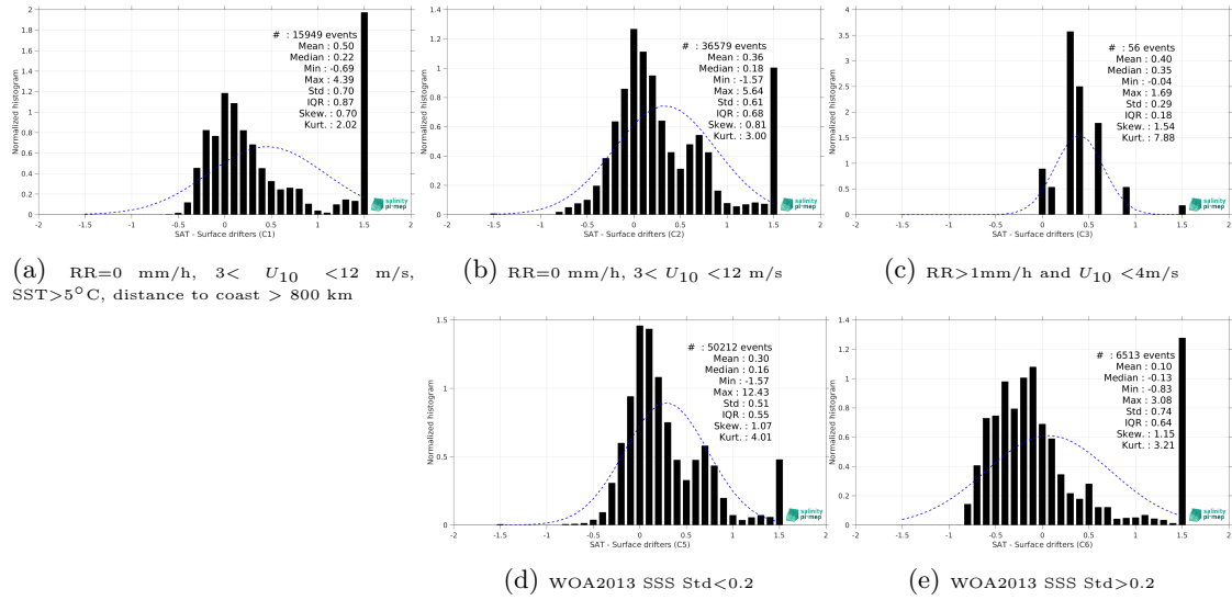
Figure 14: Normalized histogram of \Delta SSS (SMOS SSS L3 Southern Ocean v1 - 9-Day running mean (BEC) - Surface drifters) for 5 different subdatasets corresponding to: RR=0 mm/h, 3 < U_{10} < 12 m/s, SST>5°C, distance to coast > 800 km (a), RR=0 mm/h, 3 < U_{10} < 12 m/s (b), RR>1mm/h and U_{10} < 4 m/s (c), WOA2013 SSS Std<0.2 (d), WOA2013 SSS Std>0.2 (e).
