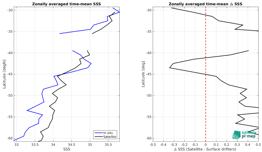
Figure 8: Left panel: Zonal mean SSS from SMOS SSS L3 Southern Ocean v1 - 9-Day running mean (BEC) satellite product (black) and from Surface drifters (blue). Right panel: Zonal mean of \Delta SSS (Satellite - Surface drifters) for all the collected Pi-MEP match-up pairs estimated over the full satellite product period.
