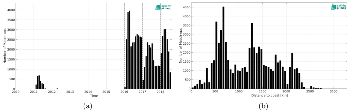
Figure 2: Number of match-ups between Surface drifters and SMOS SSS L3 Southern Ocean v1 - 9-Day running mean (BEC) SSS as a function of time (a) and as function of the distance to coast (b) over the Global Ocean Pi-MEP region and for the full satellite product period.
