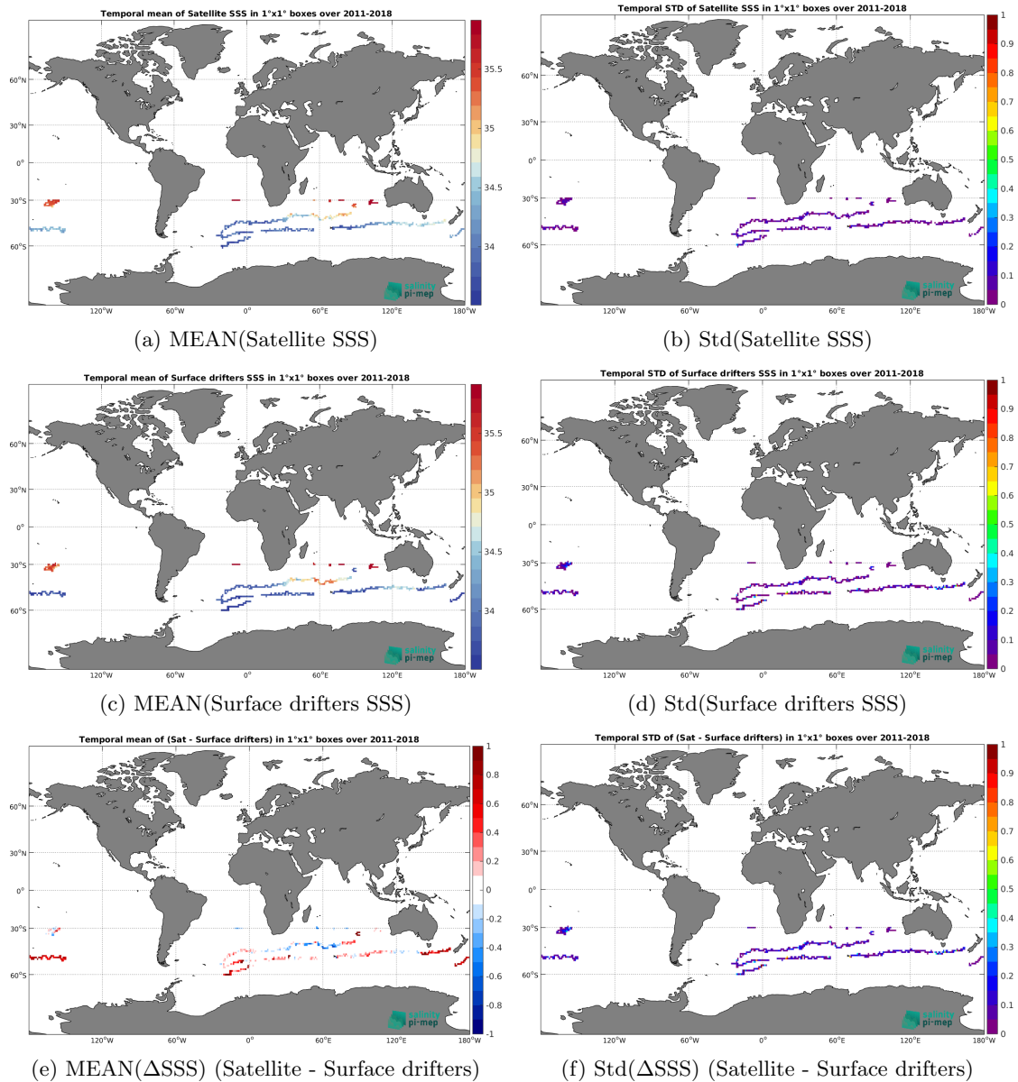
Figure 6: Temporal mean (left) and Std (right) of SSS from SMOS SSS L3 Southern Ocean v1 - 9-Day running mean (BEC) (top), Surface drifters (middle), and of \Delta SSS (Satellite - Surface drifters). Only match-up pairs are used to generate these maps.
