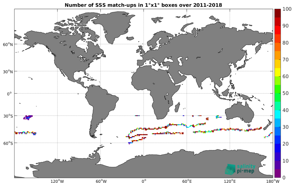
Figure 4: Number of SSS match-ups between Surface drifters SSS and the SMOS SSS L3 Southern Ocean v1 - 9-Day running mean (BEC) SSS product for the Global Ocean Pi-MEP region over 1^\circ \times 1^\circ boxes and for the full satellite product period.
