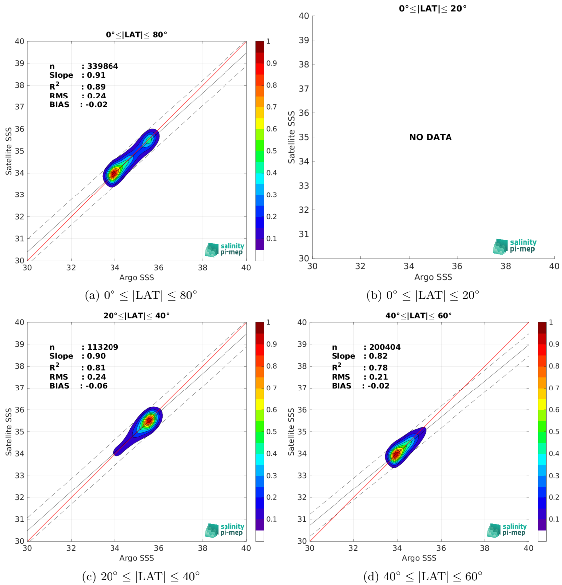
Figure 10: Contour maps of the concentration of SMOS SSS L3 Southern Ocean v1 - 9-Day running mean (BEC) SSS (y-axis) versus Argo SSS (x-axis) at match-up pairs for different latitude bands. For each plot, the red line shows x=y . The black thin and dashed lines indicate a linear fit through the data cloud and the \pm 95\% confidence levels, respectively. The number match-up pairs n , the slope and R^2 coefficient of the linear fit, the root mean square (RMS) and the mean bias between satellite and in situ data are indicated for each latitude band in each plots.
