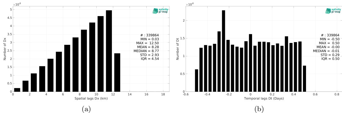
Figure 6: Histograms of the spatial (a) and temporal (b) lags between the location/time of the Argo measurement and the date of the corresponding SMOS SSS L3 Southern Ocean v1 - 9-Day running mean (BEC) SSS pixel.
