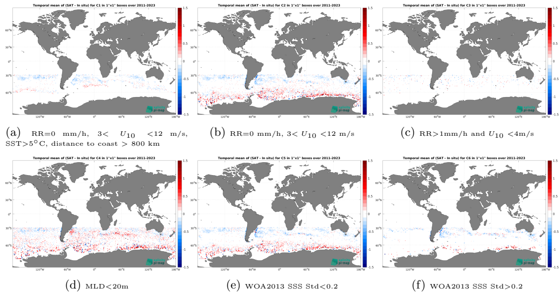
Figure 14: Temporal mean gridded over spatial boxes of size 1^\circ \times 1^\circ of \Delta SSS (SMOS SSS L3 Southern Ocean v1 - 9-Day running mean (BEC) - Argo) for 6 different subdatasets corresponding to:RR=0 mm/h, 3 < U_{10} < 12 m/s, SST>5°C, distance to coast > 800 km (a), RR=0 mm/h, 3 < U_{10} < 12 m/s (b), RR>1mm/h and U_{10} < 4 m/s (c),MLD<20m (d),WOA2013 SSS Std<0.2 (e),WOA2013 SSS Std>0.2 (f).
