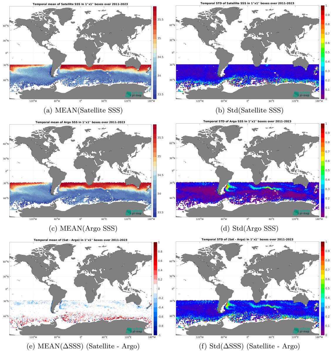
Figure 7: Temporal mean (left) and Std (right) of SSS from SMOS SSS L3 Southern Ocean v1 - 9-Day running mean (BEC) (top), Argo (middle), and of \Delta SSS (Satellite - Argo). Only match-up pairs are used to generate these maps.
