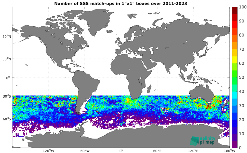
Figure 5: Number of SSS match-ups between Argo SSS and the SMOS SSS L3 Southern Ocean v1 - 9-Day running mean (BEC) SSS product for the Global Ocean Pi-MEP region over 1^\circ \times 1^\circ boxes and for the full satellite product period.
