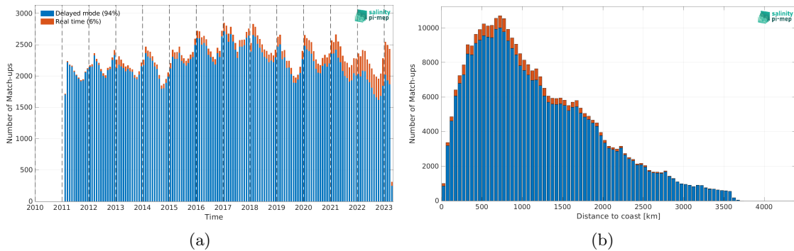
Figure 2: Number of match-ups between Argo and SMOS SSS L3 Southern Ocean v1 - 9-Day running mean (BEC) SSS as a function of time (a) and as function of the distance to coast (b) over the Global Ocean Pi-MEP region and for the full satellite product period.
