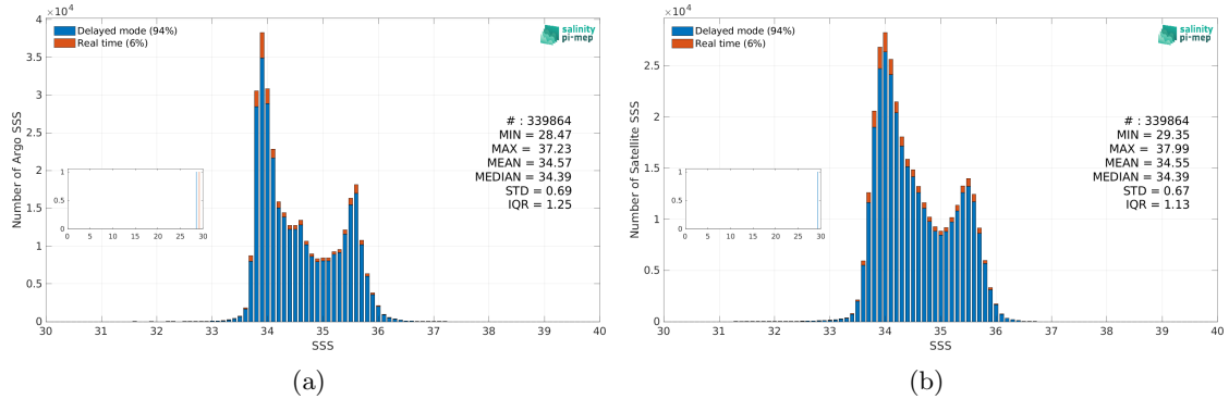
Figure 3: Histograms of SSS from Argo (a) and SMOS SSS L3 Southern Ocean v1 - 9-Day running mean (BEC) (b) considering all match-up pairs per bins of 0.1 over the Global Ocean Pi-MEP region and for the full satellite product period.
