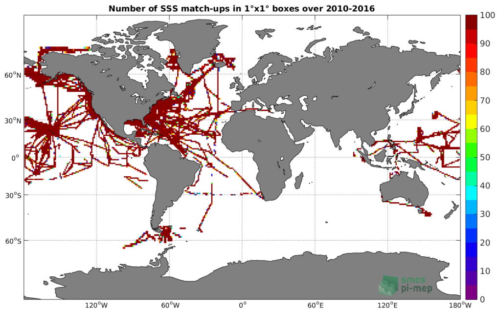
Figure 4: Number of SSS match-ups between TSG-SAMOS SSS and the SMOS-L3-BEC-OA-V1-9DAYS-0.25DEG SSS product for the Global Ocean Pi-MEP region over 1°x1° boxes and for the full satellite product period.
