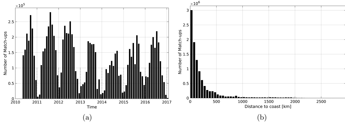
Figure 1: Number of match-ups between TSG-SAMOS and SMOS-L3-BEC-OA-V1-9DAYS-0.25DEG SSS as a function of time (a) and as function of the distance to coast (b) over the Global Ocean Pi-MEP region and for the full satellite product period.
