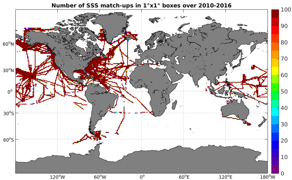
Figure 4: Number of SSS match-ups between TSG-SAMOS SSS and the SMOS-L3-BEC-OA-V1-9DAYS-0.25DEG SSS product for the Global Ocean Pi-MEP region over 1^\circ \times 1^\circ boxes and for the full satellite product period.
