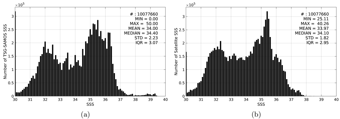
Figure 2: Histograms of SSS from TSG-SAMOS (a) and SMOS-L3-BEC-OA-V1-9DAYS-0.25DEG (b) considering all match-up pairs per bins of 0.1 over the Global Ocean Pi-MEP region and for the full satellite product period.
