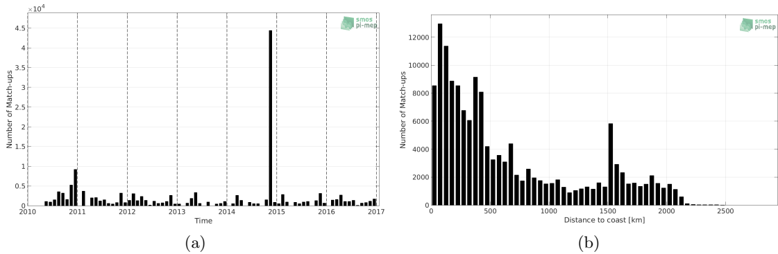
Figure 1: Number of match-ups between TSG-POLARSTERN and SMOS-L3-BEC-OA-V1-9DAYS-0.25DEG SSS as a function of time (a) and as function of the distance to coast (b) over the Global Ocean Pi-MEP region and for the full satellite product period.
