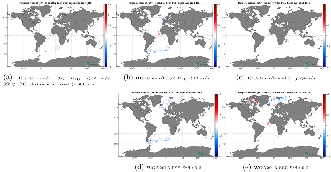
Figure 12: Temporal mean gridded over spatial boxes of size 1^\circ \times 1^\circ of \Delta SSS (SMOS-L3-BEC-OA-V1-9DAYS-0.25DEG - TSG-POLARSTERN) for 5 different subdatasets corresponding to:RR=0 mm/h, 3 < U_{10} < 12 m/s, SST > 5^\circ\text{C} , distance to coast > 800 km (a), RR=0 mm/h, 3 < U_{10} < 12 m/s (b), RR > 1 mm/h and U_{10} < 4 m/s (c), WOA2013 SSS Std < 0.2 (d), WOA2013 SSS Std > 0.2 (e).
