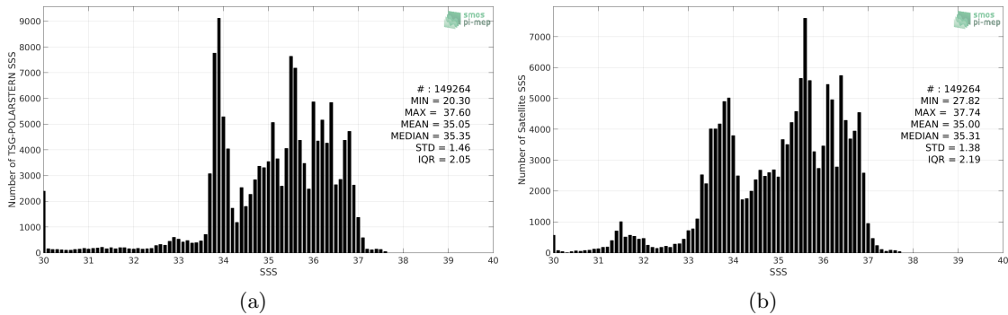
Figure 2: Histograms of SSS from TSG-POLARSTERN (a) and SMOS-L3-BEC-OA-V1-9DAYS-0.25DEG (b) considering all match-up pairs per bins of 0.1 over the Global Ocean Pi-MEP region and for the full satellite product period.
