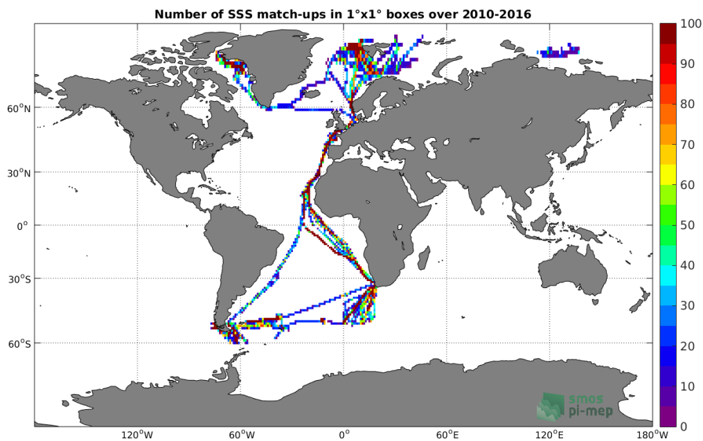
Figure 4: Number of SSS match-ups between TSG-POLARSTERN SSS and the SMOS-L3-BEC-OA-V1-9DAYS-0.25DEG SSS product for the Global Ocean Pi-MEP region over 1^\circ \times 1^\circ boxes and for the full satellite product period.
