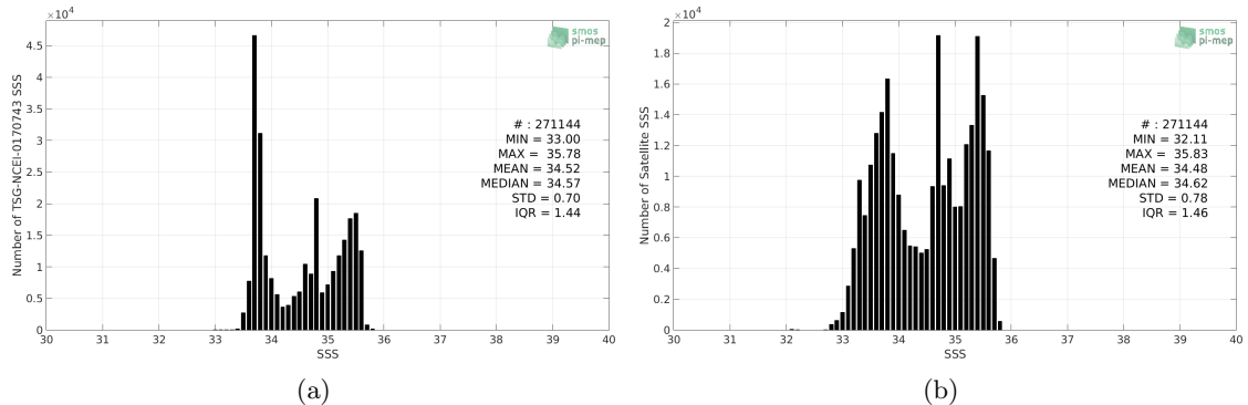
Figure 2: Histograms of SSS from TSG-NCEI-0170743 (a) and SMOS-L3-BEC-OA-V1-9DAYS-0.25DEG (b) considering all match-up pairs per bins of 0.1 over the Global Ocean Pi-MEP region and for the full satellite product period.
