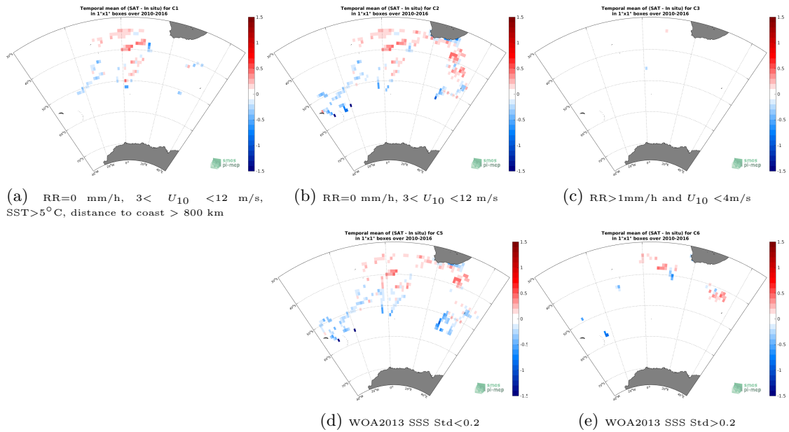
Figure 12: Temporal mean gridded over spatial boxes of size 1^\circ \times 1^\circ of \Delta SSS (SMOS-L3-BEC-OA-V1-9DAYS-0.25DEG - TSG-NCEI-0170743) for 5 different subdatasets corresponding to:RR=0 mm/h, 3 < U_{10} < 12 m/s, SST >5^\circ C, distance to coast > 800 km (a), RR=0 mm/h, 3 < U_{10} < 12 m/s (b), RR >1 mm/h and U_{10} < 4 m/s (c), WOA2013 SSS Std <0.2 (d), WOA2013 SSS Std >0.2 (e).
