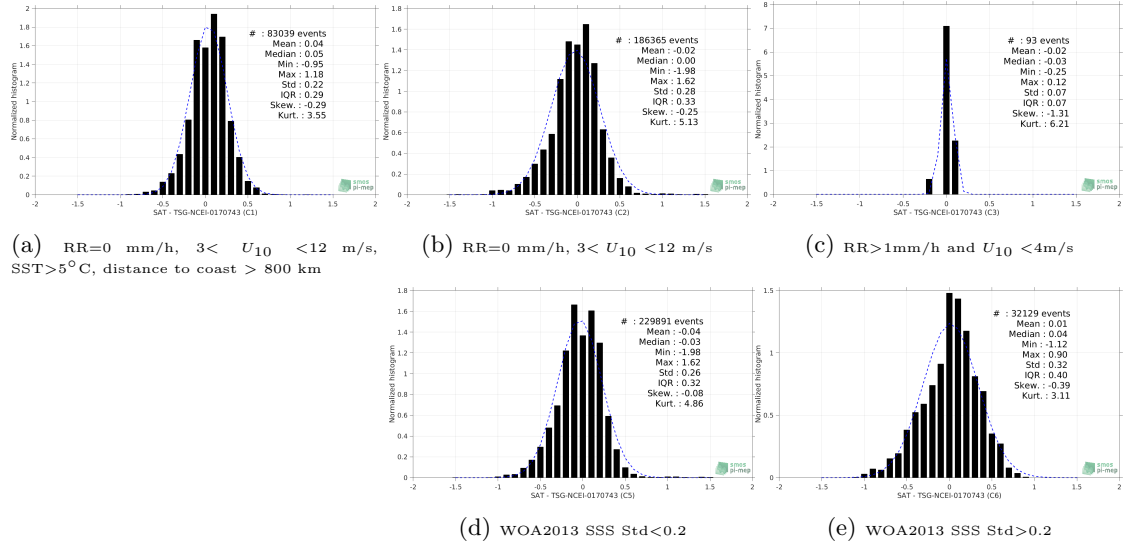
Figure 13: Normalized histogram of \Delta SSS (SMOS-L3-BEC-OA-V1-9DAYS-0.25DEG - TSG-NCEI-0170743) for 5 different subdatasets corresponding to: RR=0 mm/h, 3 < U_{10} < 12 m/s, SST>5°C, distance to coast > 800 km (a), RR=0 mm/h, 3 < U_{10} < 12 m/s (b), RR>1mm/h and U_{10} < 4 m/s (c), WOA2013 SSS Std<0.2 (d), WOA2013 SSS Std>0.2 (e).
