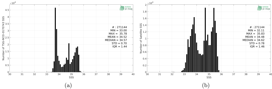
Figure 2: Histograms of SSS from TSG-NCEI-0170743 (a) and SMOS-L3-BEC-OA-V1-9DAYS-0.25DEG (b) considering all match-up pairs per bins of 0.1 over the Global Ocean Pi-MEP region and for the full satellite product period.
