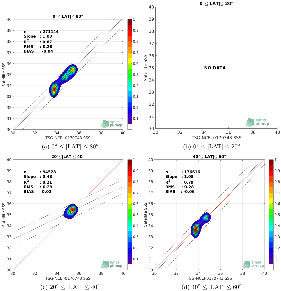
Figure 9: Contour maps of the concentration of SMOS-L3-BEC-OA-V1-9DAYS-0.25DEG SSS (y-axis) versus TSG-NCEI-0170743 SSS (x-axis) at match-up pairs for different latitude bands. For each plot, the red line shows x=y . The black thin and dashed lines indicate a linear fit through the data cloud and the \pm 95\% confidence levels, respectively. The number match-up pairs n , the slope and R^2 coefficient of the linear fit, the root mean square (RMS) and the mean bias between satellite and in situ data are indicated for each latitude band in each plots.
