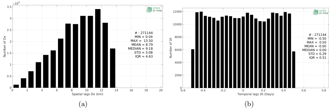
Figure 5: Histograms of the spatial (a) and temporal (b) lags between the time of the TSG-NCEI-0170743 measurements and the date of the corresponding SMOS-L3-BEC-OA-V1-9DAYS-0.25DEG SSS product.
