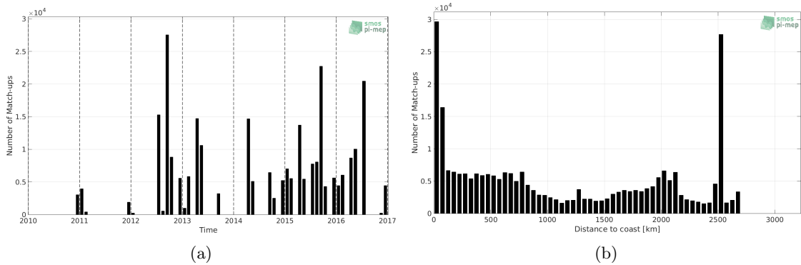
Figure 1: Number of match-ups between TSG-NCEI-0170743 and SMOS-L3-BEC-OA-V1-9DAYS-0.25DEG SSS as a function of time (a) and as function of the distance to coast (b) over the Global Ocean Pi-MEP region and for the full satellite product period.
