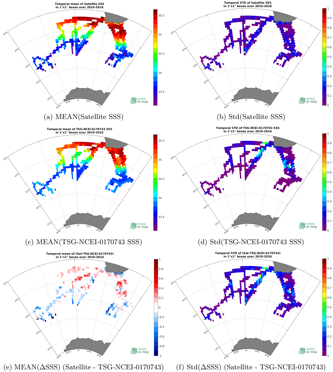
Figure 6: Temporal mean (left) and Std (right) of SSS from SMOS-L3-BEC-OA-V1-9DAYS-0.25DEG (top), TSG-NCEI-0170743 (middle), and of \Delta SSS (Satellite - TSG-NCEI-0170743). Only match-up pairs are used to generate these maps.
