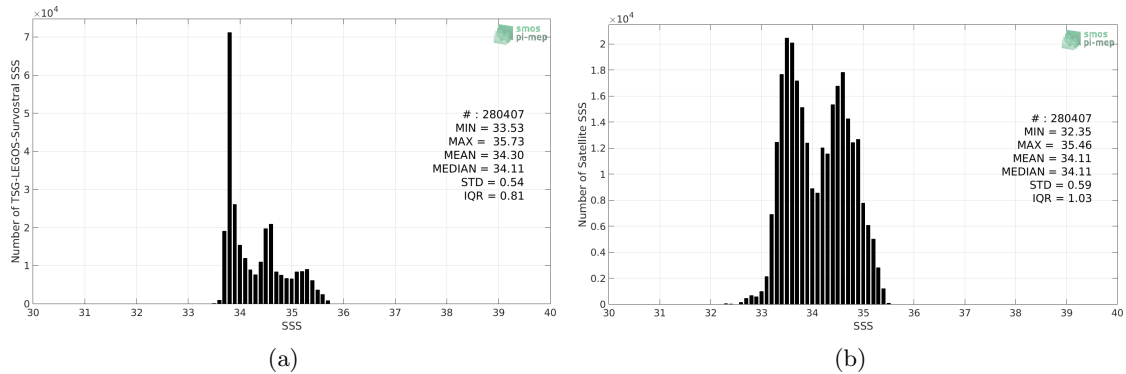
Figure 2: Histograms of SSS from TSG-LEGOS-Survostral (a) and SMOS-L3-BEC-OA-V1-9DAYS-0.25DEG (b) considering all match-up pairs per bins of 0.1 over the Global Ocean Pi-MEP region and for the full satellite product period.
