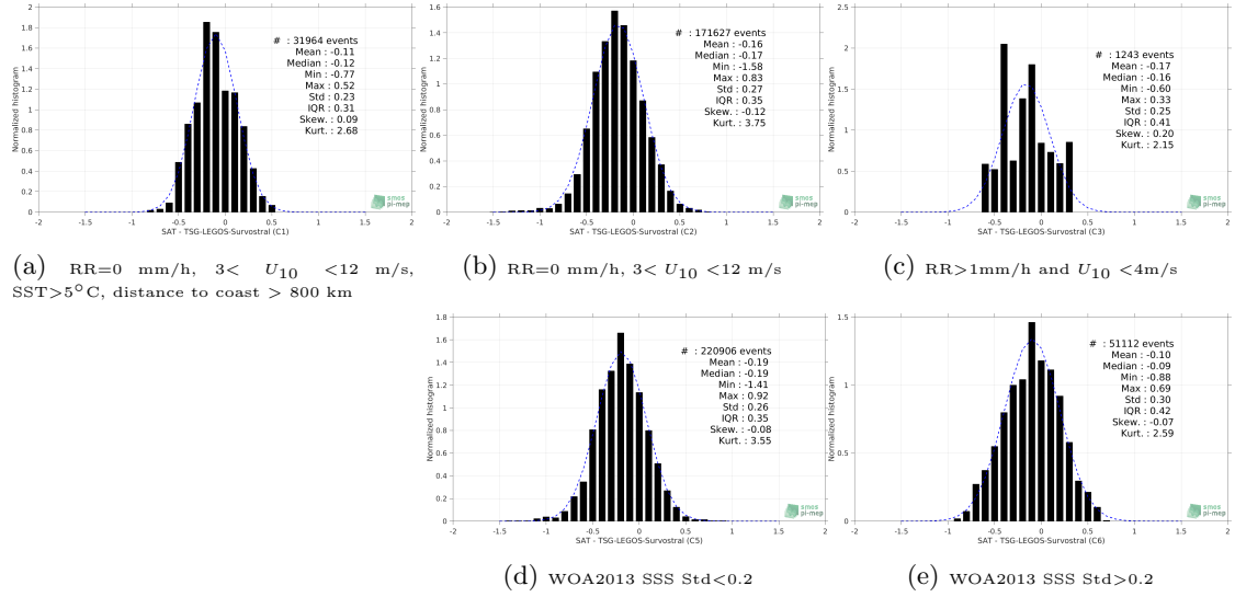
Figure 13: Normalized histogram of \Delta SSS (SMOS-L3-BEC-OA-V1-9DAYS-0.25DEG - TSG-LEGOS-Survostral) for 5 different subdatasets corresponding to: RR=0 mm/h, 3 < U_{10} < 12 m/s, SST>5°C, distance to coast > 800 km (a), RR=0 mm/h, 3 < U_{10} < 12 m/s (b), RR>1mm/h and U_{10} < 4 m/s (c), WOA2013 SSS Std<0.2 (d), WOA2013 SSS Std>0.2 (e).
