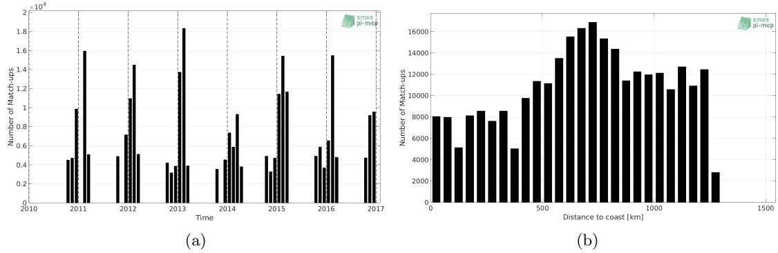
Figure 1: Number of match-ups between TSG-LEGOS-Survostral and SMOS-L3-BEC-OA-V1-9DAYS-0.25DEG SSS as a function of time (a) and as function of the distance to coast (b) over the Global Ocean Pi-MEP region and for the full satellite product period.
