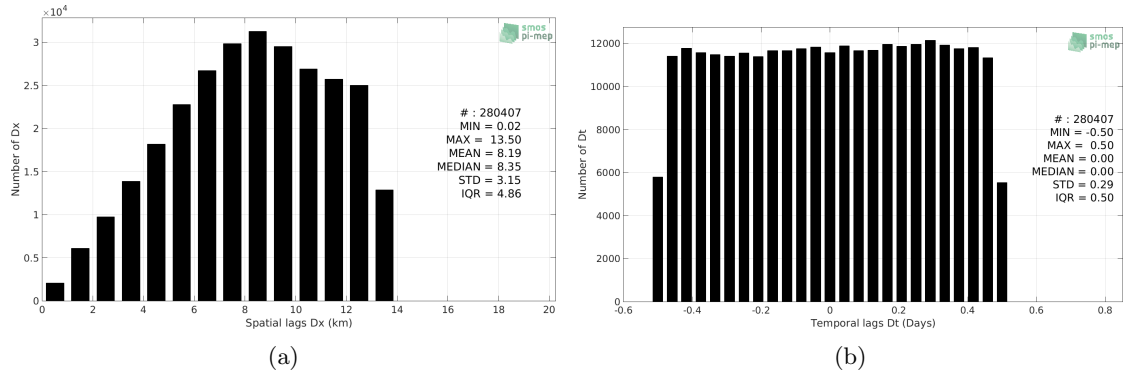
Figure 5: Histograms of the spatial (a) and temporal (b) lags between the time of the TSG-LEGOS-Survostral measurements and the date of the corresponding SMOS-L3-BEC-OA-V1-9DAYS-0.25DEG SSS product.
