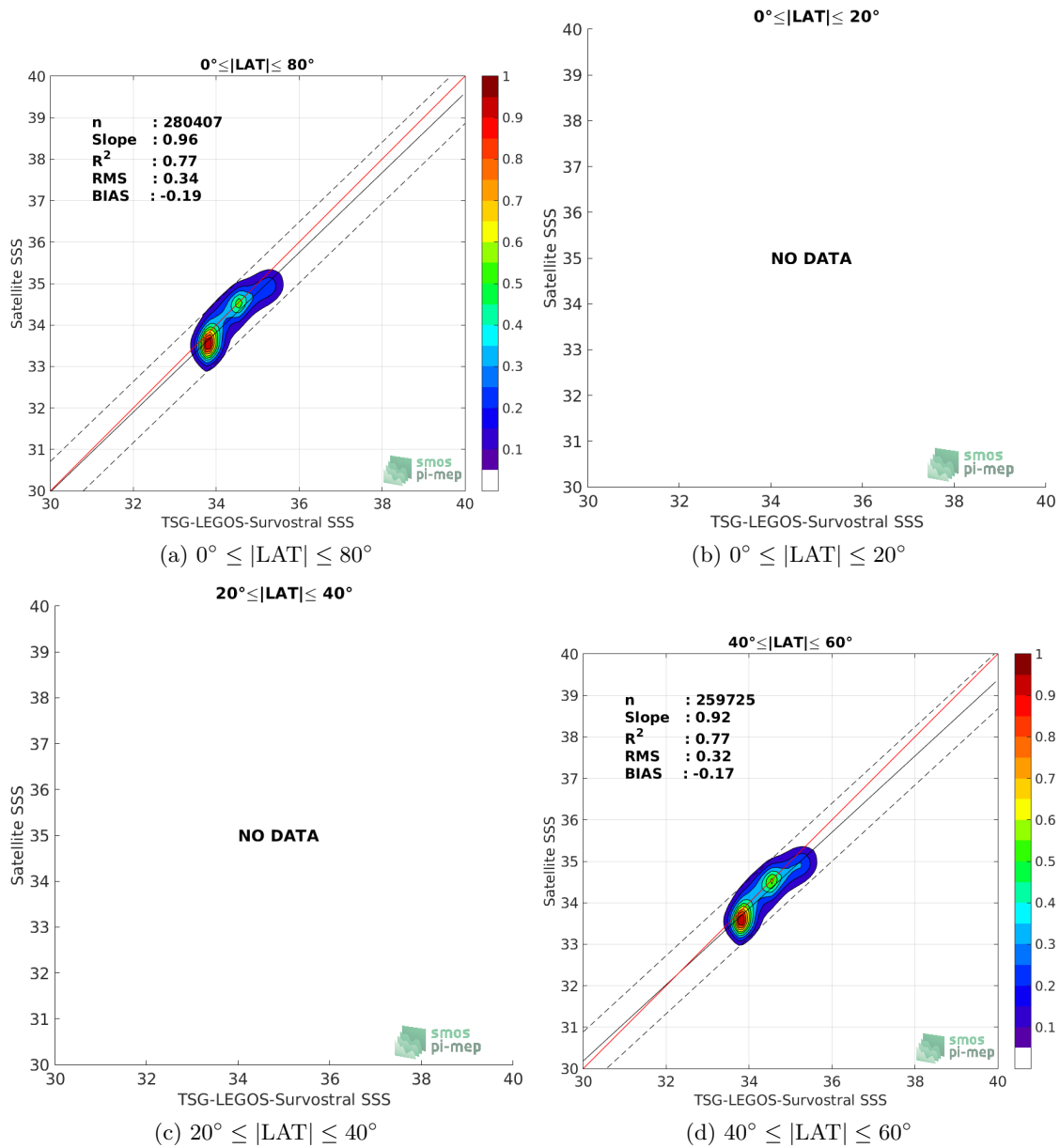
Figure 9: Contour maps of the concentration of SMOS-L3-BEC-OA-V1-9DAYS-0.25DEG SSS (y-axis) versus TSG-LEGOS-Survostral SSS (x-axis) at match-up pairs for different latitude bands. For each plot, the red line shows x=y . The black thin and dashed lines indicate a linear fit through the data cloud and the \pm 95\% confidence levels, respectively. The number match-up pairs n , the slope and R^2 coefficient of the linear fit, the root mean square (RMS) and the mean bias between satellite and in situ data are indicated for each latitude band in each plots.
