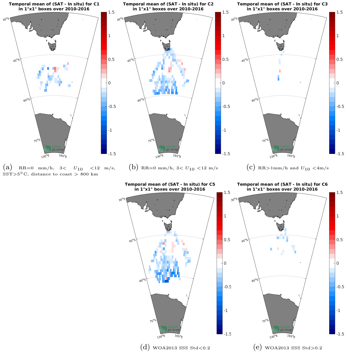
Figure 12: Temporal mean gridded over spatial boxes of size 1°x1° of \Delta SSS (SMOS-L3-BEC-OA-V1-9DAYS-0.25DEG - TSG-LEGOS-Survostral) for 5 different subdatasets corresponding to: RR=0 mm/h, 3 < U_{10} < 12 m/s, SST > 5°C, distance to coast > 800 km (a), RR=0 mm/h, 3 < U_{10} < 12 m/s (b), RR > 1mm/h and U_{10} < 4 m/s (c), WOA2013 SSS Std < 0.2 (d), WOA2013 SSS Std > 0.2 (e).
