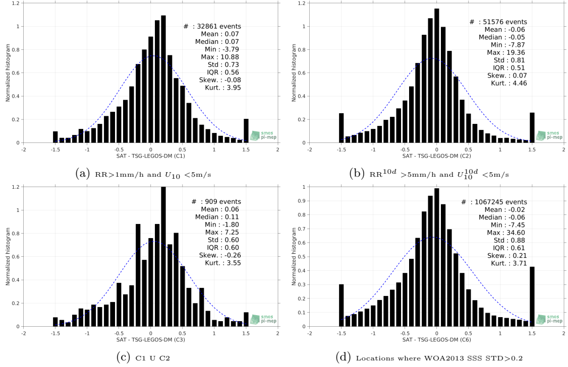
Figure 13: Normalized histogram of \Delta SSS (SMOS-L3-BEC-OA-V1-9DAYS-0.25DEG - TSG-LEGOS-DM) for 6 different subdatasets corresponding to: RR > 1\text{mm/h} and U_{10} < 5\text{m/s} (a), RR^{10d} > 5\text{mm/h} and U_{10}^{10d} < 5\text{m/s} (b), C1 U C2 (c), Locations where WOA2013 SSS STD > 0.2 (d).
