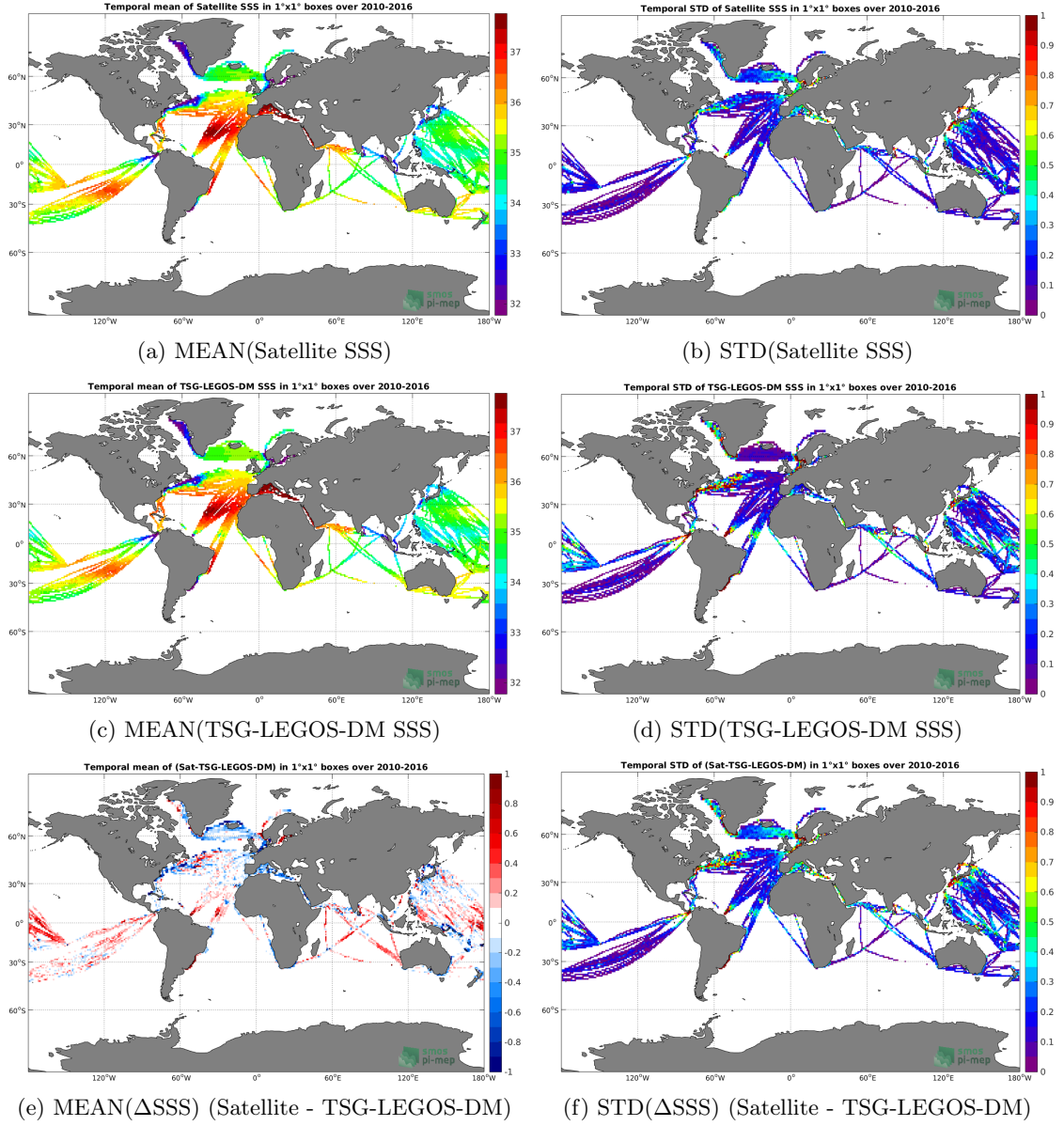
Figure 6: Temporal mean (left) and STD (right) of SSS from SMOS-L3-BEC-OA-V1-9DAYS-0.25DEG (top), TSG-LEGOS-DM (middle), and of \Delta SSS (Satellite - TSG-LEGOS-DM). Only match-up pairs are used to generate these maps.
