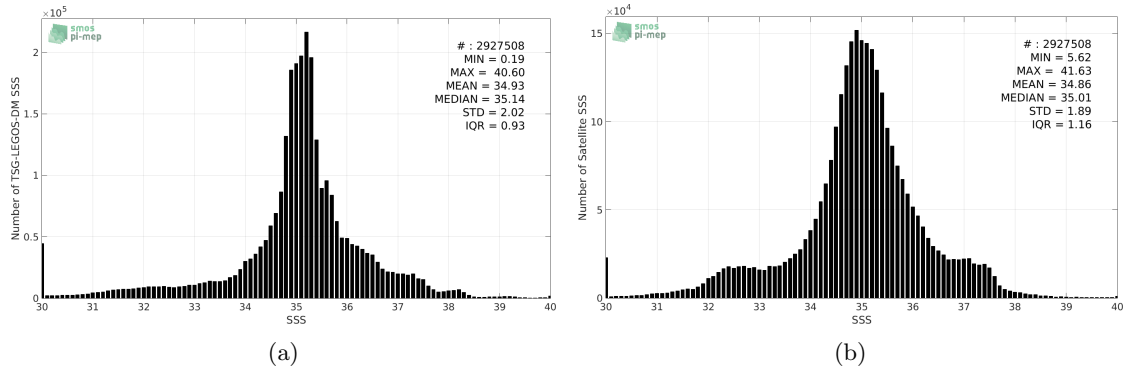
Figure 2: Histograms of SSS from TSG-LEGOS-DM (a) and SMOS-L3-BEC-OA-V1-9DAYS-0.25DEG (b) considering all match-up pairs per bins of 0.1 over the Global Ocean Pi-MEP region and for the full satellite product period.
