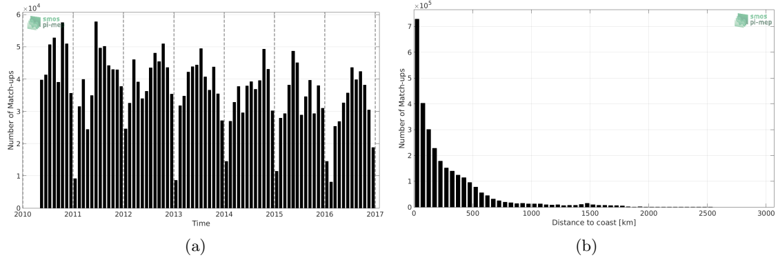
Figure 1: Number of match-ups between TSG-LEGOS-DM and SMOS-L3-BEC-OA-V1-9DAYS-0.25DEG SSS as a function of time (a) and as function of the distance to coast (b) over the Global Ocean Pi-MEP region and for the full satellite product period.
