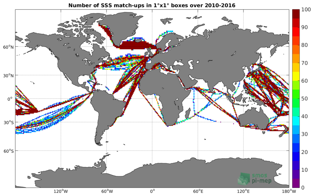
Figure 4: Number of SSS match-ups between TSG-LEGOS-DM SSS and the SMOS-L3-BEC-OA-V1-9DAYS-0.25DEG SSS product for the Global Ocean Pi-MEP region over 1°x1° boxes and for the full satellite product period.
