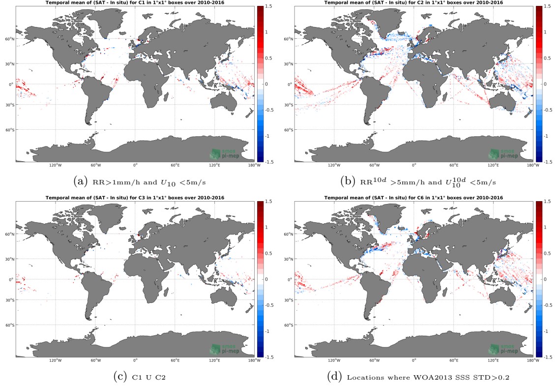
Figure 12: Temporal mean gridded over spatial boxes of size 1^\circ \times 1^\circ of \Delta SSS (SMOS-L3-BEC-OA-V1-9DAYS-0.25DEG - TSG-LEGOS-DM) for 4 different subdatasets corresponding to: RR > 1\text{mm/h} and U_{10} < 5\text{m/s} (a), RR^{10d} > 5\text{mm/h} and U_{10}^{10d} < 5\text{m/s} (b), C1 U C2 (c), Locations where WOA2013 SSS STD > 0.2 (d).
