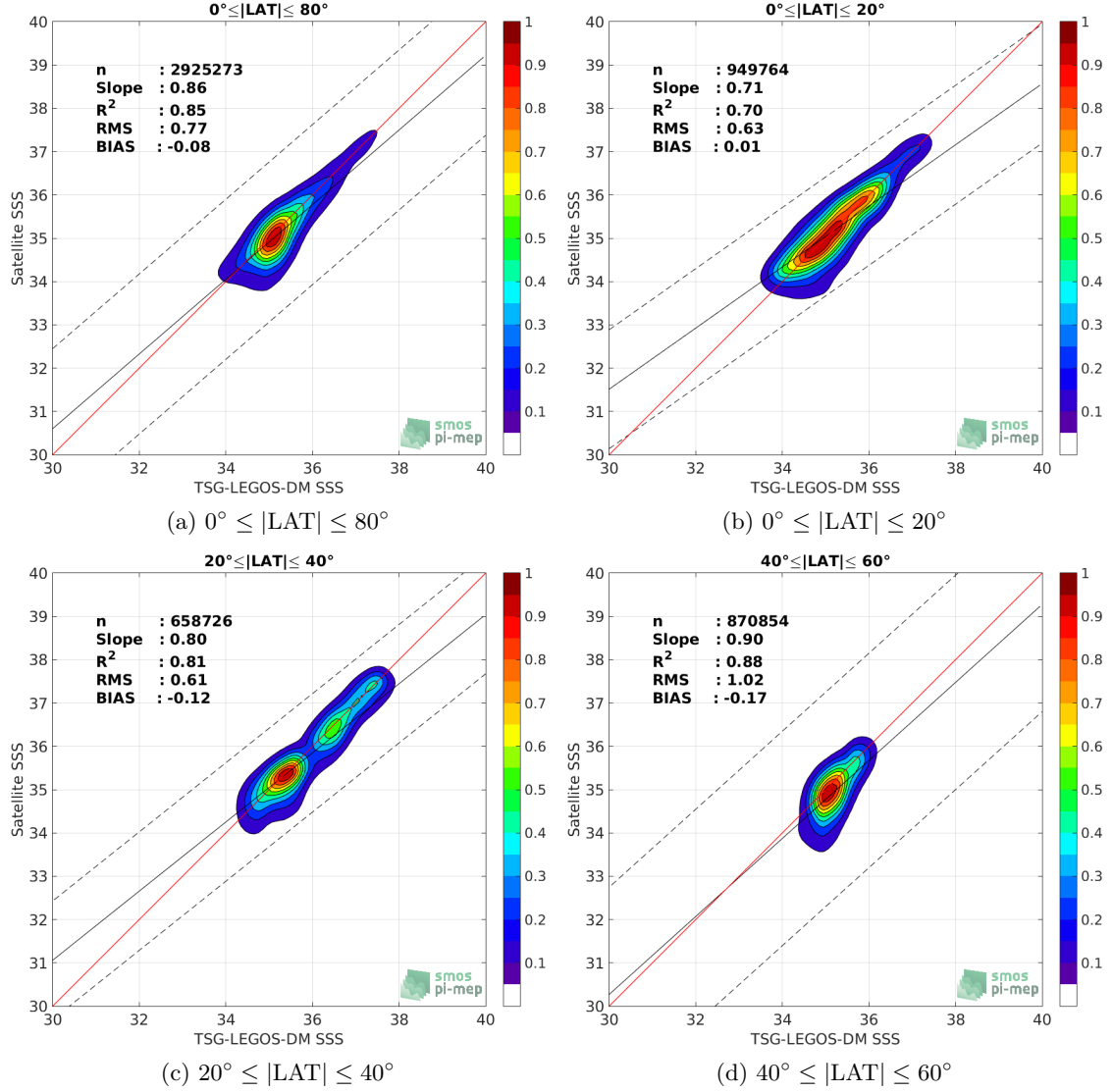
Figure 9: Contour maps of the concentration of SMOS-L3-BEC-OA-V1-9DAYS-0.25DEG SSS (y-axis) versus TSG-LEGOS-DM SSS (x-axis) at match-up pairs for different latitude bands. For each plot, the red line shows x=y . The black thin and dashed lines indicate a linear fit through the data cloud and the \pm 95\% confidence levels, respectively. The number match-up pairs n , the slope and R^2 coefficient of the linear fit, the root mean square (RMS) and the mean bias between satellite and in situ data are indicated for each latitude band in each plots.
