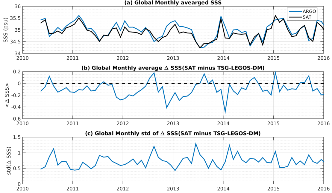
Figure 7: Time series of the monthly averaged mean SSS (top), mean \Delta SSS (Satellite - TSG-LEGOS-DM) and STD of \Delta SSS (Satellite - TSG-LEGOS-DM) over the Global Ocean Pi-MEP region considering all match-ups collected by the Pi-MEP platform.
