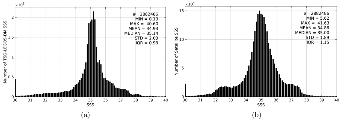
Figure 2: Histograms of SSS from TSG-LEGOS-DM (a) and SMOS-L3-BEC-OA-V1-9DAYS-0.25DEG (b) considering all match-up pairs per bins of 0.1 over the Global Ocean Pi-MEP region and for the full satellite product period.
