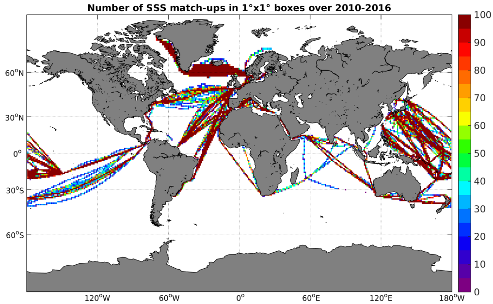
Figure 4: Number of SSS match-ups between TSG-LEGOS-DM SSS and the SMOS-L3-BEC-OA-V1-9DAYS-0.25DEG SSS product for the Global Ocean Pi-MEP region over 1°x1° boxes and for the full satellite product period.
