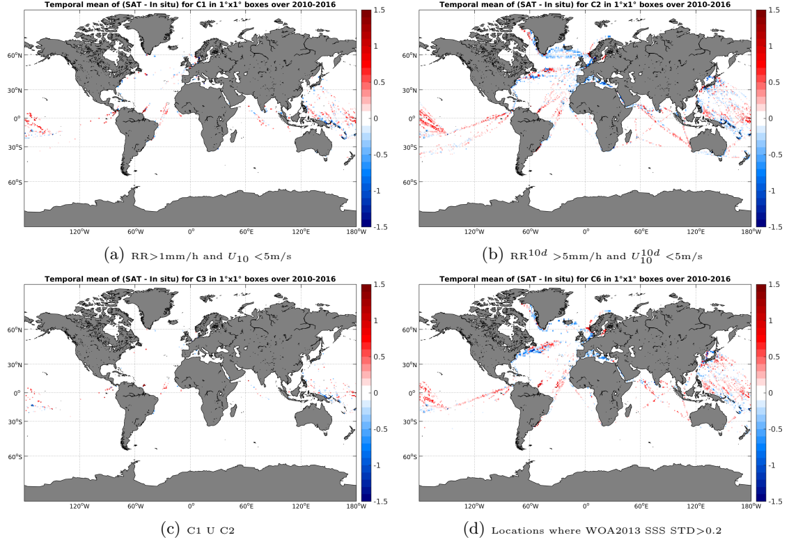
Figure 12: Temporal mean gridded over spatial boxes of size 1^\circ \times 1^\circ of \Delta SSS (SMOS-L3-BEC-OA-V1-9DAYS-0.25DEG - TSG-LEGOS-DM) for 4 different subdatasets corresponding to: RR > 1mm/h and U_{10} < 5\text{m/s} (a), RR^{10d} > 5\text{mm/h} and U_{10}^{10d} < 5\text{m/s} (b), C1 U C2 (c), Locations where WOA2013 SSS STD > 0.2 (d).
