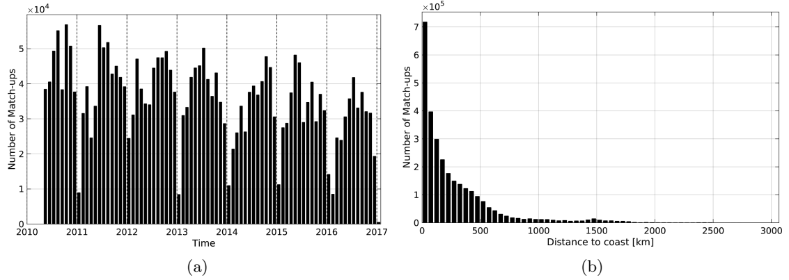
Figure 1: Number of match-ups between TSG-LEGOS-DM and SMOS-L3-BEC-OA-V1-9DAYS-0.25DEG SSS as a function of time (a) and as function of the distance to coast (b) over the Global Ocean Pi-MEP region and for the full satellite product period.
