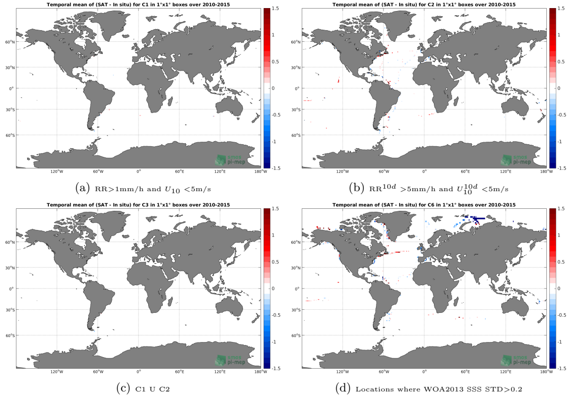
Figure 12: Temporal mean gridded over spatial boxes of size 1^\circ \times 1^\circ of \Delta SSS (SMOS-L3-BEC-OA-V1-9DAYS-0.25DEG - TSG-GOSUD-Sailing-ship) for 4 different subdatasets corresponding to: RR > 1\text{mm/h} and U_{10} < 5\text{m/s} (a), RR^{10d} > 5\text{mm/h} and U_{10}^{10d} < 5\text{m/s} (b), C1 U C2 (c), Locations where WOA2013 SSS STD > 0.2 (d).
