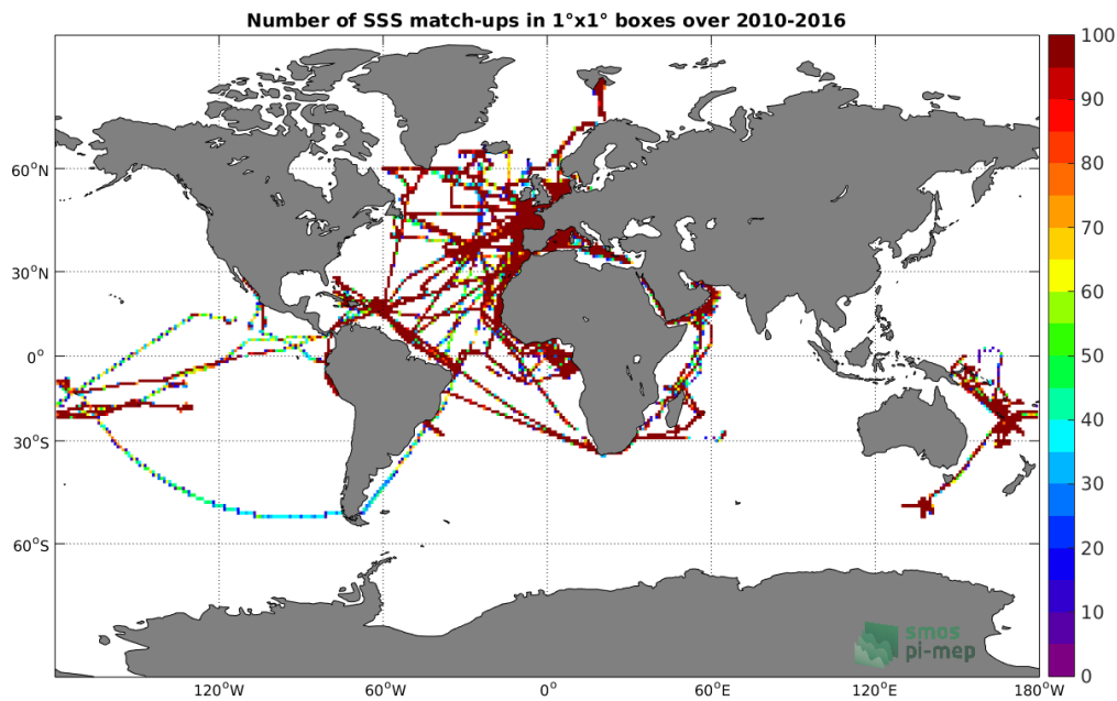
Figure 4: Number of SSS match-ups between TSG-GOSUD-Research-vessel SSS and the SMOS-L3-BEC-OA-V1-9DAYS-0.25DEG SSS product for the Global Ocean Pi-MEP region over 1°x1° boxes and for the full satellite product period.
