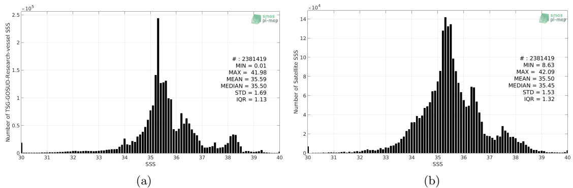
Figure 2: Histograms of SSS from TSG-GOSUD-Research-vessel (a) and SMOS-L3-BEC-OA-V1-9DAYS-0.25DEG (b) considering all match-up pairs per bins of 0.1 over the Global Ocean Pi-MEP region and for the full satellite product period.
