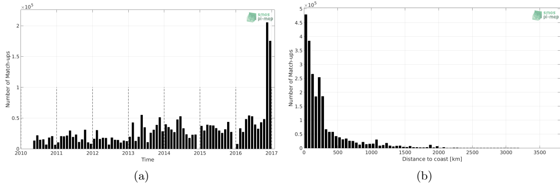
Figure 1: Number of match-ups between TSG-GOSUD-Research-vessel and SMOS-L3-BEC-OA-V1-9DAYS-0.25DEG SSS as a function of time (a) and as function of the distance to coast (b) over the Global Ocean Pi-MEP region and for the full satellite product period.
