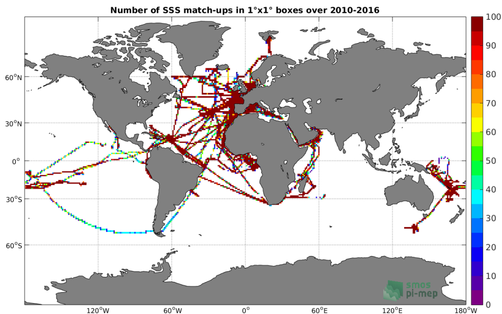
Figure 4: Number of SSS match-ups between TSG-GOSUD-Research-vessel SSS and the SMOS-L3-BEC-OA-V1-9DAYS-0.25DEG SSS product for the Global Ocean Pi-MEP region over 1^\circ \times 1^\circ boxes and for the full satellite product period.
