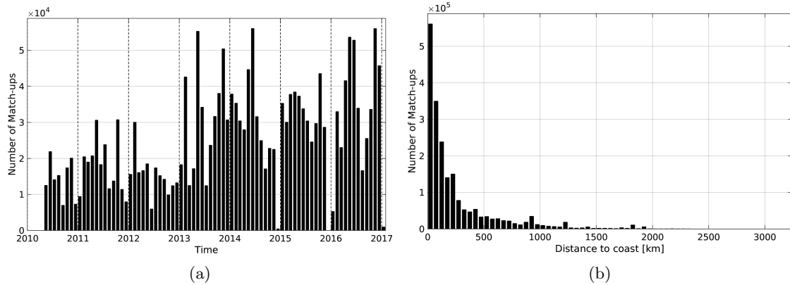
Figure 1: Number of match-ups between TSG-GOSUD-Research-vessel and SMOS-L3-BEC-OA-V1-9DAYS-0.25DEG SSS as a function of time (a) and as function of the distance to coast (b) over the Global Ocean Pi-MEP region and for the full satellite product period.
