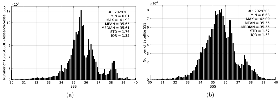
Figure 2: Histograms of SSS from TSG-GOSUD-Research-vessel (a) and SMOS-L3-BEC-OA-V1-9DAYS-0.25DEG (b) considering all match-up pairs per bins of 0.1 over the Global Ocean Pi-MEP region and for the full satellite product period.
