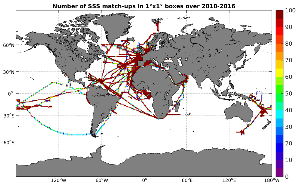
Figure 4: Number of SSS match-ups between TSG-GOSUD-Research-vessel SSS and the SMOS-L3-BEC-OA-V1-9DAYS-0.25DEG SSS product for the Global Ocean Pi-MEP region over 1^\circ \times 1^\circ boxes and for the full satellite product period.
