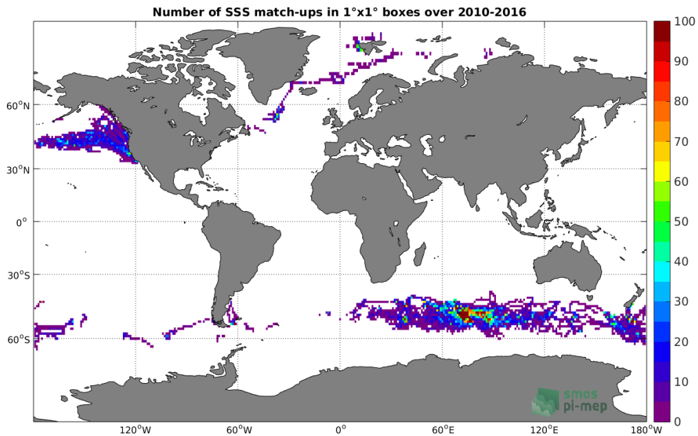
Figure 4: Number of SSS match-ups between Sea mammals SSS and the SMOS-L3-BEC-OA-V1-9DAYS-0.25DEG SSS product for the Global Ocean Pi-MEP region over 1^\circ \times 1^\circ boxes and for the full satellite product period.
