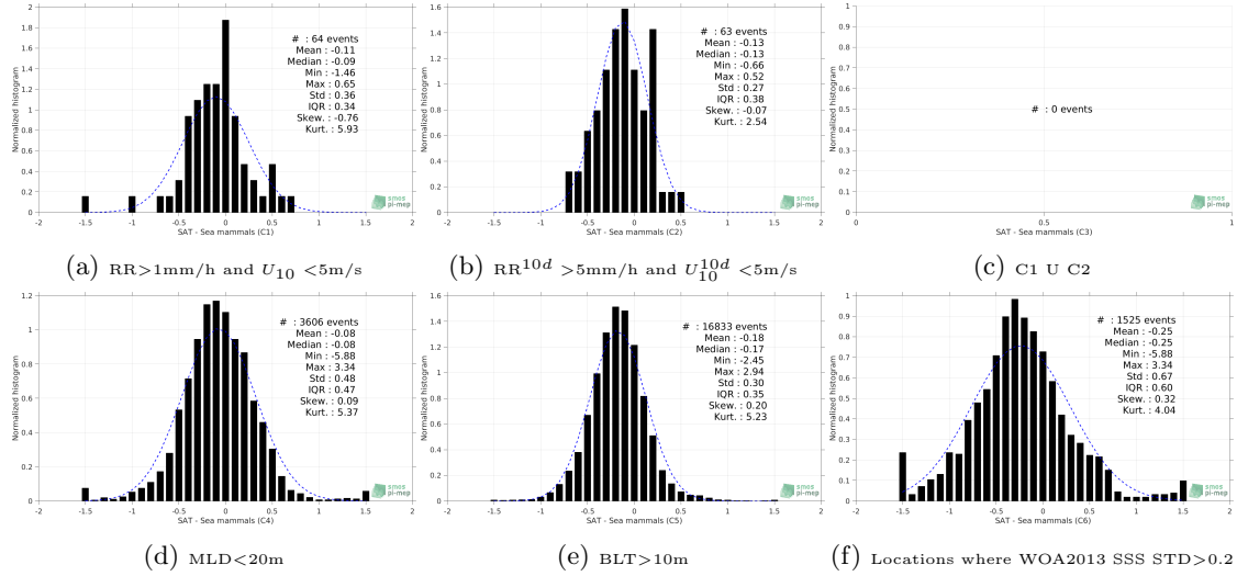
Figure 13: Normalized histogram of \Delta\text{SSS} (SMOS-L3-BEC-OA-V1-9DAYS-0.25DEG - Sea mammals) for 6 different subdatasets corresponding to: RR > 1\text{mm/h} and U_{10} < 5\text{m/s} (a), RR^{10d} > 5\text{mm/h} and U_{10}^{10d} < 5\text{m/s} (b), C1 U C2 (c), MLD < 20\text{m} (d), BLT > 10\text{m} (e), Locations where WOA2013 SSS STD > 0.2 (f).
