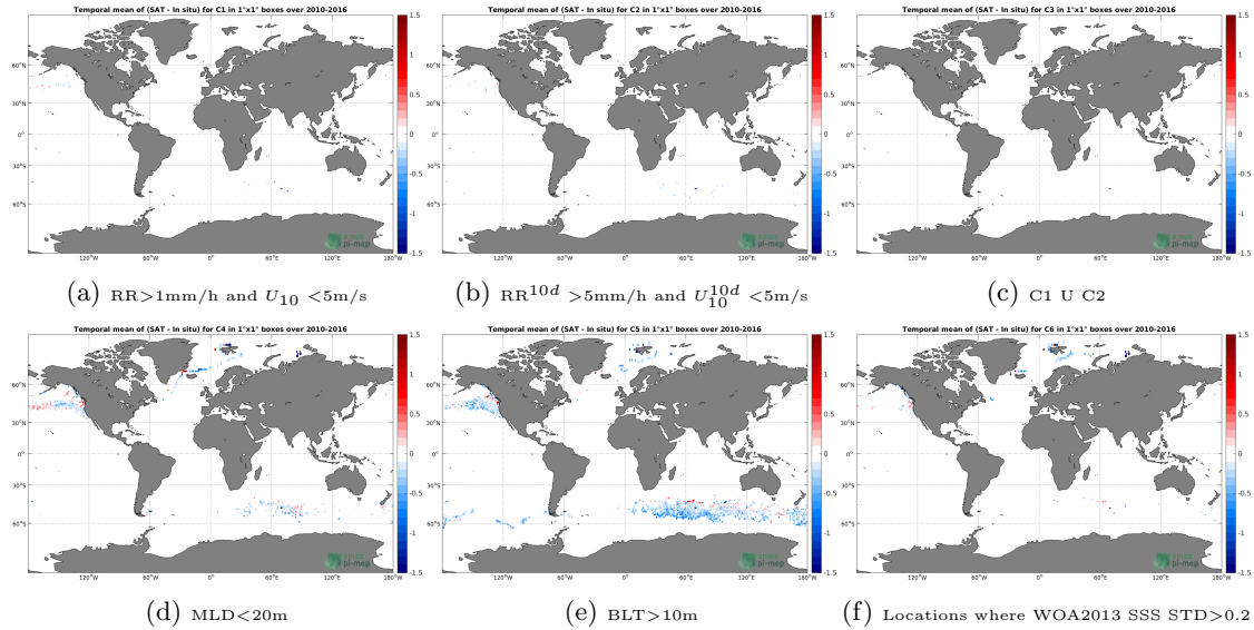
Figure 12: Temporal mean gridded over spatial boxes of size 1^\circ \times 1^\circ of \Delta\text{SSS} (SMOS-L3-BEC-OA-V1-9DAYS-0.25DEG - Sea mammals) for 6 different subdatasets corresponding to: RR > 1\text{mm/h} and U_{10} < 5\text{m/s} (a), RR^{10d} > 5\text{mm/h} and U_{10}^{10d} < 5\text{m/s} (b), C1 U C2 (c), MLD < 20\text{m} (d), BLT > 10\text{m} (e), Locations where WOA2013 SSS STD > 0.2 (f).
