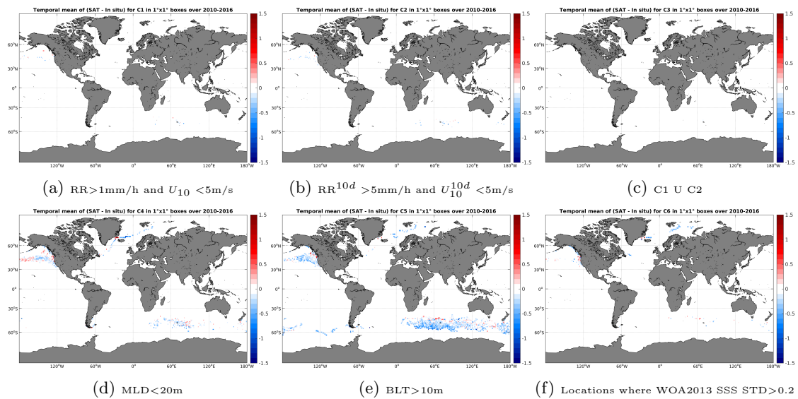
Figure 12: Temporal mean gridded over spatial boxes of size 1^\circ \times 1^\circ of \Delta SSS (SMOS-L3-BEC-OA-V1-9DAYS-0.25DEG - Sea mammals) for 6 different subdatasets corresponding to: RR > 1\text{mm/h} and U_{10} < 5\text{m/s} (a), RR^{10d} > 5\text{mm/h} and U_{10}^{10d} < 5\text{m/s} (b), C1 U C2 (c), MLD < 20\text{m} (d), BLT > 10\text{m} (e), Locations where WOA2013 SSS STD > 0.2 (f).
