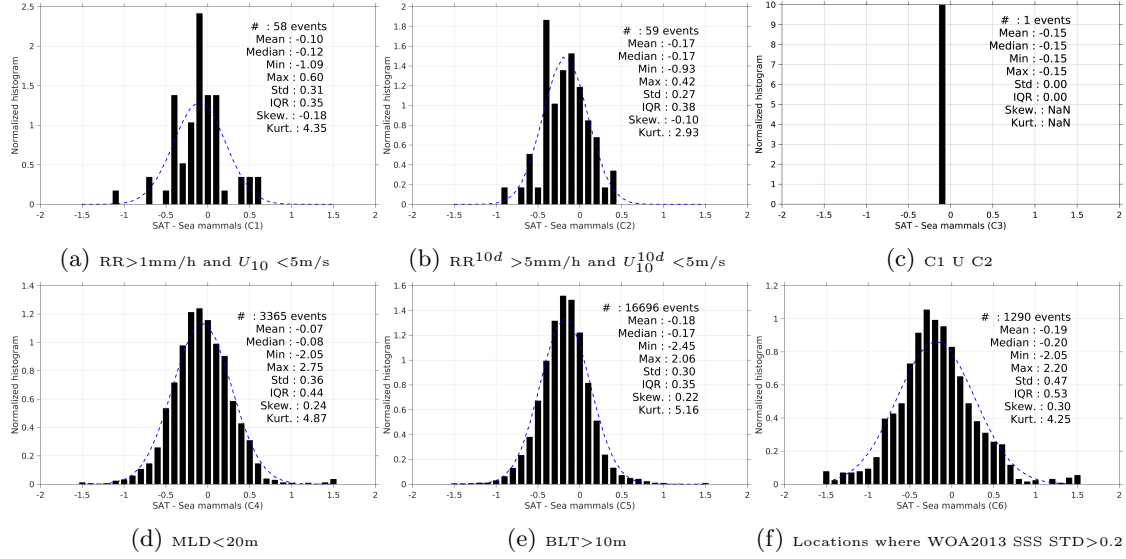
Figure 13: Normalized histogram of \Delta SSS (SMOS-L3-BEC-OA-V1-9DAYS-0.25DEG - Sea mammals) for 6 different subdatasets corresponding to: RR>1mm/h and U_{10} < 5\text{m/s} (a), RR^{10d} > 5\text{mm/h} and U_{10}^{10d} < 5\text{m/s} (b), C1 U C2 (c), MLD<20m (d), BLT>10m (e), Locations where WOA2013 SSS STD>0.2 (f).
