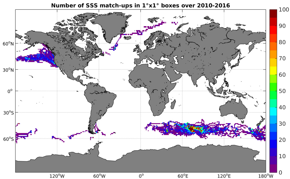
Figure 4: Number of SSS match-ups between Sea mammals SSS and the SMOS-L3-BEC-OA-V1-9DAYS-0.25DEG SSS product for the Global Ocean Pi-MEP region over 1^\circ \times 1^\circ boxes and for the full satellite product period.
