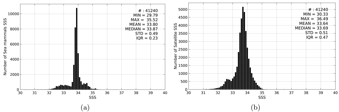
Figure 2: Histograms of SSS from Sea mammals (a) and SMOS-L3-BEC-OA-V1-9DAYS-0.25DEG (b) considering all match-up pairs per bins of 0.1 over the Global Ocean Pi-MEP region and for the full satellite product period.
