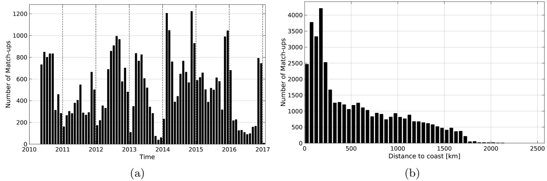
Figure 1: Number of match-ups between Sea mammals and SMOS-L3-BEC-OA-V1-9DAYS-0.25DEG SSS as a function of time (a) and as function of the distance to coast (b) over the Global Ocean Pi-MEP region and for the full satellite product period.
