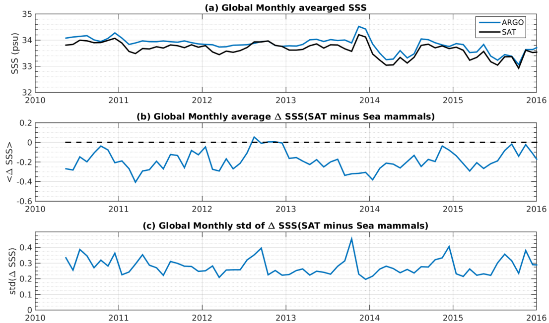
Figure 7: Time series of the monthly averaged mean SSS (top), mean \Delta SSS (Satellite - Sea mammals) and STD of \Delta SSS (Satellite - Sea mammals) over the Global Ocean Pi-MEP region considering all match-ups collected by the Pi-MEP platform.
