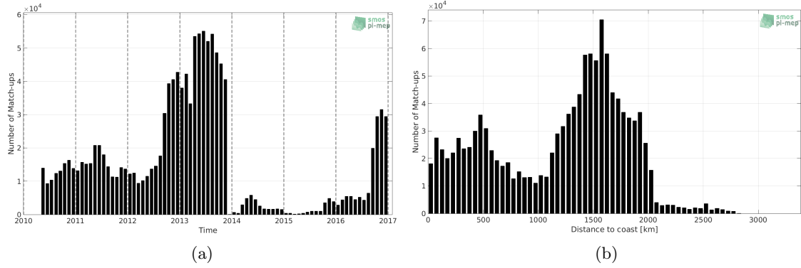
Figure 1: Number of match-ups between Surface drifters and SMOS-L3-BEC-OA-V1-9DAYS-0.25DEG SSS as a function of time (a) and as function of the distance to coast (b) over the Global Ocean Pi-MEP region and for the full satellite product period.
