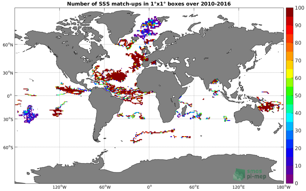
Figure 3: Number of SSS match-ups between Surface drifters SSS and the SMOS-L3-BEC-OA-V1-9DAYS-0.25DEG SSS product for the Global Ocean Pi-MEP region over 1°x1° boxes and for the full satellite product period.
