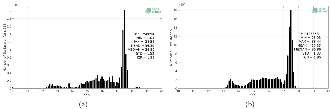
Figure 2: Histograms of SSS from Surface drifters (a) and SMOS-L3-BEC-OA-V1-9DAYS-0.25DEG (b) considering all match-up pairs per bins of 0.1 over the Global Ocean Pi-MEP region and for the full satellite product period.
