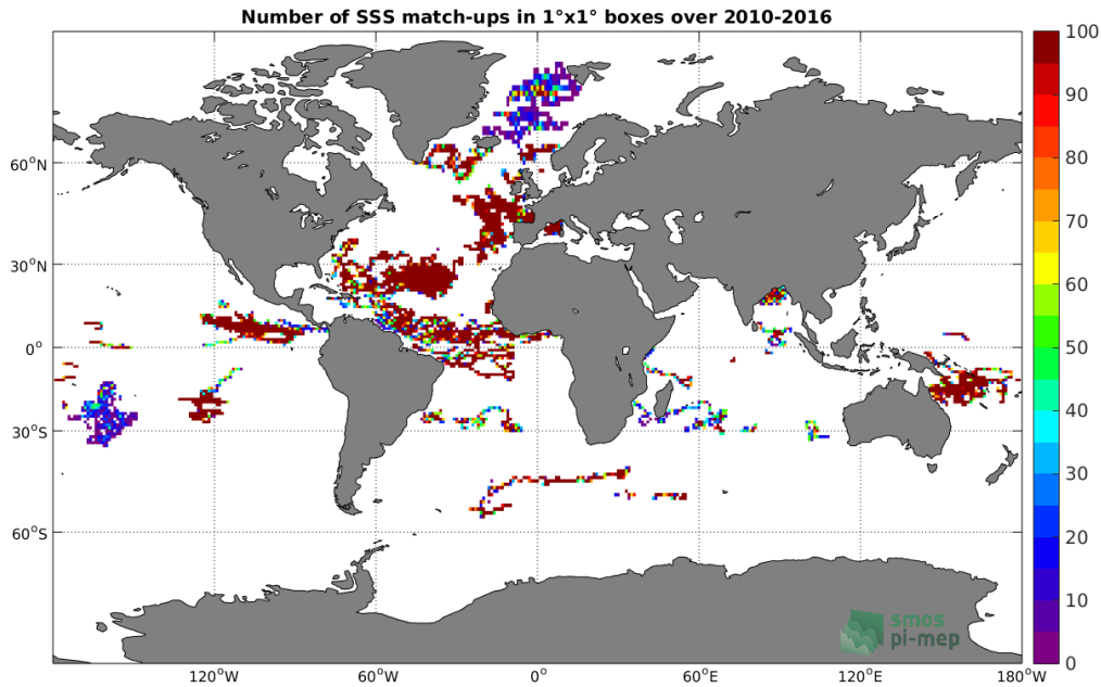
Figure 3: Number of SSS match-ups between Surface drifters SSS and the SMOS-L3-BEC-OA-V1-9DAYS-0.25DEG SSS product for the Global Ocean Pi-MEP region over 1^\circ \times 1^\circ boxes and for the full satellite product period.
