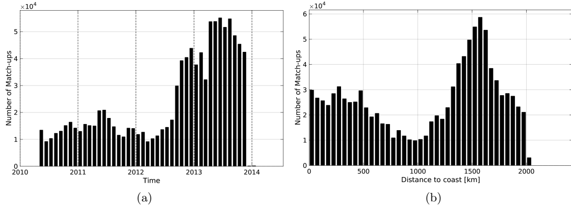
Figure 1: Number of match-ups between Surface drifters and SMOS-L3-BEC-OA-V1-9DAYS-0.25DEG SSS as a function of time (a) and as function of the distance to coast (b) over the Global Ocean Pi-MEP region and for the full satellite product period.
