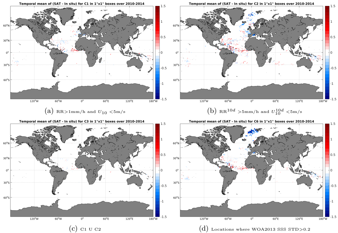
Figure 11: Temporal mean gridded over spatial boxes of size 1°x1° of \Delta SSS (SMOS-L3-BEC-OA-V1-9DAYS-0.25DEG - Surface drifters) for 4 different subdatasets corresponding to:RR>1mm/h and U_{10} < 5\text{m/s} (a), RR^{10d} > 5\text{mm/h} and U_{10}^{10d} < 5\text{m/s} (b), C1 U C2 (c),Locations where WOA2013 SSS STD>0.2 (d).
