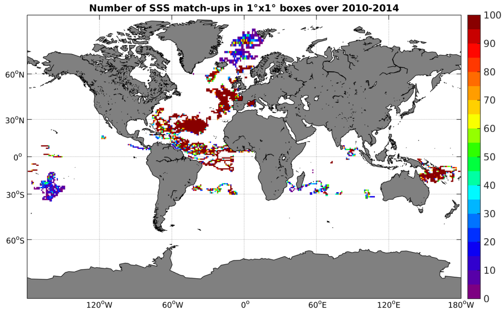
Figure 3: Number of SSS match-ups between Surface drifters SSS and the SMOS-L3-BEC-OA-V1-9DAYS-0.25DEG SSS product for the Global Ocean Pi-MEP region over 1°x1° boxes and for the full satellite product period.
