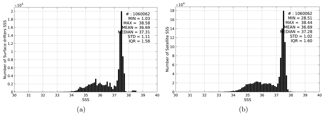
Figure 2: Histograms of SSS from Surface drifters (a) and SMOS-L3-BEC-OA-V1-9DAYS-0.25DEG (b) considering all match-up pairs per bins of 0.1 over the Global Ocean Pi-MEP region and for the full satellite product period.
