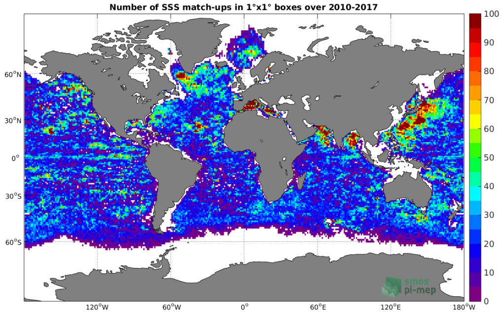
Figure 4: Number of SSS match-ups between Argo SSS and the SMOS-L3-BEC-OA-V1-9DAYS-0.25DEG SSS product for the Global Ocean Pi-MEP region over 1°x1° boxes and for the full satellite product period.
