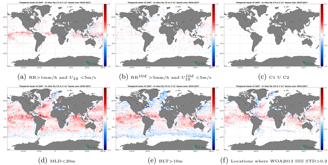
Figure 12: Temporal mean gridded over spatial boxes of size 1^\circ \times 1^\circ of \Delta\text{SSS} (SMOS-L3-BEC-OA-V1-9DAYS-0.25DEG - Argo) for 6 different subdatasets corresponding to: RR > 1\text{mm/h} and U_{10} < 5\text{m/s} (a), RR^{10d} > 5\text{mm/h} and U_{10}^{10d} < 5\text{m/s} (b), C1 U C2 (c), MLD < 20\text{m} (d), BLT > 10\text{m} (e), Locations where WOA2013 SSS STD > 0.2 (f).
