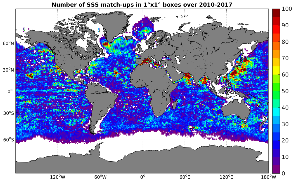
Figure 4: Number of SSS match-ups between Argo SSS and the SMOS-L3-BEC-OA-V1-9DAYS-0.25DEG SSS product for the Global Ocean Pi-MEP region over 1^\circ \times 1^\circ boxes and for the full satellite product period.
