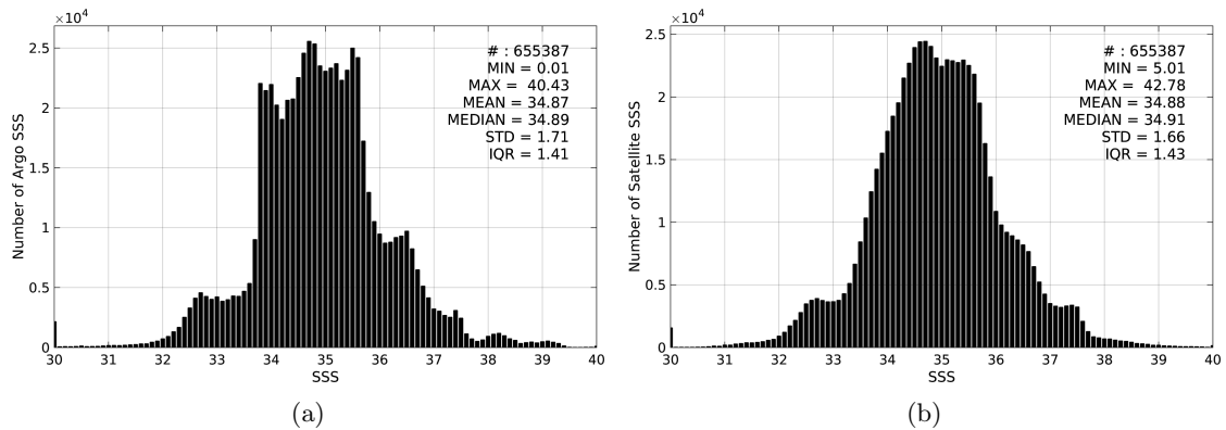
Figure 2: Histograms of SSS from Argo (a) and SMOS-L3-BEC-OA-V1-9DAYS-0.25DEG (b) considering all match-up pairs per bins of 0.1 over the Global Ocean Pi-MEP region and for the full satellite product period.
