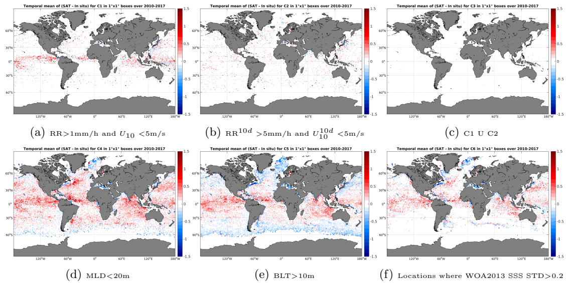
Figure 12: Temporal mean gridded over spatial boxes of size 1^\circ \times 1^\circ of \Delta SSS (SMOS-L3-BEC-OA-V1-9DAYS-0.25DEG - Argo) for 6 different subdatasets corresponding to:RR >1 mm/h and U_{10} < 5 m/s (a), RR ^{10d} > 5 mm/h and U_{10}^{10d} < 5 m/s (b), C1 U C2 (c),MLD <20 m (d),BLT >10 m (e),Locations where WOA2013 SSS STD >0.2 (f).
