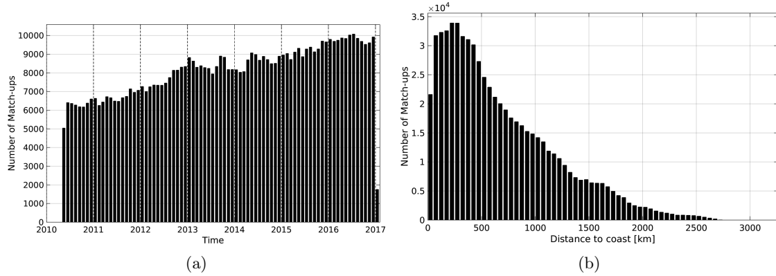
Figure 1: Number of match-ups between Argo and SMOS-L3-BEC-OA-V1-9DAYS-0.25DEG SSS as a function of time (a) and as function of the distance to coast (b) over the Global Ocean Pi-MEP region and for the full satellite product period.
