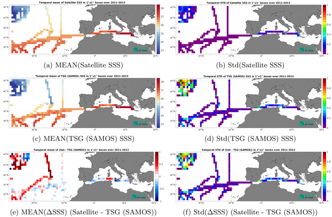
Figure 7: Temporal mean (left) and Std (right) of SSS from SMOS SSS L3 MED-ATL-OA v2 - 9 Days (BEC) (top), TSG (SAMOS) (middle), and of \Delta SSS (Satellite - TSG (SAMOS)). Only match-up pairs are used to generate these maps.
