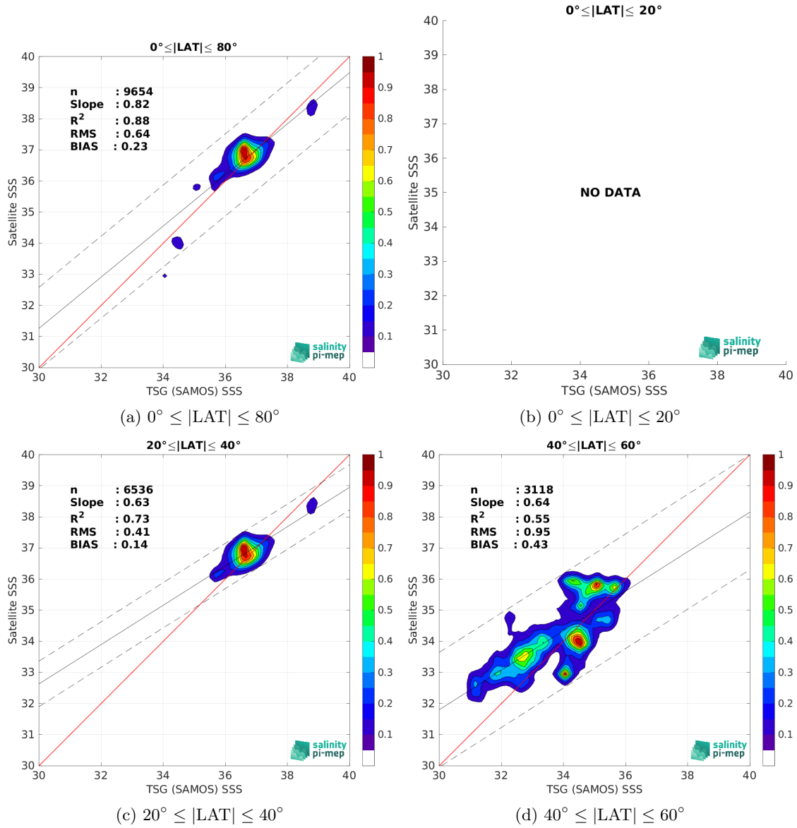
Figure 10: Contour maps of the concentration of SMOS SSS L3 MED-ATL-OA v2 - 9 Days (BEC) SSS (y-axis) versus TSG (SAMOS) SSS (x-axis) at match-up pairs for different latitude bands. For each plot, the red line shows x=y . The black thin and dashed lines indicate a linear fit through the data cloud and the \pm 95\% confidence levels, respectively. The number match-up pairs n , the slope and R^2 coefficient of the linear fit, the root mean square (RMS) and the mean bias between satellite and in situ data are indicated for each latitude band in each plots.
