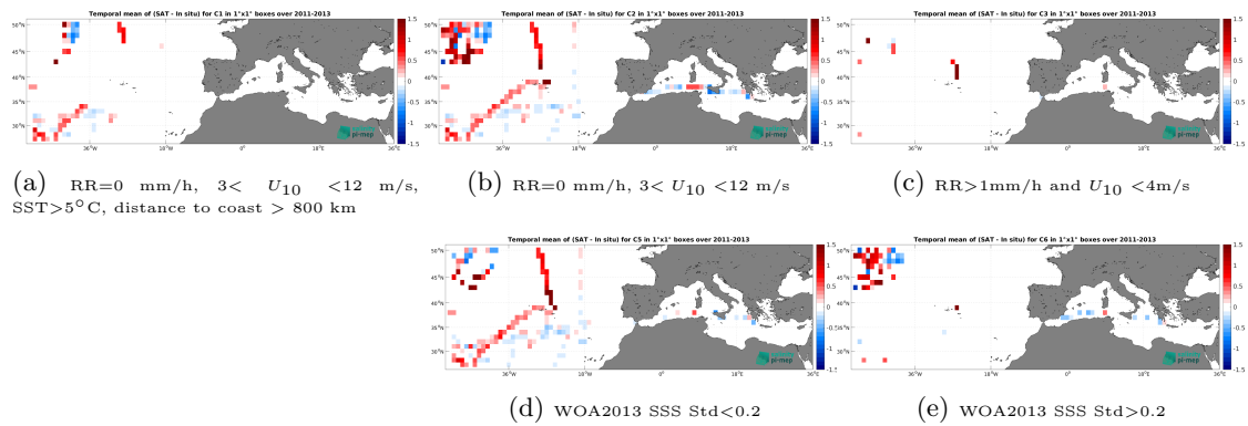
Figure 14: Temporal mean gridded over spatial boxes of size 1^\circ \times 1^\circ of \Delta\text{SSS} (SMOS SSS L3 MED-ATL-OA v2 - 9 Days (BEC) - TSG (SAMOS)) for 5 different subdatasets corresponding to:RR=0 mm/h, 3 < U_{10} < 12 m/s, SST >5^\circ\text{C} , distance to coast > 800 km (a), RR=0 mm/h, 3 < U_{10} < 12 m/s (b), RR >1 mm/h and U_{10} < 4 m/s (c), WOA2013 SSS Std <0.2 (d), WOA2013 SSS Std >0.2 (e).
