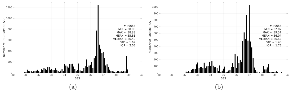
Figure 3: Histograms of SSS from TSG (SAMOS) (a) and SMOS SSS L3 MED-ATL-OA v2 - 9 Days (BEC) (b) considering all match-up pairs per bins of 0.1 over the Global Ocean Pi-MEP region and for the full satellite product period.
