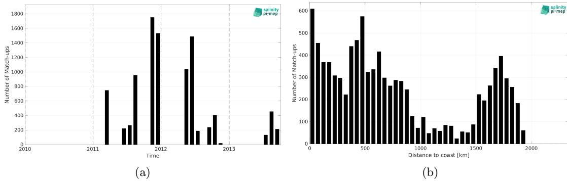
Figure 2: Number of match-ups between TSG (SAMOS) and SMOS SSS L3 MED-ATL-OA v2 - 9 Days (BEC) SSS as a function of time (a) and as function of the distance to coast (b) over the Global Ocean Pi-MEP region and for the full satellite product period.
